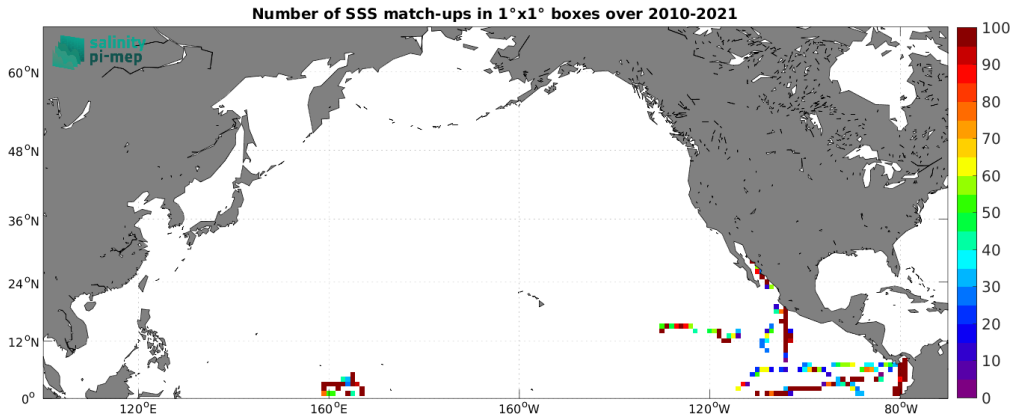
Figure 5: Number of SSS match-ups between TSG (GOSUD-Research-vessel) SSS and the SMOS SSS L2Q v331 - No FLAG (CMEMS-CATDS-CPDC) SSS product for the North Pacific Ocean Pi-MEP region over 1^\circ \times 1^\circ boxes and for the full satellite product period.
