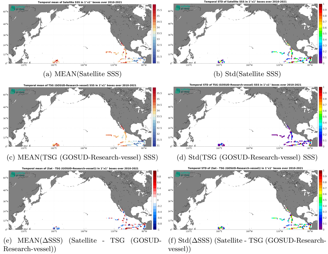
Figure 7: Temporal mean (left) and Std (right) of SSS from SMOS SSS L2Q v331 - No FLAG (CMEMS-CATDS-CPDC) (top), TSG (GOSUD-Research-vessel) (middle), and of \Delta SSS (Satellite - TSG (GOSUD-Research-vessel)). Only match-up pairs are used to generate these maps.
