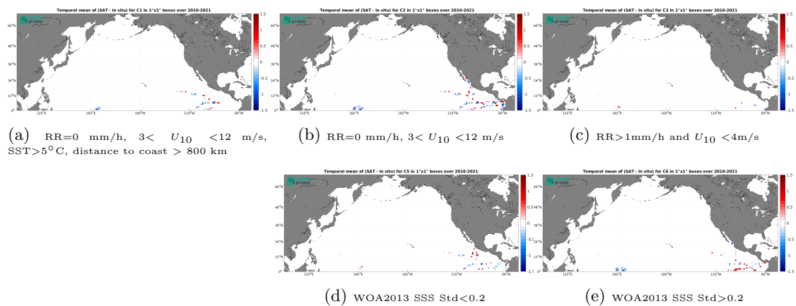
Figure 14: Temporal mean gridded over spatial boxes of size 1^\circ \times 1^\circ of \Delta SSS (SMOS SSS L2Q v331 - No FLAG (CMEMS-CATDS-CPDC) - TSG (GOSUD-Research-vessel)) for 5 different subdatasets corresponding to:RR=0 mm/h, 3 < U_{10} < 12 m/s, SST >5^\circ C, distance to coast > 800 km (a), RR=0 mm/h, 3 < U_{10} < 12 m/s (b), RR >1 mm/h and U_{10} < 4 m/s (c), WOA2013 SSS Std <0.2 (d), WOA2013 SSS Std >0.2 (e).
