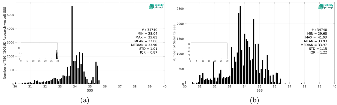
Figure 3: Histograms of SSS from TSG (GOSUD-Research-vessel) (a) and SMOS SSS L2Q v331 - No FLAG (CMEMS-CATDS-CPDC) (b) considering all match-up pairs per bins of 0.1 over the North Pacific Ocean Pi-MEP region and for the full satellite product period.
