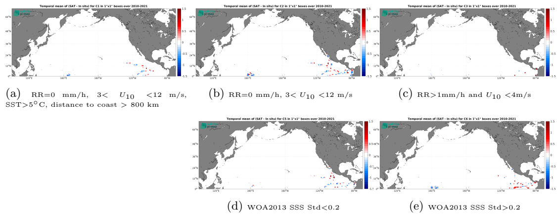
Figure 12: Temporal mean gridded over spatial boxes of size 1^\circ \times 1^\circ of \Delta\text{SSS} (SMOS SSS L2Q v331 - No FLAG (CMEMS-CATDS-CPDC) - TSG (GOSUD-Research-vessel)) for 5 different subdatasets corresponding to: RR=0 mm/h, 3 < U_{10} < 12 m/s, SST > 5°C, distance to coast > 800 km (a), RR=0 mm/h, 3 < U_{10} < 12 m/s (b), RR > 1mm/h and U_{10} < 4 m/s (c), WOA2013 SSS Std < 0.2 (d), WOA2013 SSS Std > 0.2 (e).
