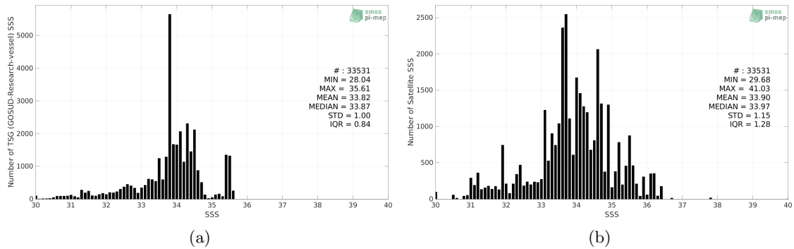
Figure 2: Histograms of SSS from TSG (GOSUD-Research-vessel) (a) and SMOS SSS L2Q v331 - No FLAG (CMEMS-CATDS-CPDC) (b) considering all match-up pairs per bins of 0.1 over the North Pacific Ocean Pi-MEP region and for the full satellite product period.
