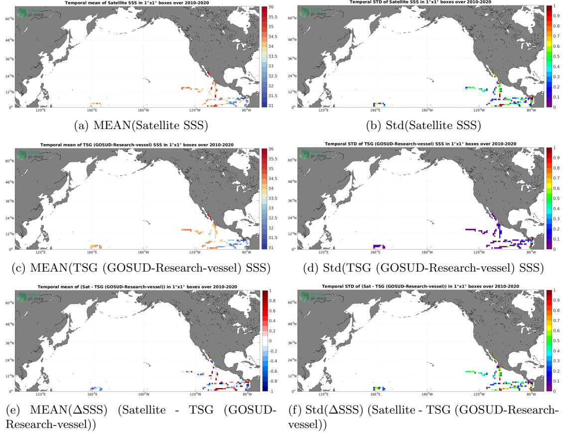
Figure 6: Temporal mean (left) and Std (right) of SSS from SMOS SSS L2Q v331 - No FLAG (CMEMS-CATDS-CPDC) (top), TSG (GOSUD-Research-vessel) (middle), and of \Delta SSS (Satellite - TSG (GOSUD-Research-vessel)). Only match-up pairs are used to generate these maps.
