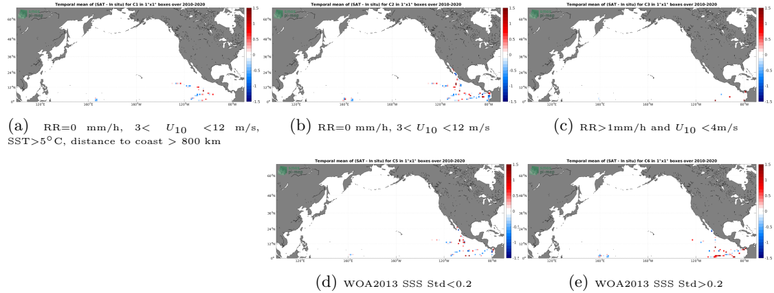
Figure 12: Temporal mean gridded over spatial boxes of size 1^{\circ}\times 1^{\circ} of \Delta SSS (SMOS SSS L2Q v331 - No FLAG (CMEMS-CATDS-CPDC) - TSG (GOSUD-Research-vessel)) for 5 different subdatasets corresponding to:RR=0 mm/h, 3 < U_{10} < 12 m/s, SST >5^{\circ}\text{C} , distance to coast > 800 km (a), RR=0 mm/h, 3 < U_{10} < 12 m/s (b), RR >1 mm/h and U_{10} < 4 m/s (c), WOA2013 SSS Std <0.2 (d), WOA2013 SSS Std >0.2 (e).
