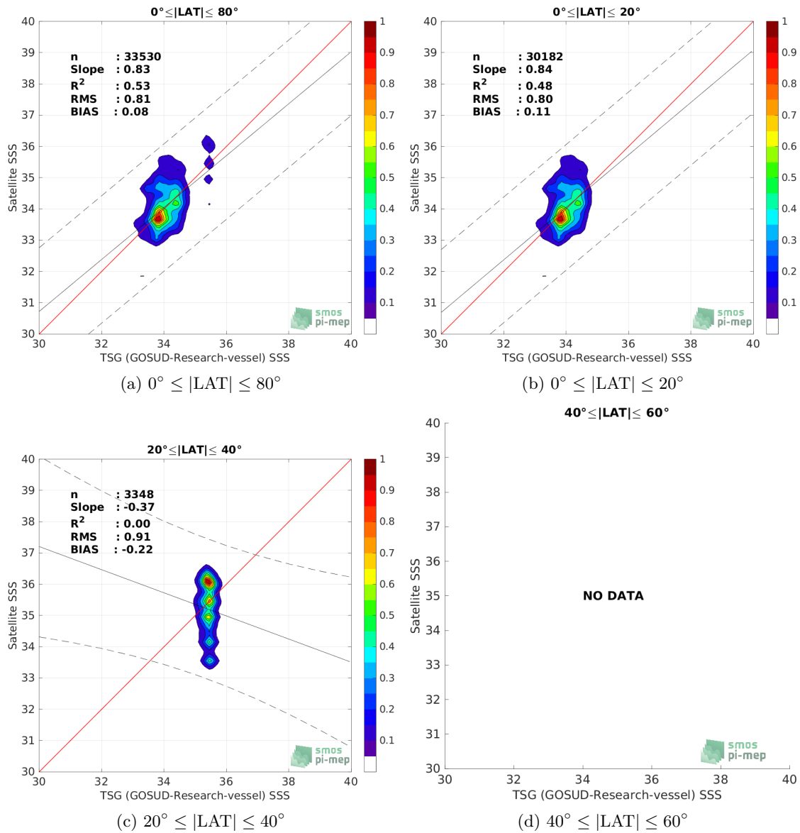
Figure 9: Contour maps of the concentration of SMOS SSS L2Q v331 - No FLAG (CMEMS-CATDS-CPDC) SSS (y-axis) versus TSG (GOSUD-Research-vessel) SSS (x-axis) at match-up pairs for different latitude bands. For each plot, the red line shows x=y . The black thin and dashed lines indicate a linear fit through the data cloud and the \pm 95\% confidence levels, respectively. The number match-up pairs n , the slope and R^2 coefficient of the linear fit, the root mean square (RMS) and the mean bias between satellite and in situ data are indicated for each latitude band in each plots.
