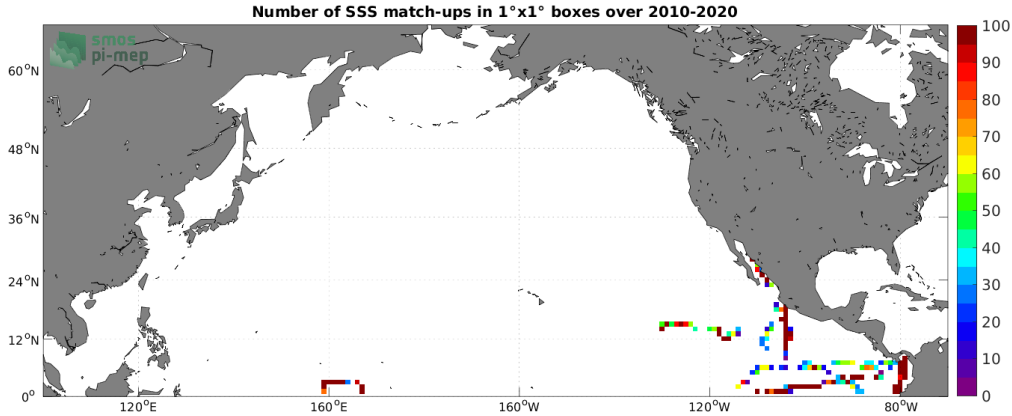
Figure 4: Number of SSS match-ups between TSG (GOSUD-Research-vessel) SSS and the SMOS SSS L2Q v331 - No FLAG (CMEMS-CATDS-CPDC) SSS product for the North Pacific Ocean Pi-MEP region over 1^\circ \times 1^\circ boxes and for the full satellite product period.
