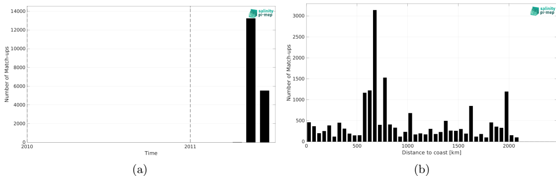
Figure 2: Number of match-ups between TSG (CSIC-UTM) and SMOS SSS L2Q v331 - No FLAG (CMEMS-CATDS-CPDC) SSS as a function of time (a) and as function of the distance to coast (b) over the North Pacific Ocean Pi-MEP region and for the full satellite product period.
