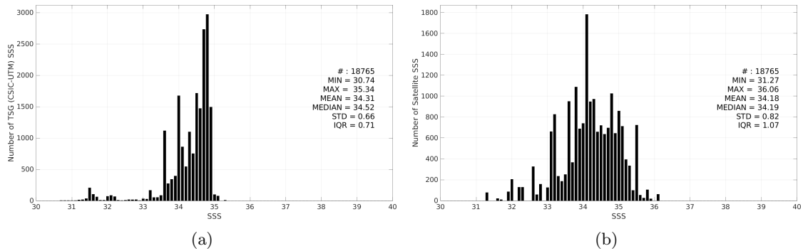
Figure 3: Histograms of SSS from TSG (CSIC-UTM) (a) and SMOS SSS L2Q v331 - No FLAG (CMEMS-CATDS-CPDC) (b) considering all match-up pairs per bins of 0.1 over the North Pacific Ocean Pi-MEP region and for the full satellite product period.
