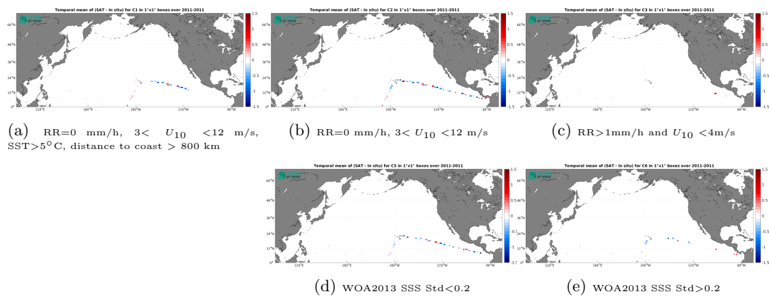
Figure 14: Temporal mean gridded over spatial boxes of size 1^\circ \times 1^\circ of \Delta\text{SSS} (SMOS SSS L2Q v331 - No FLAG (CMEMS-CATDS-CPDC) - TSG (CSIC-UTM)) for 5 different subdatasets corresponding to: RR=0 mm/h, 3 < U_{10} < 12 m/s, SST > 5°C, distance to coast > 800 km (a), RR=0 mm/h, 3 < U_{10} < 12 m/s (b), RR > 1mm/h and U_{10} < 4 m/s (c), WOA2013 SSS Std < 0.2 (d), WOA2013 SSS Std > 0.2 (e).
