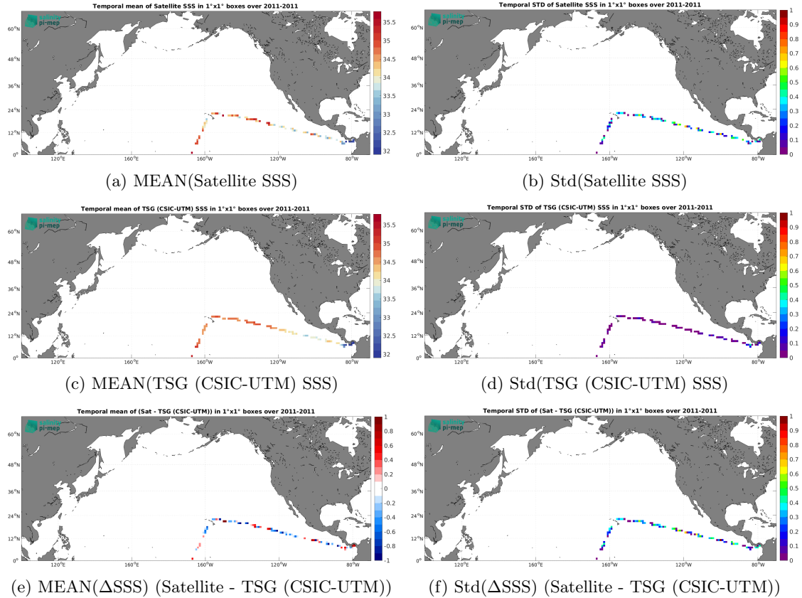
Figure 7: Temporal mean (left) and Std (right) of SSS from SMOS SSS L2Q v331 - No FLAG (CMEMS-CATDS-CPDC) (top), TSG (CSIC-UTM) (middle), and of \Delta\text{SSS} (Satellite - TSG (CSIC-UTM)). Only match-up pairs are used to generate these maps.
