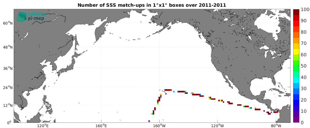
Figure 5: Number of SSS match-ups between TSG (CSIC-UTM) SSS and the SMOS SSS L2Q v331 - No FLAG (CMEMS-CATDS-CPDC) SSS product for the North Pacific Ocean Pi-MEP region over 1^\circ \times 1^\circ boxes and for the full satellite product period.
