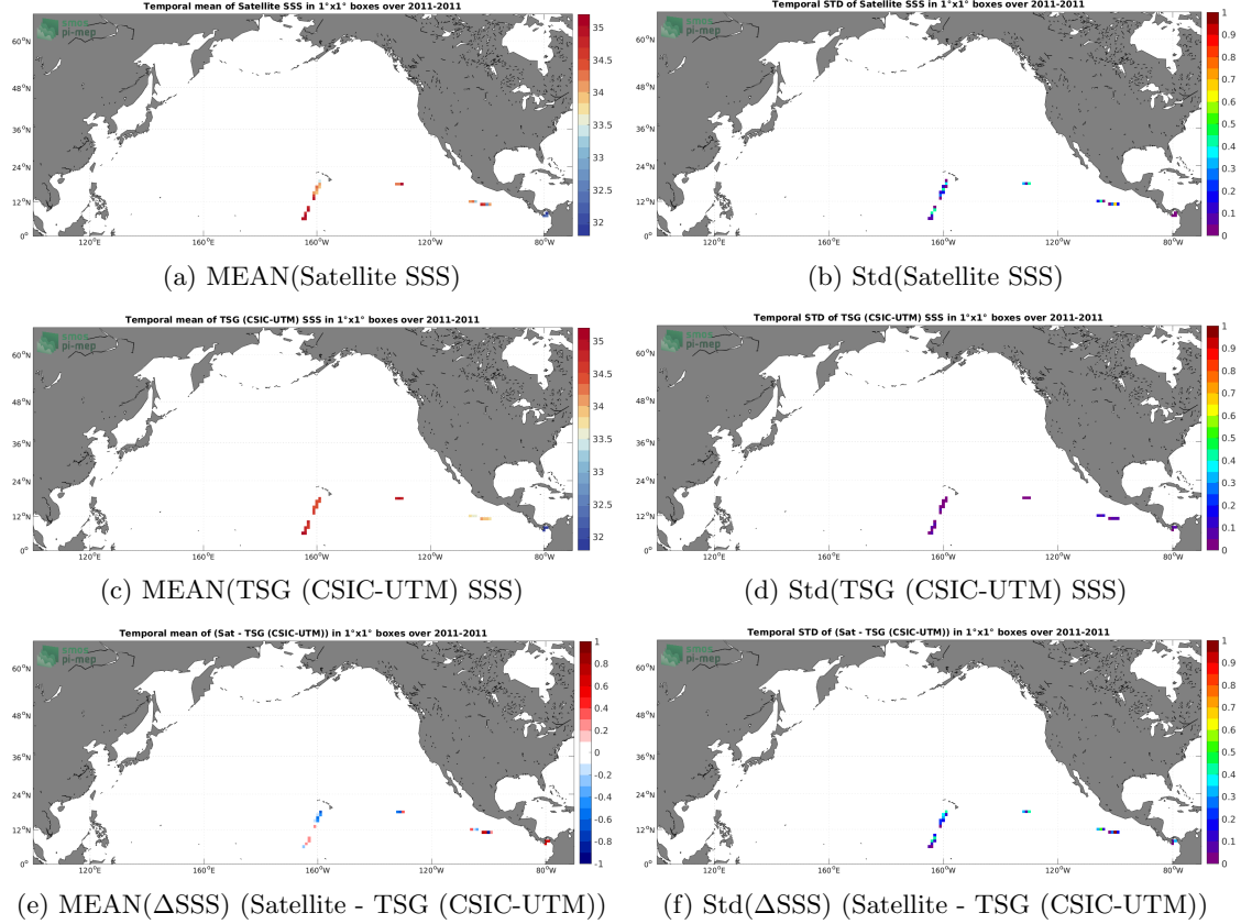
Figure 6: Temporal mean (left) and Std (right) of SSS from SMOS SSS L2Q v331 - No FLAG (CMEMS-CATDS-CPDC) (top), TSG (CSIC-UTM) (middle), and of \Delta\text{SSS} (Satellite - TSG (CSIC-UTM)). Only match-up pairs are used to generate these maps.
