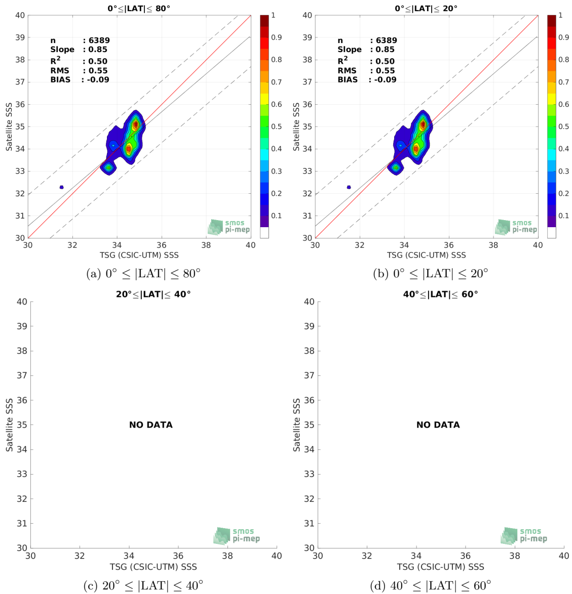
Figure 9: Contour maps of the concentration of SMOS SSS L2Q v331 - No FLAG (CMEMS-CATDS-CPDC) SSS (y-axis) versus TSG (CSIC-UTM) SSS (x-axis) at match-up pairs for different latitude bands. For each plot, the red line shows x=y . The black thin and dashed lines indicate a linear fit through the data cloud and the \pm 95\% confidence levels, respectively. The number match-up pairs n , the slope and R^2 coefficient of the linear fit, the root mean square (RMS) and the mean bias between satellite and in situ data are indicated for each latitude band in each plots.
