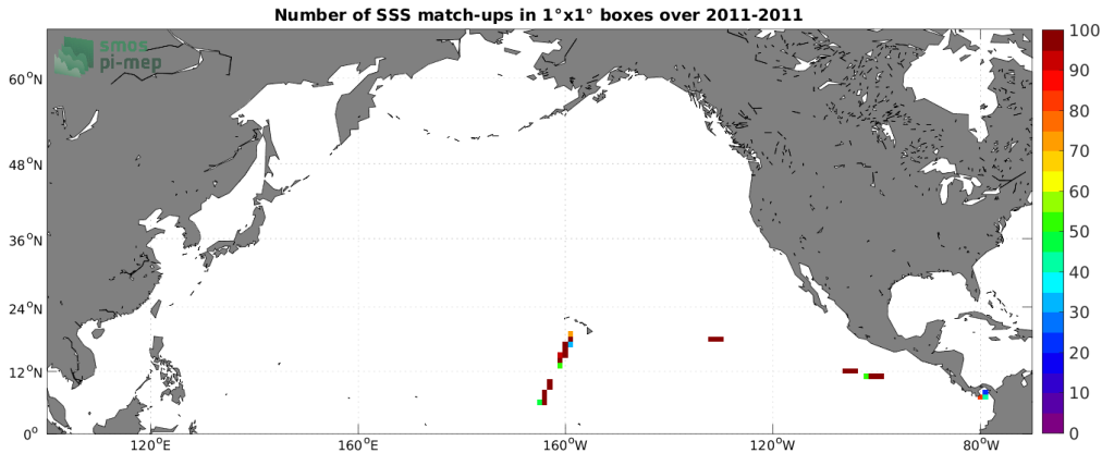
Figure 4: Number of SSS match-ups between TSG (CSIC-UTM) SSS and the SMOS SSS L2Q v331 - No FLAG (CMEMS-CATDS-CPDC) SSS product for the North Pacific Ocean Pi-MEP region over 1^\circ \times 1^\circ boxes and for the full satellite product period.
