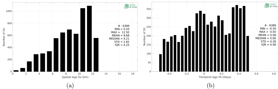
Figure 5: Histograms of the spatial (a) and temporal (b) lags between the location/time of the TSG (CSIC-UTM) measurement and the date of the corresponding SMOS SSS L2Q v331 - No FLAG (CMEMS-CATDS-CPDC) SSS pixel.
