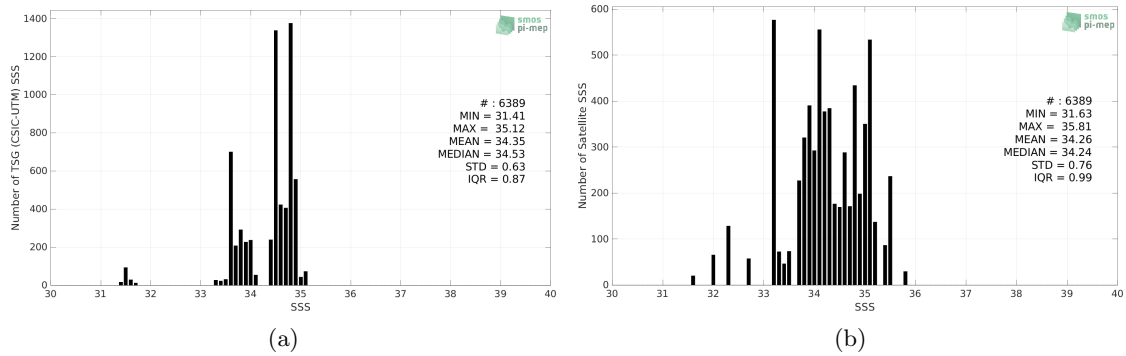
Figure 2: Histograms of SSS from TSG (CSIC-UTM) (a) and SMOS SSS L2Q v331 - No FLAG (CMEMS-CATDS-CPDC) (b) considering all match-up pairs per bins of 0.1 over the North Pacific Ocean Pi-MEP region and for the full satellite product period.
