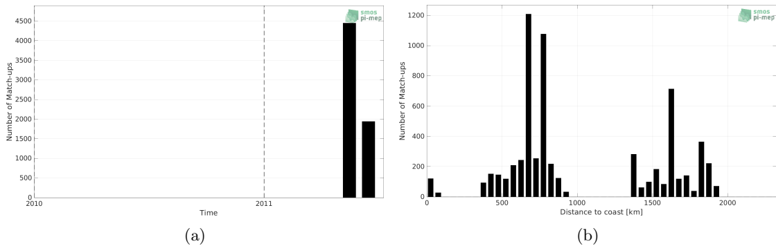
Figure 1: Number of match-ups between TSG (CSIC-UTM) and SMOS SSS L2Q v331 - No FLAG (CMEMS-CATDS-CPDC) SSS as a function of time (a) and as function of the distance to coast (b) over the North Pacific Ocean Pi-MEP region and for the full satellite product period.
