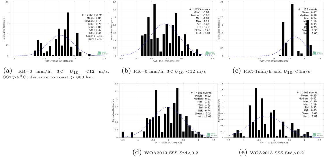
Figure 13: Normalized histogram of \Delta SSS (SMOS SSS L2Q v331 - No FLAG (CMEMS-CATDS-CPDC) - TSG (CSIC-UTM)) for 5 different subdatasets corresponding to: RR=0 mm/h, 3 < U_{10} < 12 m/s, SST > 5°C, distance to coast > 800 km (a), RR=0 mm/h, 3 < U_{10} < 12 m/s (b), RR > 1mm/h and U_{10} < 4 m/s (c), WOA2013 SSS Std < 0.2 (d), WOA2013 SSS Std > 0.2 (e).
