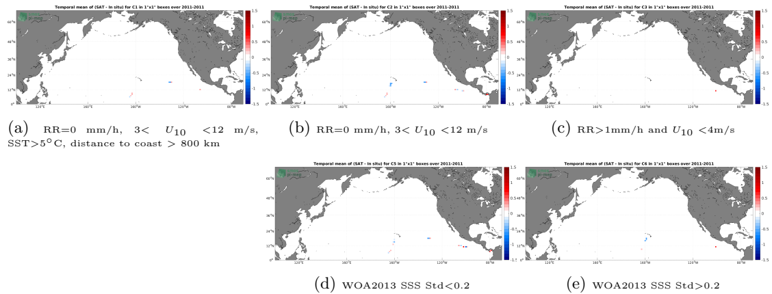
Figure 12: Temporal mean gridded over spatial boxes of size 1^{\circ}\times 1^{\circ} of \Delta\text{SSS} (SMOS SSS L2Q v331 - No FLAG (CMEMS-CATDS-CPDC) - TSG (CSIC-UTM)) for 5 different subdatasets corresponding to:RR=0 mm/h, 3 < U_{10} < 12 m/s, SST >5^{\circ}\text{C} , distance to coast > 800 km (a), RR=0 mm/h, 3 < U_{10} < 12 m/s (b), RR >1 mm/h and U_{10} < 4 m/s (c), WOA2013 SSS Std <0.2 (d), WOA2013 SSS Std >0.2 (e).
