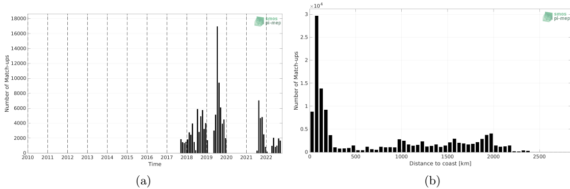
Figure 1: Number of match-ups between Saildrone and SMOS SSS L2Q v331 - No FLAG (CMEMS-CATDS-CPDC) SSS as a function of time (a) and as function of the distance to coast (b) over the North Pacific Ocean Pi-MEP region and for the full satellite product period.
