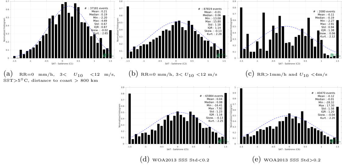
Figure 13: Normalized histogram of \Delta SSS (SMOS SSS L2Q v331 - No FLAG (CMEMS-CATDS-CPDC) - Sairdrone) for 5 different subdatasets corresponding to: RR=0 mm/h, 3 < U_{10} < 12 m/s, SST>5°C, distance to coast > 800 km (a), RR=0 mm/h, 3 < U_{10} < 12 m/s (b), RR>1mm/h and U_{10} < 4 m/s (c), WOA2013 SSS Std<0.2 (d), WOA2013 SSS Std>0.2 (e).
