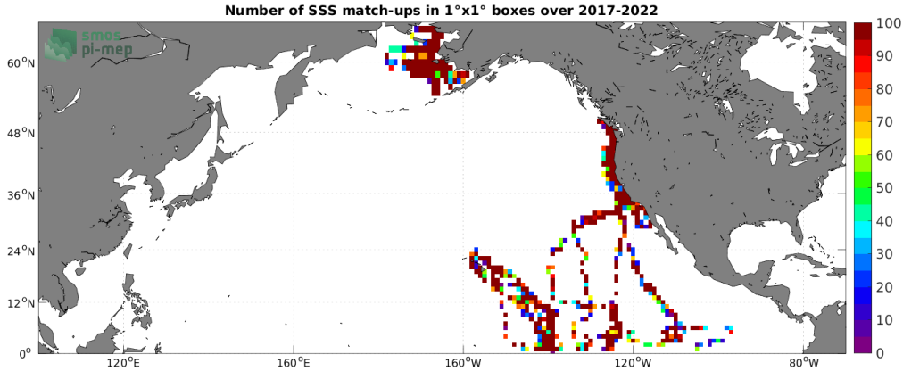
Figure 4: Number of SSS match-ups between Saildrone SSS and the SMOS SSS L2Q v331 - No FLAG (CMEMS-CATDS-CPDC) SSS product for the North Pacific Ocean Pi-MEP region over 1^\circ \times 1^\circ boxes and for the full satellite product period.
