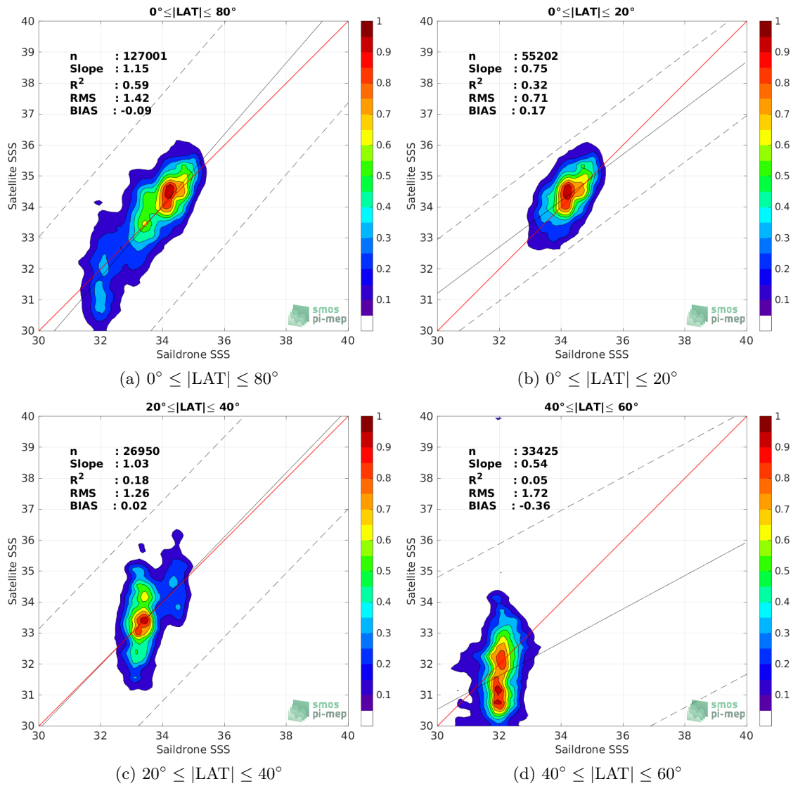
Figure 9: Contour maps of the concentration of SMOS SSS L2Q v331 - No FLAG (CMEMS-CATDS-CPDC) SSS (y-axis) versus Saildrone SSS (x-axis) at match-up pairs for different latitude bands. For each plot, the red line shows x=y . The black thin and dashed lines indicate a linear fit through the data cloud and the \pm 95\% confidence levels, respectively. The number match-up pairs n , the slope and R^2 coefficient of the linear fit, the root mean square (RMS) and the mean bias between satellite and in situ data are indicated for each latitude band in each plots.
