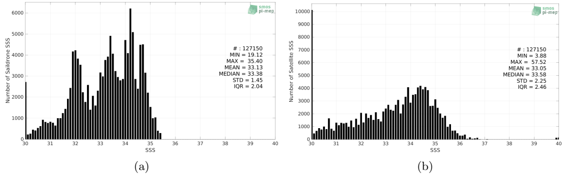
Figure 2: Histograms of SSS from Saildrone (a) and SMOS SSS L2Q v331 - No FLAG (CMEMS-CATDS-CPDC) (b) considering all match-up pairs per bins of 0.1 over the North Pacific Ocean Pi-MEP region and for the full satellite product period.
