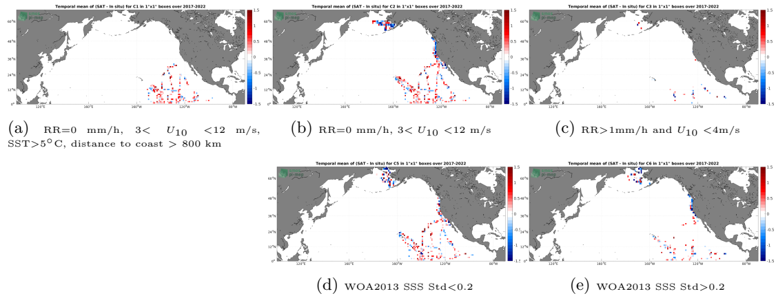
Figure 12: Temporal mean gridded over spatial boxes of size 1^\circ \times 1^\circ of \Delta SSS (SMOS SSS L2Q v331 - No FLAG (CMEMS-CATDS-CPDC) - Saildrone) for 5 different subdatasets corresponding to:RR=0 mm/h, 3 < U_{10} < 12 m/s, SST >5^\circ C, distance to coast > 800 km (a), RR=0 mm/h, 3 < U_{10} < 12 m/s (b), RR >1 mm/h and U_{10} < 4 m/s (c), WOA2013 SSS Std <0.2 (d), WOA2013 SSS Std >0.2 (e).
