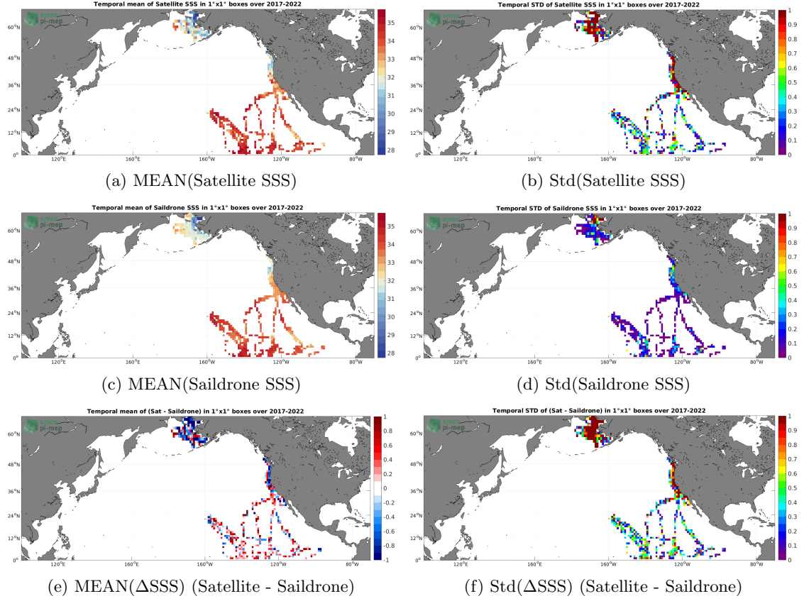
Figure 6: Temporal mean (left) and Std (right) of SSS from SMOS SSS L2Q v331 - No FLAG (CMEMS-CATDS-CPDC) (top), Saildrone (middle), and of \Delta SSS (Satellite - Saildrone). Only match-up pairs are used to generate these maps.
