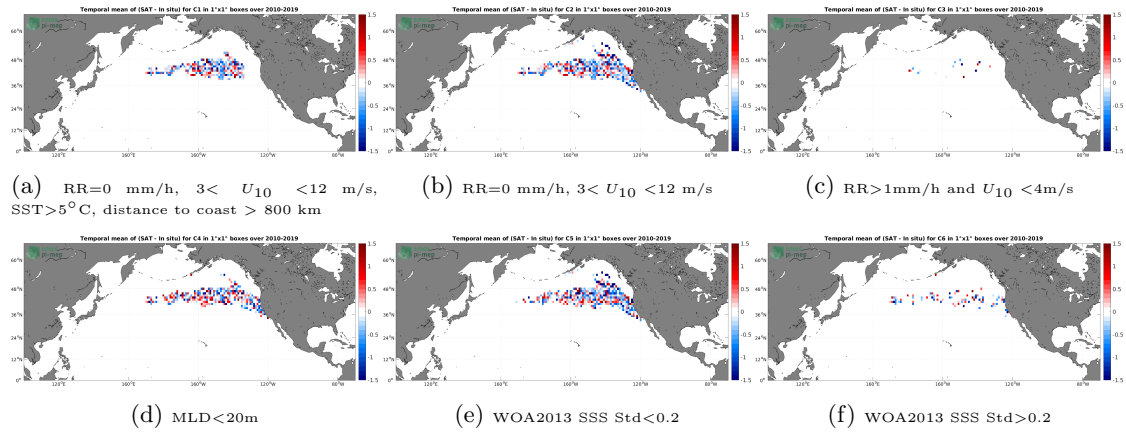
Figure 12: Temporal mean gridded over spatial boxes of size 1^{\circ}\times 1^{\circ} of \Delta\text{SSS} (SMOS SSS L2Q v331 - No FLAG (CMEMS-CATDS-CPDC) - Marine mammals) for 6 different subdatasets corresponding to: RR=0 mm/h, 3 < U_{10} < 12 m/s, SST > 5^{\circ}\text{C} , distance to coast > 800 km (a), RR=0 mm/h, 3 < U_{10} < 12 m/s (b), RR > 1\text{mm/h} and U_{10} < 4\text{m/s} (c), MLD < 20\text{m} (d), WOA2013 SSS Std < 0.2 (e), WOA2013 SSS Std > 0.2 (f).
