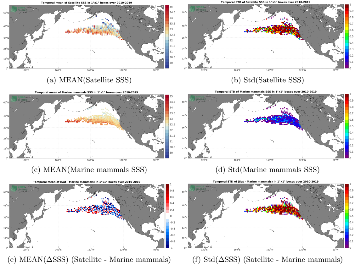
Figure 6: Temporal mean (left) and Std (right) of SSS from SMOS SSS L2Q v331 - No FLAG (CMEMS-CATDS-CPDC) (top), Marine mammals (middle), and of \Delta SSS (Satellite - Marine mammals). Only match-up pairs are used to generate these maps.
