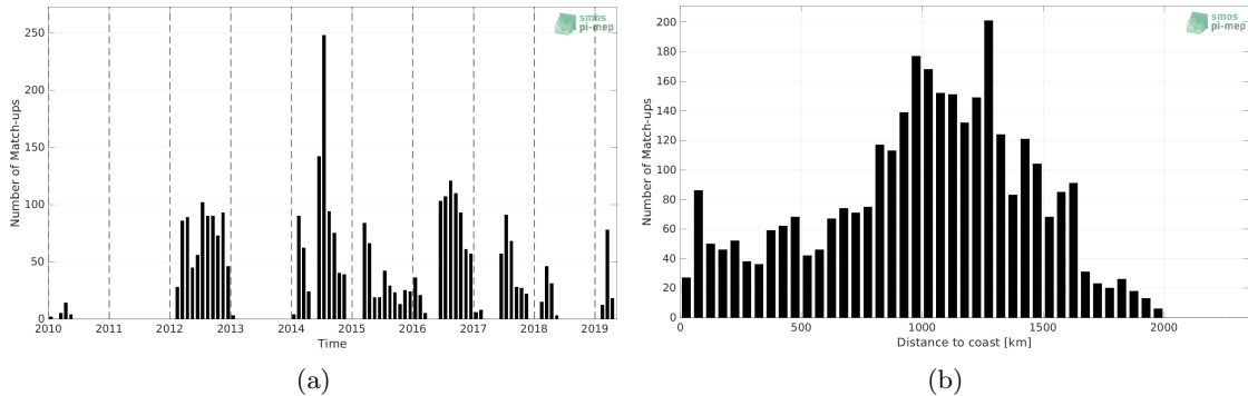
Figure 1: Number of match-ups between Marine mammals and SMOS SSS L2Q v331 - No FLAG (CMEMS-CATDS-CPDC) SSS as a function of time (a) and as function of the distance to coast (b) over the North Pacific Ocean Pi-MEP region and for the full satellite product period.
