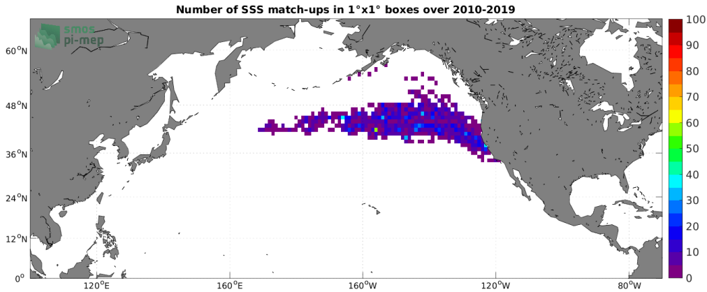
Figure 4: Number of SSS match-ups between Marine mammals SSS and the SMOS SSS L2Q v331 - No FLAG (CMEMS-CATDS-CPDC) SSS product for the North Pacific Ocean Pi-MEP region over 1^\circ \times 1^\circ boxes and for the full satellite product period.
