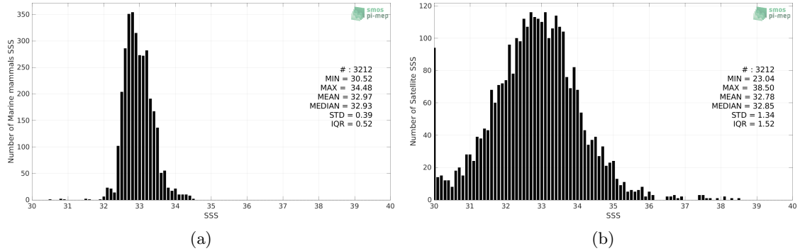
Figure 2: Histograms of SSS from Marine mammals (a) and SMOS SSS L2Q v331 - No FLAG (CMEMS-CATDS-CPDC) (b) considering all match-up pairs per bins of 0.1 over the North Pacific Ocean Pi-MEP region and for the full satellite product period.
