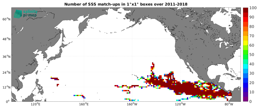
Figure 4: Number of SSS match-ups between Surface drifters SSS and the SMOS SSS L2Q v331 - No FLAG (CMEMS-CATDS-CPDC) SSS product for the North Pacific Ocean Pi-MEP region over 1^\circ \times 1^\circ boxes and for the full satellite product period.
