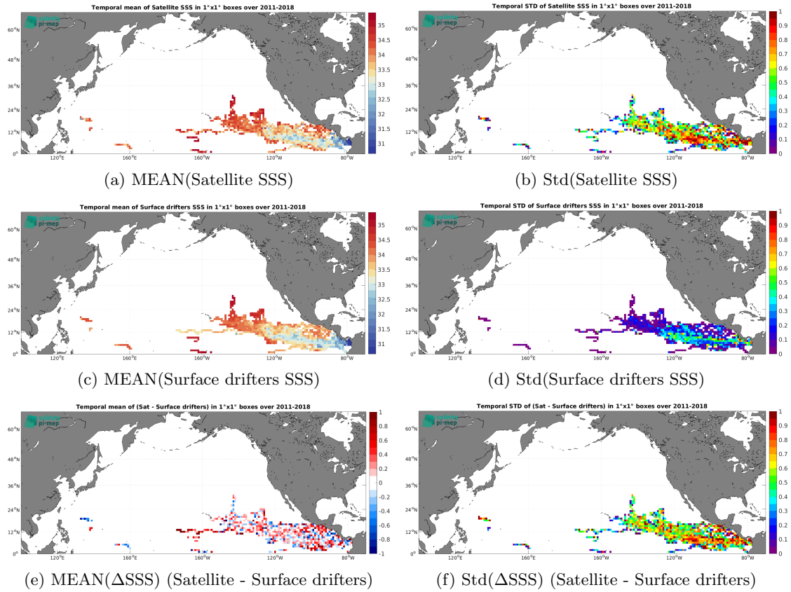
Figure 6: Temporal mean (left) and Std (right) of SSS from SMOS SSS L2Q v331 - No FLAG (CMEMS-CATDS-CPDC) (top), Surface drifters (middle), and of \Delta SSS (Satellite - Surface drifters). Only match-up pairs are used to generate these maps.
