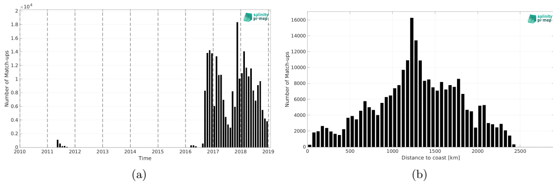
Figure 2: Number of match-ups between Surface drifters and SMOS SSS L2Q v331 - No FLAG (CMEMS-CATDS-CPDC) SSS as a function of time (a) and as function of the distance to coast (b) over the North Pacific Ocean Pi-MEP region and for the full satellite product period.
