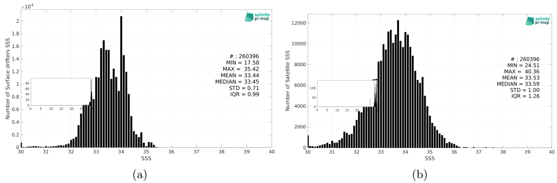
Figure 3: Histograms of SSS from Surface drifters (a) and SMOS SSS L2Q v331 - No FLAG (CMEMS-CATDS-CPDC) (b) considering all match-up pairs per bins of 0.1 over the North Pacific Ocean Pi-MEP region and for the full satellite product period.
