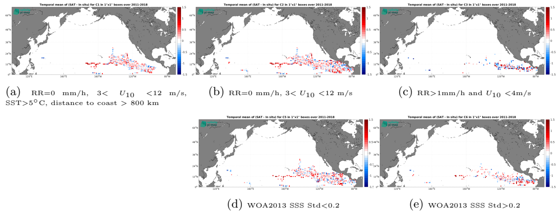
Figure 13: Temporal mean gridded over spatial boxes of size 1^\circ \times 1^\circ of \Delta\text{SSS} (SMOS SSS L2Q v331 - No FLAG (CMEMS-CATDS-CPDC) - Surface drifters) for 5 different subdatasets corresponding to:RR=0 mm/h, 3 < U_{10} < 12 m/s, SST >5^\circ\text{C} , distance to coast > 800 km (a), RR=0 mm/h, 3 < U_{10} < 12 m/s (b), RR >1 mm/h and U_{10} < 4 m/s (c), WOA2013 SSS Std <0.2 (d), WOA2013 SSS Std >0.2 (e).
