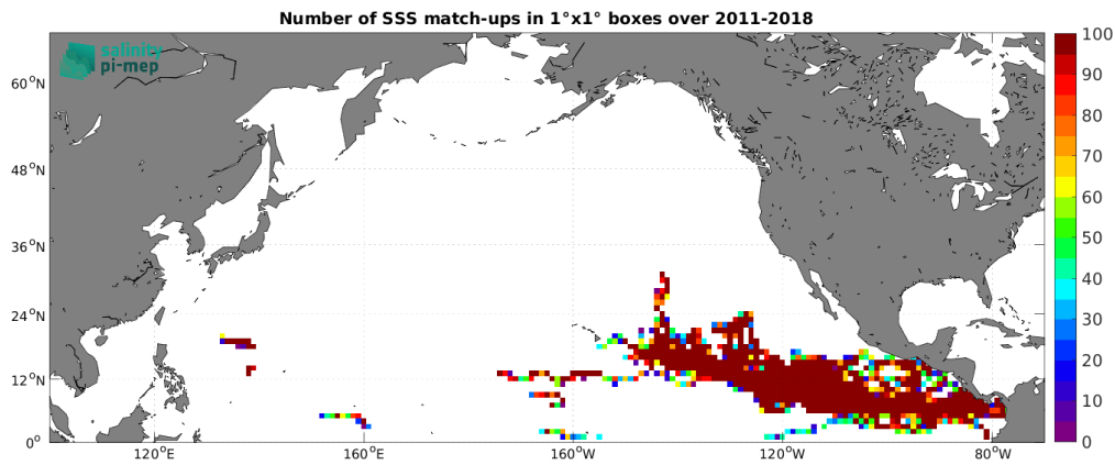
Figure 3: Number of SSS match-ups between Surface drifters SSS and the SMOS SSS L2Q v331 - No FLAG (CMEMS-CATDS-CPDC) SSS product for the North Pacific Ocean Pi-MEP region over 1^\circ \times 1^\circ boxes and for the full satellite product period.
