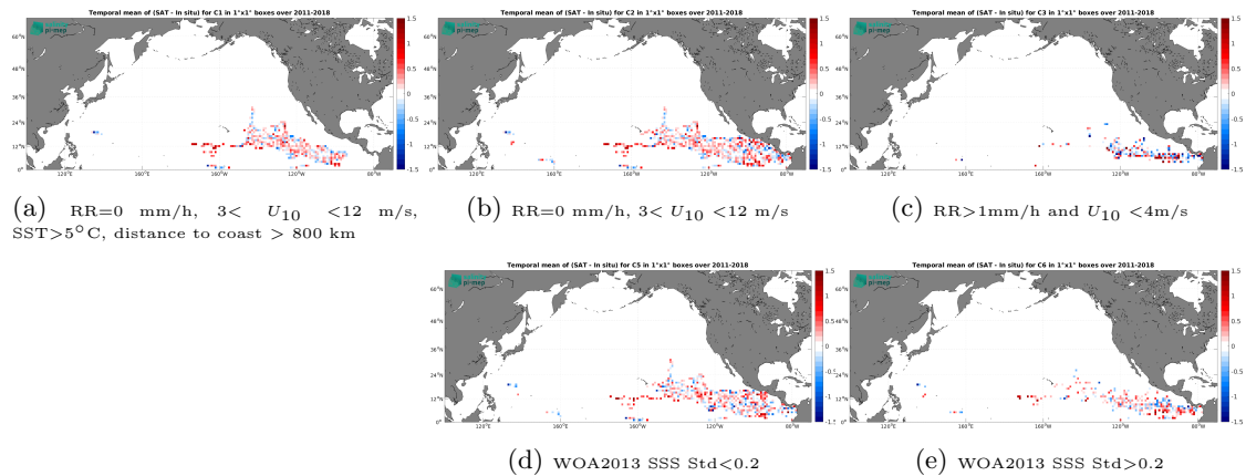
Figure 11: Temporal mean gridded over spatial boxes of size 1^\circ \times 1^\circ of \Delta\text{SSS} (SMOS SSS L2Q v331 - No FLAG (CMEMS-CATDS-CPDC) - Surface drifters) for 5 different subdatasets corresponding to:RR=0 mm/h, 3 < U_{10} < 12 m/s, SST >5^\circ\text{C} , distance to coast > 800 km (a), RR=0 mm/h, 3 < U_{10} < 12 m/s (b), RR >1 mm/h and U_{10} < 4 m/s (c), WOA2013 SSS Std <0.2 (d), WOA2013 SSS Std >0.2 (e).
