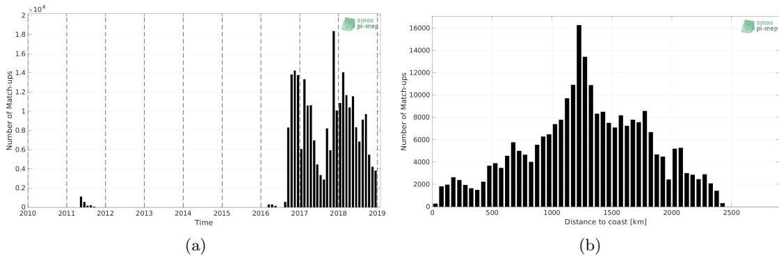
Figure 1: Number of match-ups between Surface drifters and SMOS SSS L2Q v331 - No FLAG (CMEMS-CATDS-CPDC) SSS as a function of time (a) and as function of the distance to coast (b) over the North Pacific Ocean Pi-MEP region and for the full satellite product period.
