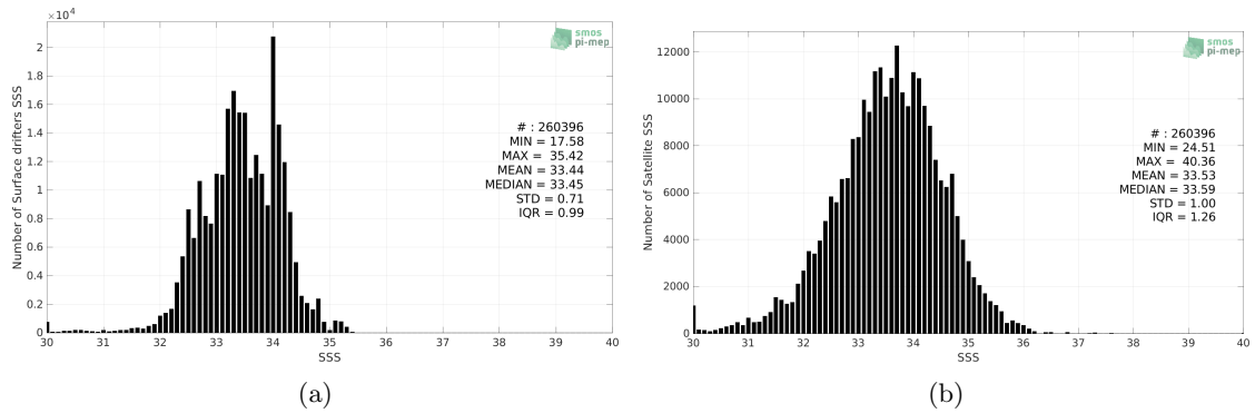
Figure 2: Histograms of SSS from Surface drifters (a) and SMOS SSS L2Q v331 - No FLAG (CMEMS-CATDS-CPDC) (b) considering all match-up pairs per bins of 0.1 over the North Pacific Ocean Pi-MEP region and for the full satellite product period.
