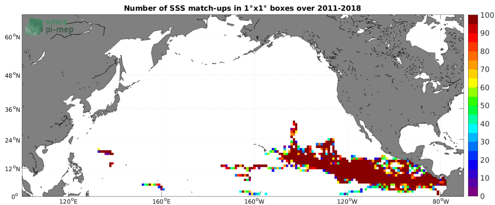
Figure 3: Number of SSS match-ups between Surface drifters SSS and the SMOS SSS L2Q v331 - No FLAG (CMEMS-CATDS-CPDC) SSS product for the North Pacific Ocean Pi-MEP region over 1^\circ \times 1^\circ boxes and for the full satellite product period.
