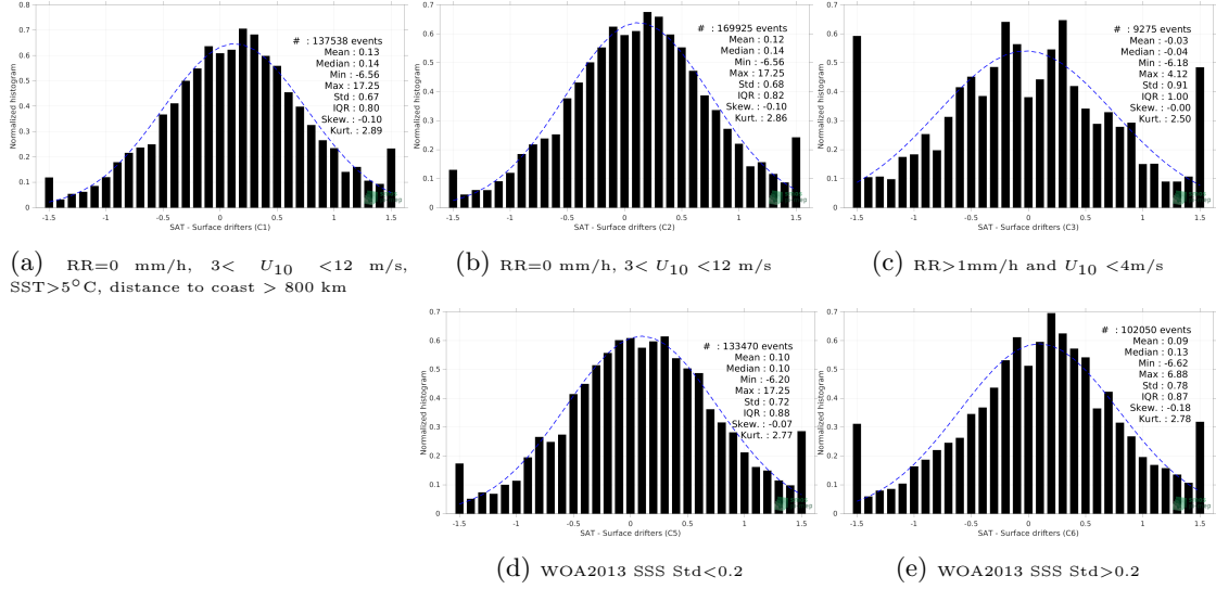
Figure 12: Normalized histogram of \Delta SSS (SMOS SSS L2Q v331 - No FLAG (CMEMS-CATDS-CPDC) - Surface drifters) for 5 different subdatasets corresponding to: RR=0 mm/h, 3 < U_{10} < 12 m/s, SST>5°C, distance to coast > 800 km (a), RR=0 mm/h, 3 < U_{10} < 12 m/s (b), RR>1mm/h and U_{10} < 4 m/s (c), WOA2013 SSS Std<0.2 (d), WOA2013 SSS Std>0.2 (e).
