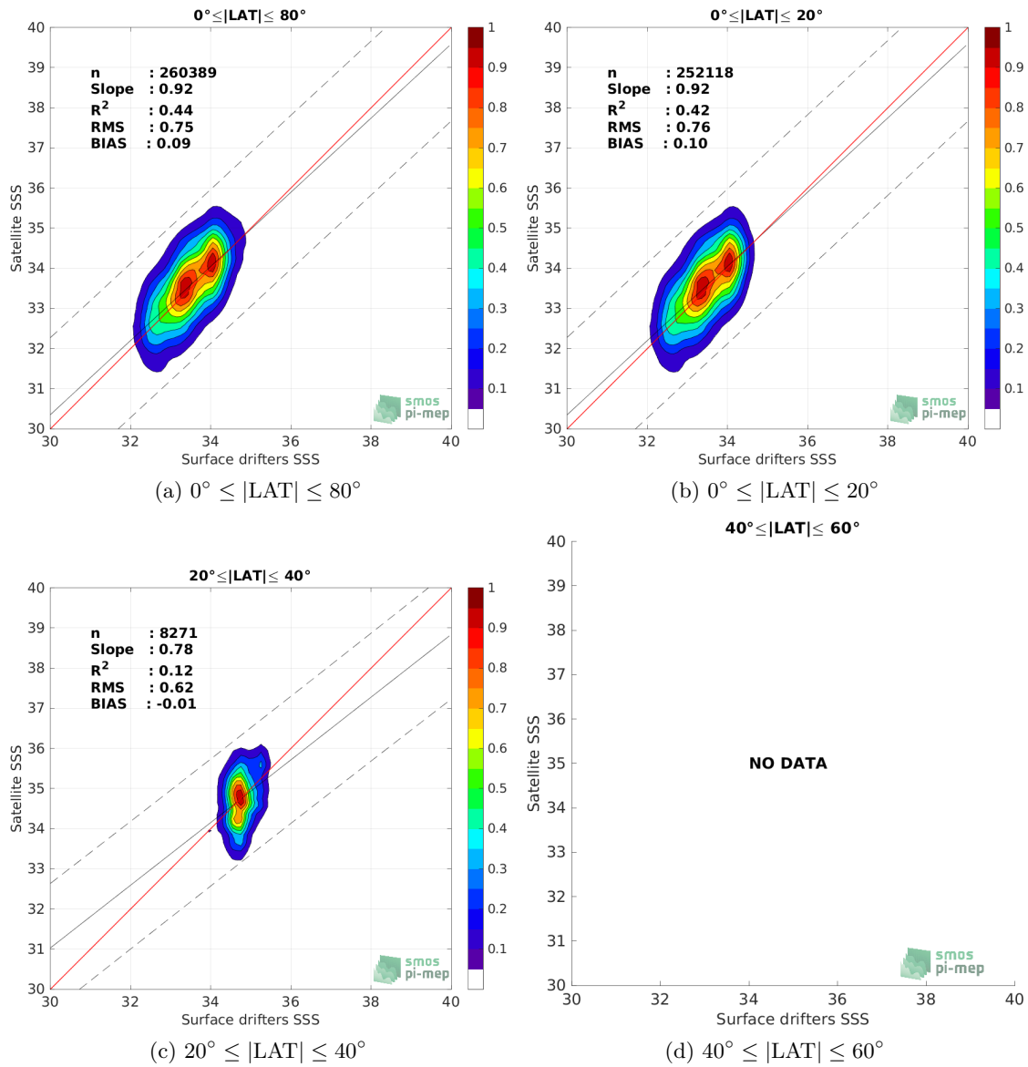
Figure 8: Contour maps of the concentration of SMOS SSS L2Q v331 - No FLAG (CMEMS-CATDS-CPDC) SSS (y-axis) versus Surface drifters SSS (x-axis) at match-up pairs for different latitude bands. For each plot, the red line shows x=y . The black thin and dashed lines indicate a linear fit through the data cloud and the \pm 95\% confidence levels, respectively. The number match-up pairs n , the slope and R^2 coefficient of the linear fit, the root mean square (RMS) and the mean bias between satellite and in situ data are indicated for each latitude band in each plots.
