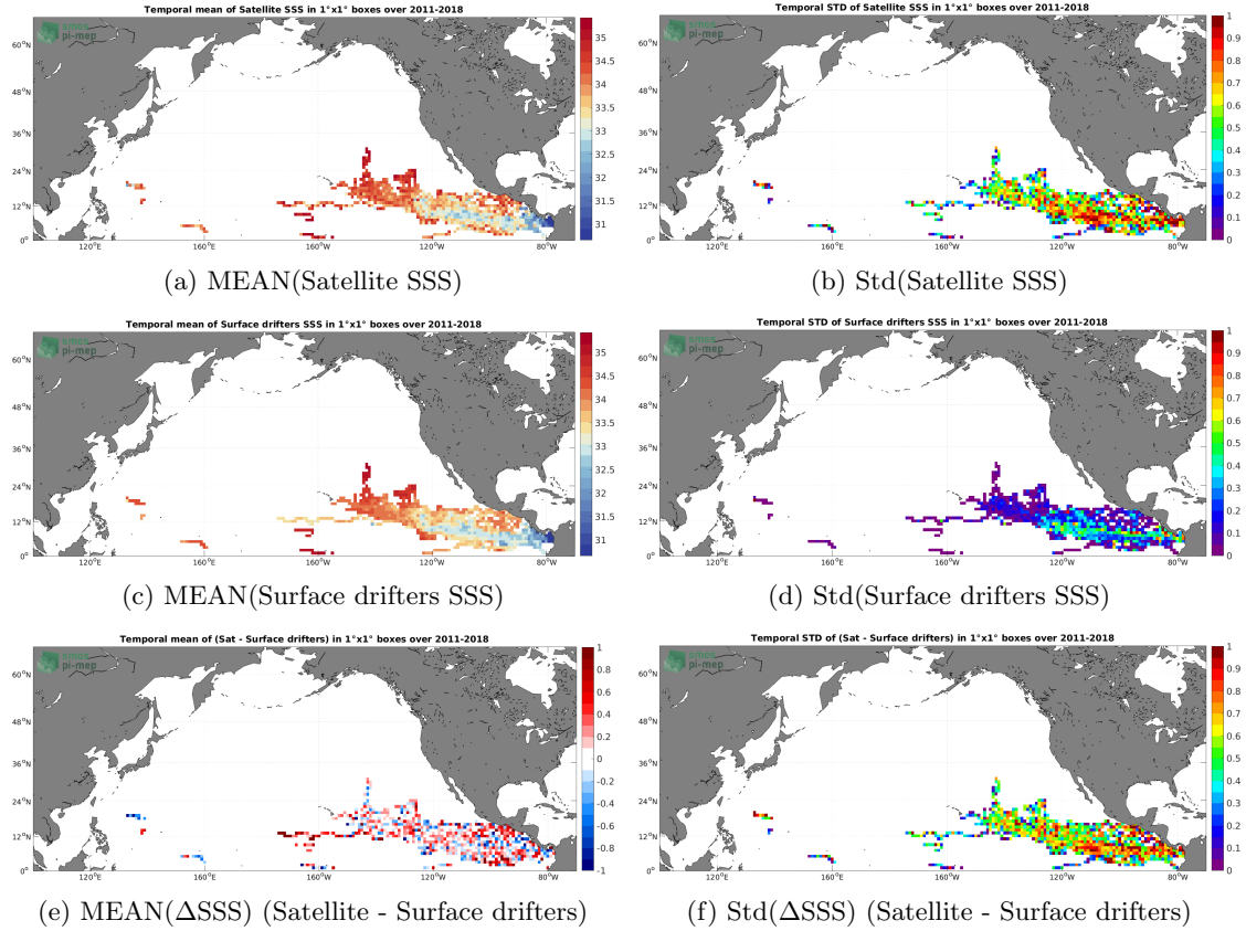
Figure 5: Temporal mean (left) and Std (right) of SSS from SMOS SSS L2Q v331 - No FLAG (CMEMS-CATDS-CPDC) (top), Surface drifters (middle), and of \Delta SSS (Satellite - Surface drifters). Only match-up pairs are used to generate these maps.
