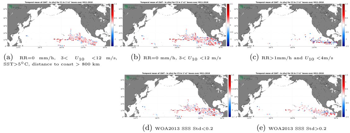
Figure 11: Temporal mean gridded over spatial boxes of size 1^{\circ}\times 1^{\circ} of \Delta\text{SSS} (SMOS SSS L2Q v331 - No FLAG (CMEMS-CATDS-CPDC) - Surface drifters) for 5 different subdatasets corresponding to:RR=0 mm/h, 3 < U_{10} < 12 m/s, SST >5^{\circ}\text{C} , distance to coast > 800 km (a), RR=0 mm/h, 3 < U_{10} < 12 m/s (b), RR >1 mm/h and U_{10} < 4 m/s (c), WOA2013 SSS Std <0.2 (d), WOA2013 SSS Std >0.2 (e).
