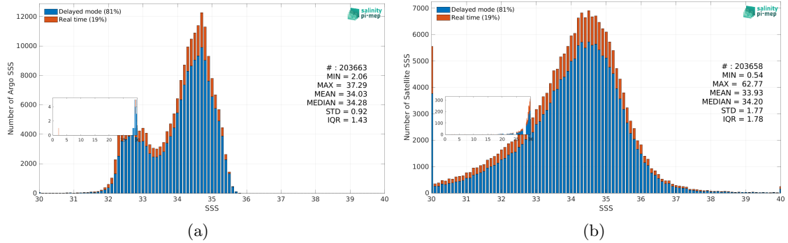
Figure 3: Histograms of SSS from Argo (a) and SMOS SSS L2Q v331 - No FLAG (CMEMS-CATDS-CPDC) (b) considering all match-up pairs per bins of 0.1 over the North Pacific Ocean Pi-MEP region and for the full satellite product period.
