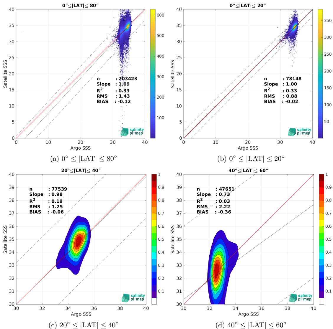
Figure 10: Contour maps of the concentration of SMOS SSS L2Q v331 - No FLAG (CMEMS-CATDS-CPDC) SSS ( y -axis) versus Argo SSS ( x -axis) at match-up pairs for different latitude bands. For each plot, the red line shows x=y . The black thin and dashed lines indicate a linear fit through the data cloud and the \pm 95\% confidence levels, respectively. The number match-up pairs n , the slope and R^2 coefficient of the linear fit, the root mean square (RMS) and the mean bias between satellite and in situ data are indicated for each latitude band in each plots.
