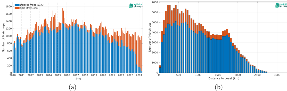
Figure 2: Number of match-ups between Argo and SMOS SSS L2Q v331 - No FLAG (CMEMS-CATDS-CPDC) SSS as a function of time (a) and as function of the distance to coast (b) over the North Pacific Ocean Pi-MEP region and for the full satellite product period.
