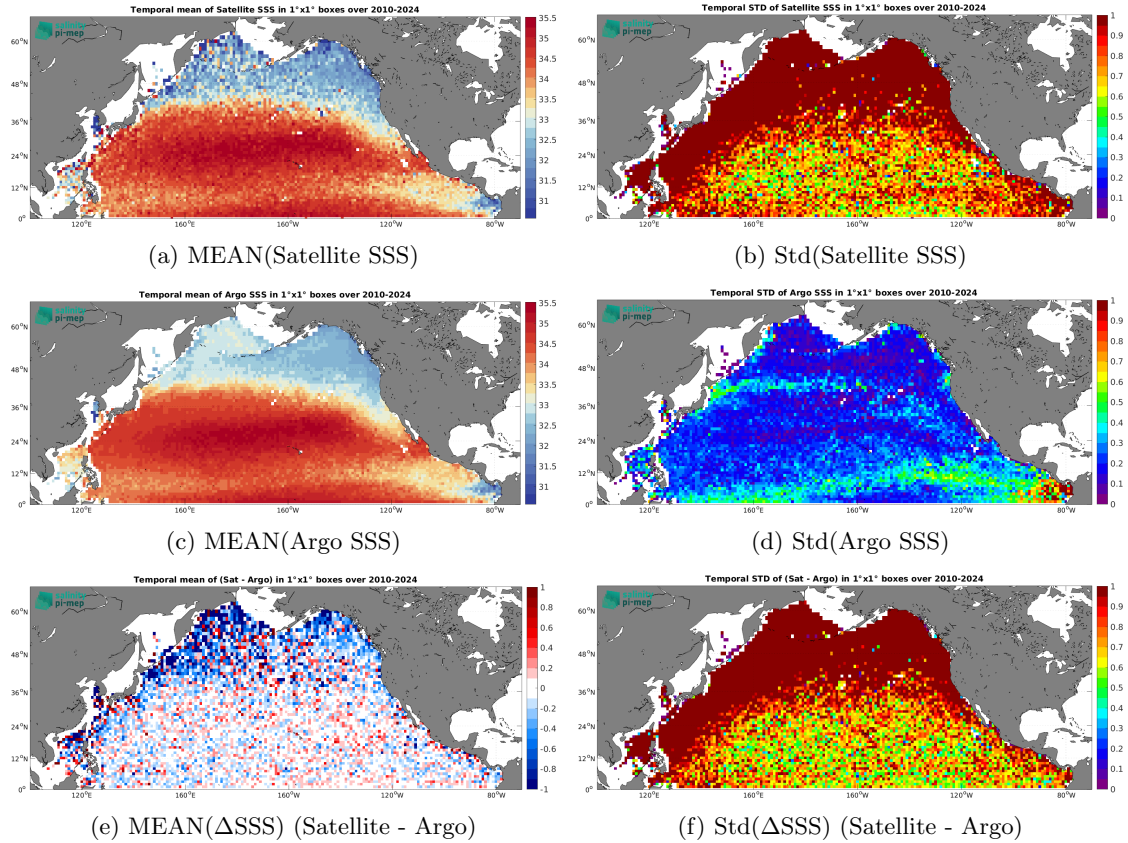
Figure 7: Temporal mean (left) and Std (right) of SSS from SMOS SSS L2Q v331 - No FLAG (CMEMS-CATDS-CPDC) (top), Argo (middle), and of \Delta\text{SSS} (Satellite - Argo). Only match-up pairs are used to generate these maps.
