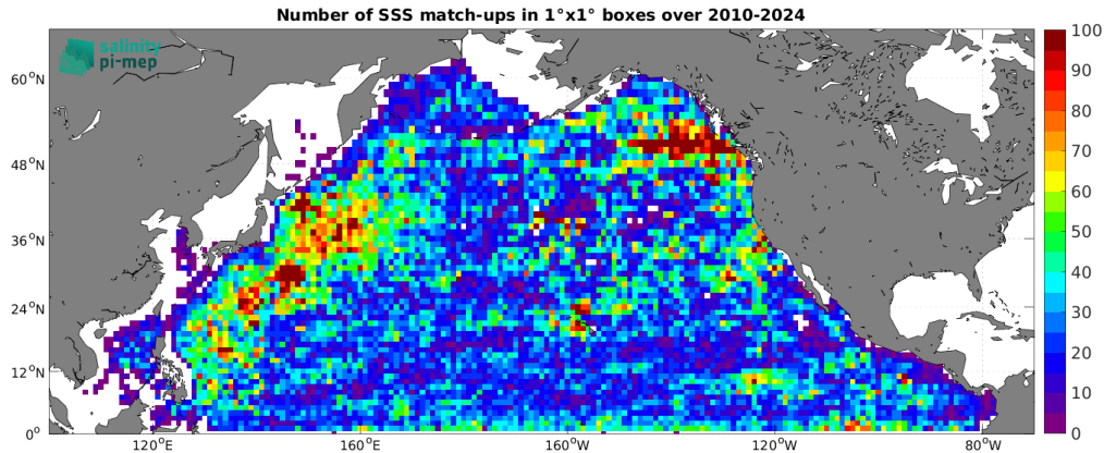
Figure 5: Number of SSS match-ups between Argo SSS and the SMOS SSS L2Q v331 - No FLAG (CMEMS-CATDS-CPDC) SSS product for the North Pacific Ocean Pi-MEP region over 1^\circ \times 1^\circ boxes and for the full satellite product period.
