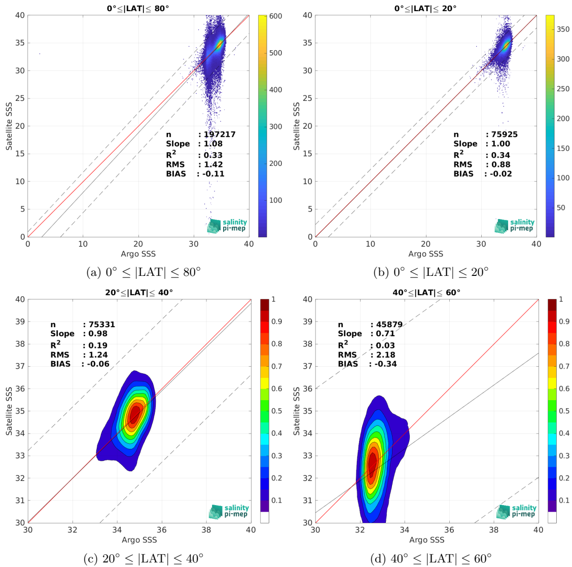
Figure 9: Contour maps of the concentration of SMOS SSS L2Q v331 - No FLAG (CMEMS-CATDS-CPDC) SSS ( y -axis) versus Argo SSS ( x -axis) at match-up pairs for different latitude bands. For each plot, the red line shows x=y . The black thin and dashed lines indicate a linear fit through the data cloud and the \pm 95\% confidence levels, respectively. The number match-up pairs n , the slope and R^2 coefficient of the linear fit, the root mean square (RMS) and the mean bias between satellite and in situ data are indicated for each latitude band in each plots.
