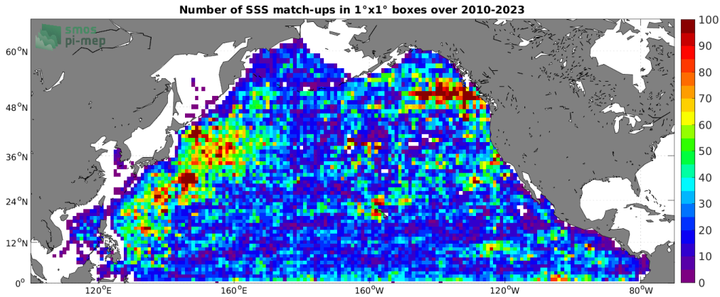
Figure 4: Number of SSS match-ups between Argo SSS and the SMOS SSS L2Q v331 - No FLAG (CMEMS-CATDS-CPDC) SSS product for the North Pacific Ocean Pi-MEP region over 1^\circ \times 1^\circ boxes and for the full satellite product period.
