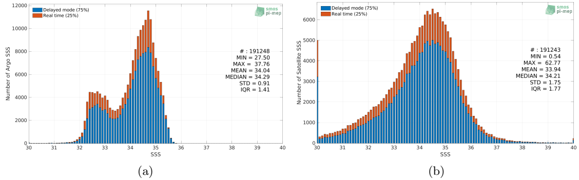
Figure 2: Histograms of SSS from Argo (a) and SMOS SSS L2Q v331 - No FLAG (CMEMS-CATDS-CPDC) (b) considering all match-up pairs per bins of 0.1 over the North Pacific Ocean Pi-MEP region and for the full satellite product period.
