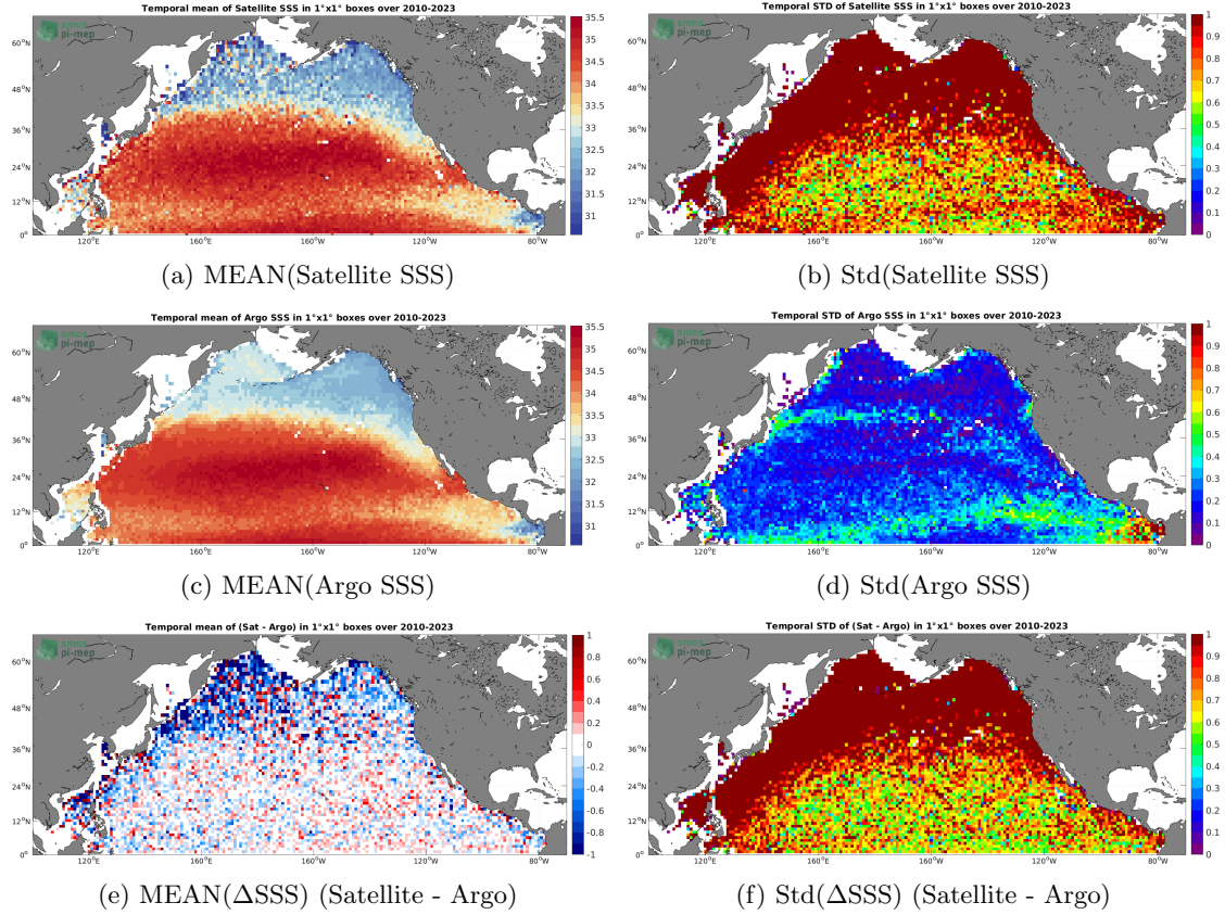
Figure 6: Temporal mean (left) and Std (right) of SSS from SMOS SSS L2Q v331 - No FLAG (CMEMS-CATDS-CPDC) (top), Argo (middle), and of \Delta\text{SSS} (Satellite - Argo). Only match-up pairs are used to generate these maps.
