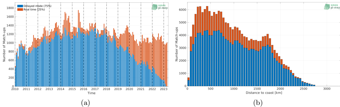
Figure 1: Number of match-ups between Argo and SMOS SSS L2Q v331 - No FLAG (CMEMS-CATDS-CPDC) SSS as a function of time (a) and as function of the distance to coast (b) over the North Pacific Ocean Pi-MEP region and for the full satellite product period.
