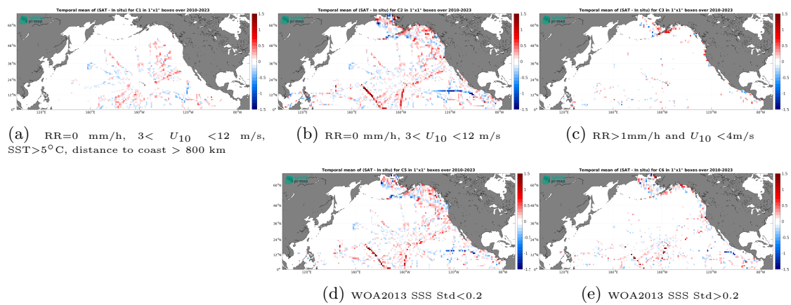
Figure 14: Temporal mean gridded over spatial boxes of size 1^\circ \times 1^\circ of \Delta SSS (SMOS SSS L3 v9 - 9 Days (CATDS-CEC-LOCEAN) - TSG (SAMOS)) for 5 different subdatasets corresponding to:RR=0 mm/h, 3 < U_{10} < 12 m/s, SST >5^\circ\text{C} , distance to coast > 800 km (a), RR=0 mm/h, 3 < U_{10} < 12 m/s (b), RR >1 mm/h and U_{10} < 4 m/s (c), WOA2013 SSS Std <0.2 (d), WOA2013 SSS Std >0.2 (e).
