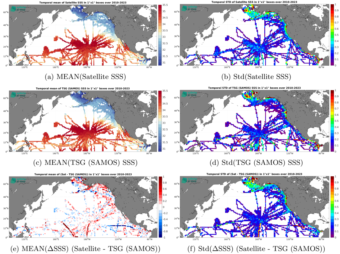
Figure 7: Temporal mean (left) and Std (right) of SSS from SMOS SSS L3 v9 - 9 Days (CATDS-CEC-LOCEAN) (top), TSG (SAMOS) (middle), and of \Delta\text{SSS} (Satellite - TSG (SAMOS)). Only match-up pairs are used to generate these maps.
