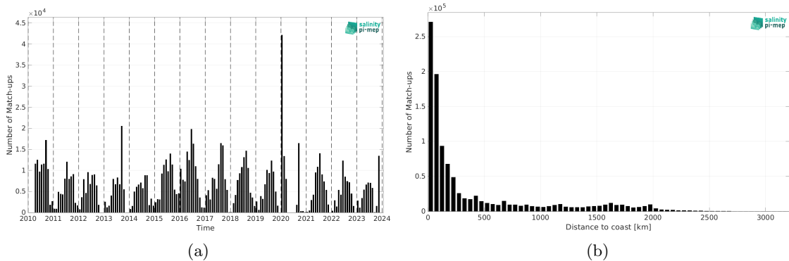
Figure 2: Number of match-ups between TSG (SAMOS) and SMOS SSS L3 v9 - 9 Days (CATDS-CEC-LOCEAN) SSS as a function of time (a) and as function of the distance to coast (b) over the North Pacific Ocean Pi-MEP region and for the full satellite product period.
