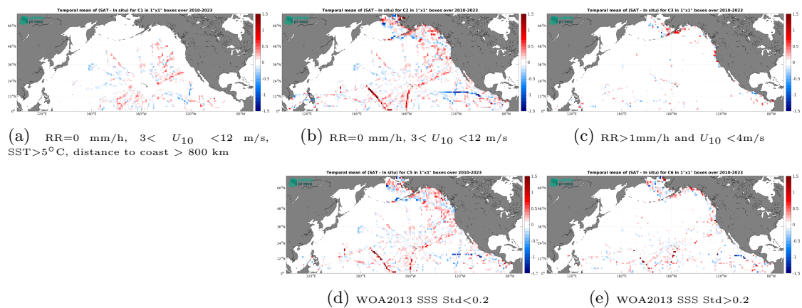
Figure 14: Temporal mean gridded over spatial boxes of size 1^\circ \times 1^\circ of \Delta\text{SSS} (SMOS SSS L3 v9 - 9 Days (CATDS-CEC-LOCEAN) - TSG (SAMOS)) for 5 different subdatasets corresponding to: RR=0 mm/h, 3 < U_{10} < 12 m/s, SST > 5°C, distance to coast > 800 km (a), RR=0 mm/h, 3 < U_{10} < 12 m/s (b), RR > 1mm/h and U_{10} < 4 m/s (c), WOA2013 SSS Std < 0.2 (d), WOA2013 SSS Std > 0.2 (e).
