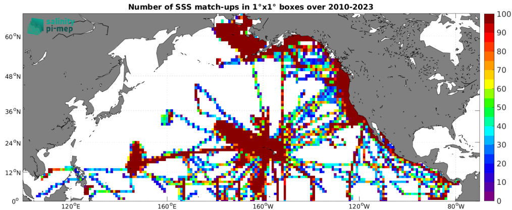
Figure 5: Number of SSS match-ups between TSG (SAMOS) SSS and the SMOS SSS L3 v9 - 9 Days (CATDS-CEC-LOCEAN) SSS product for the North Pacific Ocean Pi-MEP region over 1^\circ \times 1^\circ boxes and for the full satellite product period.
