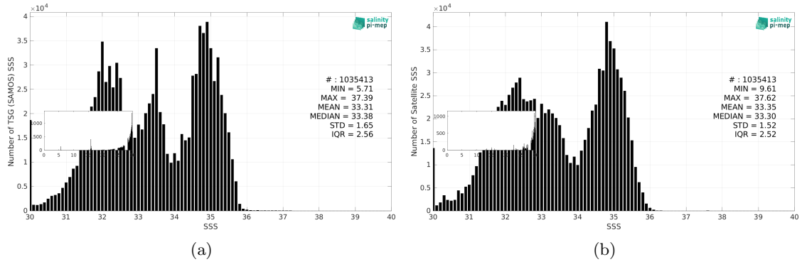
Figure 3: Histograms of SSS from TSG (SAMOS) (a) and SMOS SSS L3 v9 - 9 Days (CATDS-CEC-LOCEAN) (b) considering all match-up pairs per bins of 0.1 over the North Pacific Ocean Pi-MEP region and for the full satellite product period.
