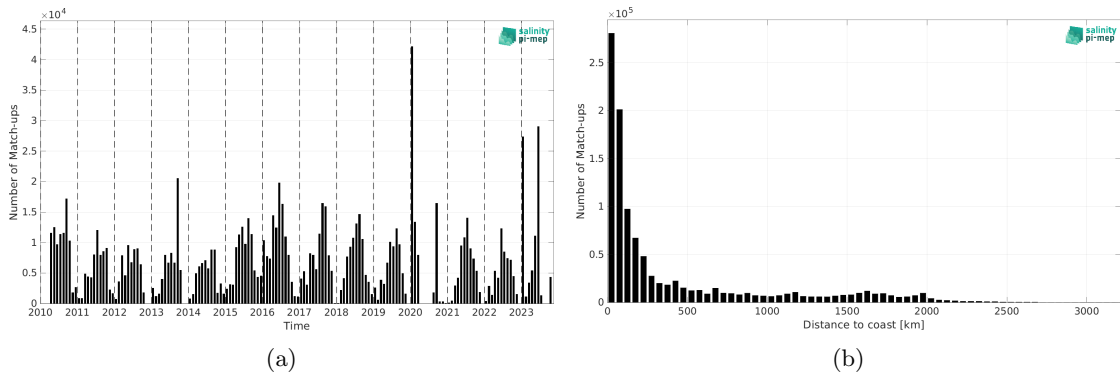
Figure 1: Number of match-ups between TSG (SAMOS) and SMOS SSS L3 v9 - 9 Days (CATDS-CEC-LOCEAN) SSS as a function of time (a) and as function of the distance to coast (b) over the North Pacific Ocean Pi-MEP region and for the full satellite product period.
