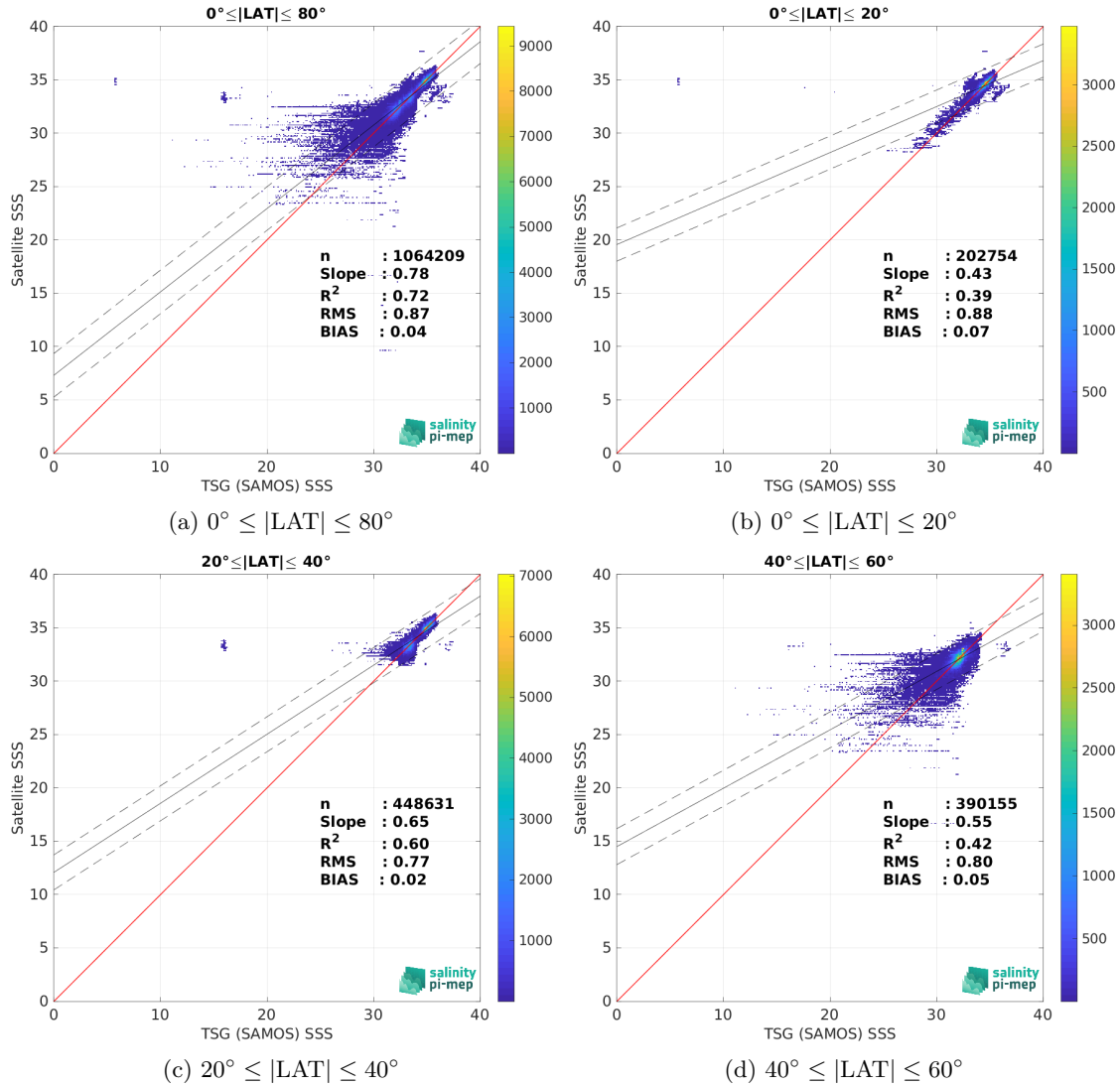
Figure 9: Contour maps of the concentration of SMOS SSS L3 v9 - 9 Days (CATDS-CEC-LOCEAN) SSS (y-axis) versus TSG (SAMOS) SSS (x-axis) at match-up pairs for different latitude bands. For each plot, the red line shows x=y . The black thin and dashed lines indicate a linear fit through the data cloud and the \pm 95\% confidence levels, respectively. The number match-up pairs n , the slope and R^2 coefficient of the linear fit, the root mean square (RMS) and the mean bias between satellite and in situ data are indicated for each latitude band in each plots.
