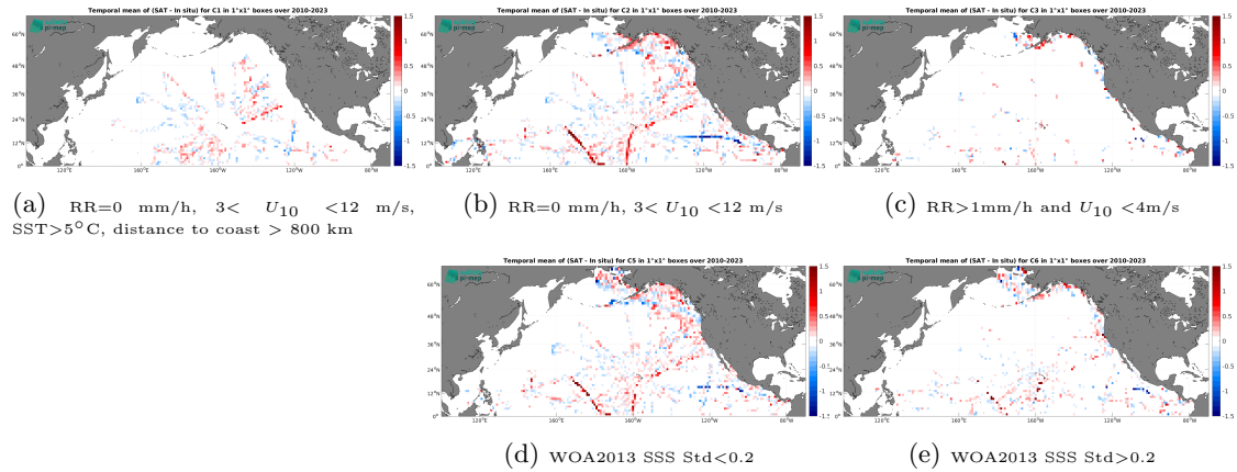
Figure 12: Temporal mean gridded over spatial boxes of size 1^\circ \times 1^\circ of \Delta SSS (SMOS SSS L3 v9 - 9 Days (CATDS-CEC-LOCEAN) - TSG (SAMOS)) for 5 different subdatasets corresponding to:RR=0 mm/h, 3 < U_{10} < 12 m/s, SST >5^\circ C, distance to coast > 800 km (a), RR=0 mm/h, 3 < U_{10} < 12 m/s (b), RR >1 mm/h and U_{10} < 4 m/s (c), WOA2013 SSS Std <0.2 (d), WOA2013 SSS Std >0.2 (e).
