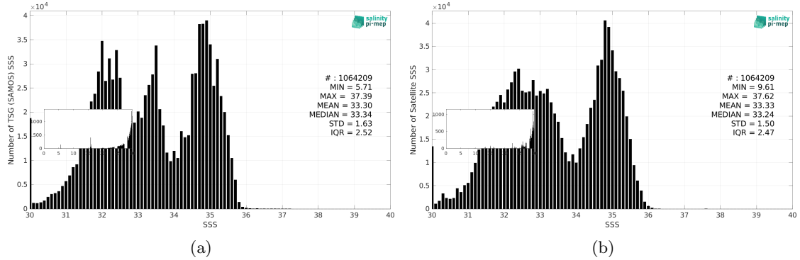
Figure 2: Histograms of SSS from TSG (SAMOS) (a) and SMOS SSS L3 v9 - 9 Days (CATDS-CEC-LOCEAN) (b) considering all match-up pairs per bins of 0.1 over the North Pacific Ocean Pi-MEP region and for the full satellite product period.
