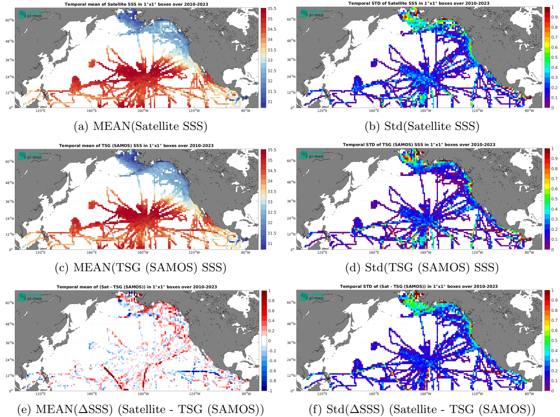
Figure 6: Temporal mean (left) and Std (right) of SSS from SMOS SSS L3 v9 - 9 Days (CATDS-CEC-LOCEAN) (top), TSG (SAMOS) (middle), and of \Delta SSS (Satellite - TSG (SAMOS)). Only match-up pairs are used to generate these maps.
