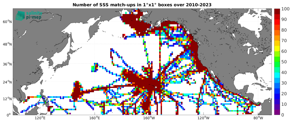
Figure 4: Number of SSS match-ups between TSG (SAMOS) SSS and the SMOS SSS L3 v9 - 9 Days (CATDS-CEC-LOCEAN) SSS product for the North Pacific Ocean Pi-MEP region over 1^\circ \times 1^\circ boxes and for the full satellite product period.
