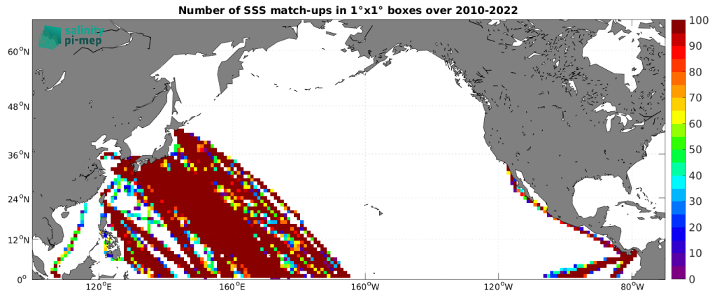
Figure 5: Number of SSS match-ups between TSG (LEGOS-DM) SSS and the SMOS SSS L3 v9 - 9 Days (CATDS-CEC-LOCEAN) SSS product for the North Pacific Ocean Pi-MEP region over 1^\circ \times 1^\circ boxes and for the full satellite product period.
