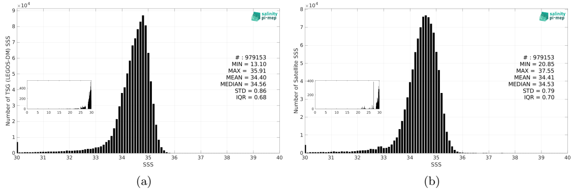
Figure 3: Histograms of SSS from TSG (LEGOS-DM) (a) and SMOS SSS L3 v9 - 9 Days (CATDS-CEC-LOCEAN) (b) considering all match-up pairs per bins of 0.1 over the North Pacific Ocean Pi-MEP region and for the full satellite product period.
