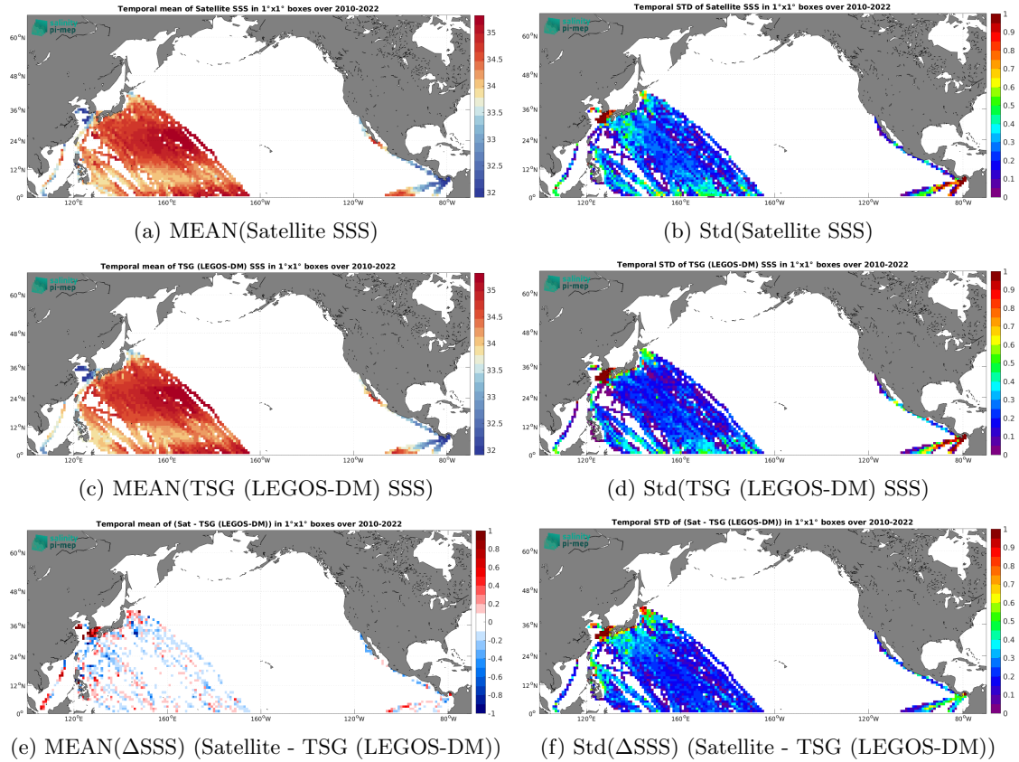
Figure 7: Temporal mean (left) and Std (right) of SSS from SMOS SSS L3 v9 - 9 Days (CATDS-CEC-LOCEAN) (top), TSG (LEGOS-DM) (middle), and of \Delta\text{SSS} (Satellite - TSG (LEGOS-DM)). Only match-up pairs are used to generate these maps.
