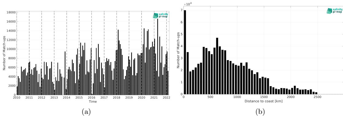
Figure 2: Number of match-ups between TSG (LEGOS-DM) and SMOS SSS L3 v9 - 9 Days (CATDS-CEC-LOCEAN) SSS as a function of time (a) and as function of the distance to coast (b) over the North Pacific Ocean Pi-MEP region and for the full satellite product period.
