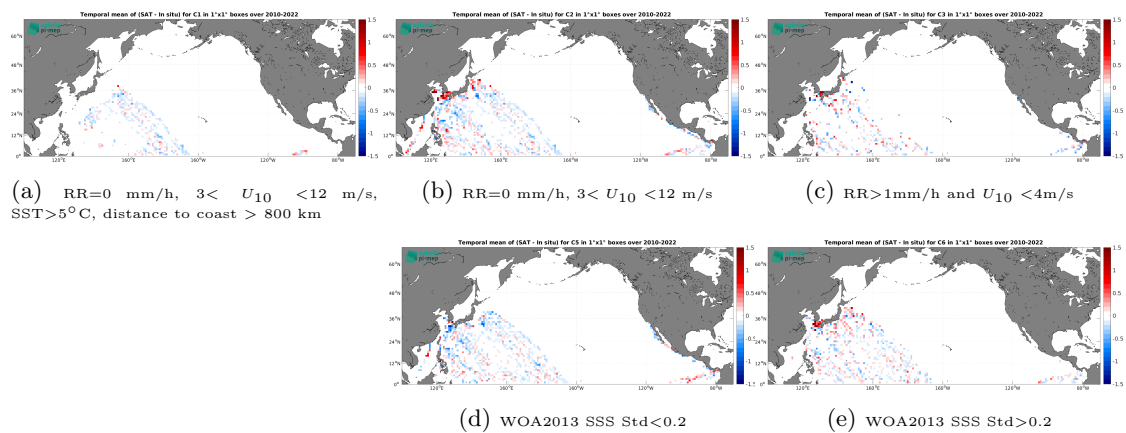
Figure 14: Temporal mean gridded over spatial boxes of size 1^\circ \times 1^\circ of \Delta\text{SSS} (SMOS SSS L3 v9 - 9 Days (CATDS-CEC-LOCEAN) - TSG (LEGOS-DM)) for 5 different subdatasets corresponding to:RR=0 mm/h, 3 < U_{10} < 12 m/s, SST>5°C, distance to coast > 800 km (a), RR=0 mm/h, 3 < U_{10} < 12 m/s (b), RR>1mm/h and U_{10} < 4 m/s (c), WOA2013 SSS Std<0.2 (d), WOA2013 SSS Std>0.2 (e).
