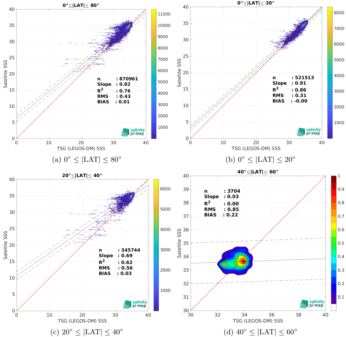
Figure 9: Contour maps of the concentration of SMOS SSS L3 v9 - 9 Days (CATDS-CEC-LOCEAN) SSS (y-axis) versus TSG (LEGOS-DM) SSS (x-axis) at match-up pairs for different latitude bands. For each plot, the red line shows x=y . The black thin and dashed lines indicate a linear fit through the data cloud and the \pm 95\% confidence levels, respectively. The number of match-up pairs n , the slope and R^2 coefficient of the linear fit, the root mean square (RMS) and the mean bias between satellite and in situ data are indicated for each latitude band in each plot.
