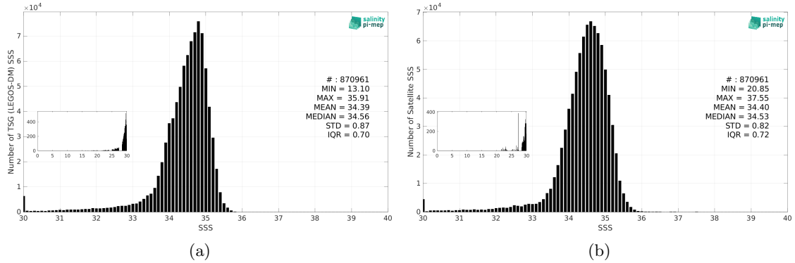
Figure 2: Histograms of SSS from TSG (LEGOS-DM) (a) and SMOS SSS L3 v9 - 9 Days (CATDS-CEC-LOCEAN) (b) considering all match-up pairs per bins of 0.1 over the North Pacific Ocean Pi-MEP region and for the full satellite product period.
