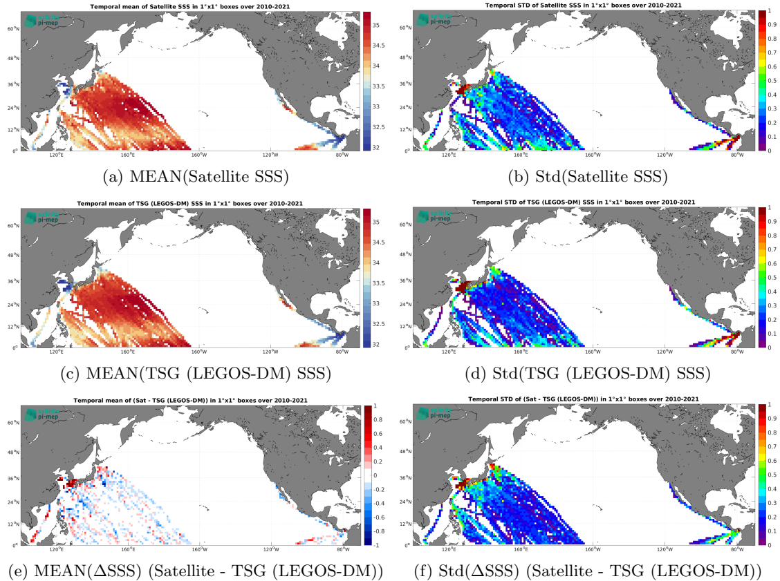
Figure 6: Temporal mean (left) and Std (right) of SSS from SMOS SSS L3 v9 - 9 Days (CATDS-CEC-LOCEAN) (top), TSG (LEGOS-DM) (middle), and of \Delta\text{SSS} (Satellite - TSG (LEGOS-DM)). Only match-up pairs are used to generate these maps.
