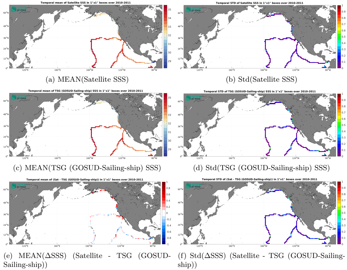
Figure 7: Temporal mean (left) and Std (right) of SSS from SMOS SSS L3 v9 - 9 Days (CATDS-CEC-LOCEAN) (top), TSG (GOSUD-Sailing-ship) (middle), and of \Delta SSS (Satellite - TSG (GOSUD-Sailing-ship)). Only match-up pairs are used to generate these maps.
