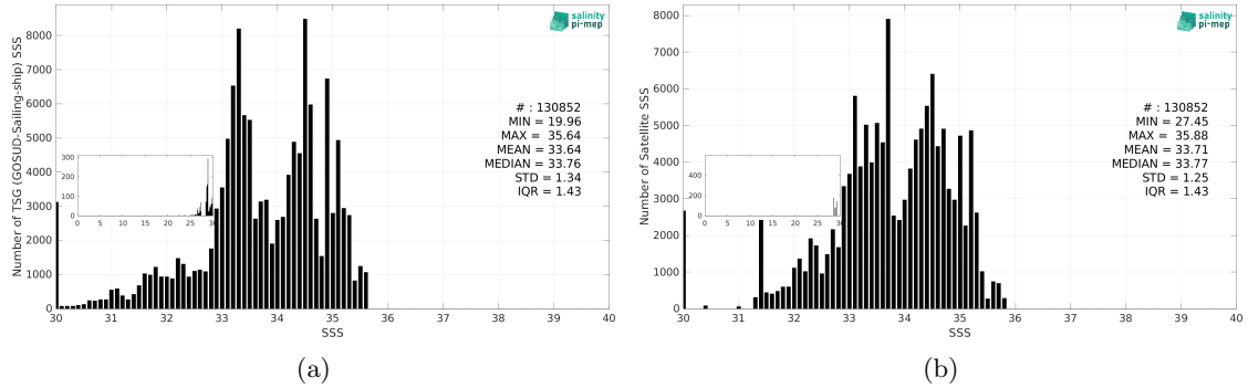
Figure 2: Histograms of SSS from TSG (GOSUD-Sailing-ship) (a) and SMOS SSS L3 v9 - 9 Days (CATDS-CEC-LOCEAN) (b) considering all match-up pairs per bins of 0.1 over the North Pacific Ocean Pi-MEP region and for the full satellite product period.
