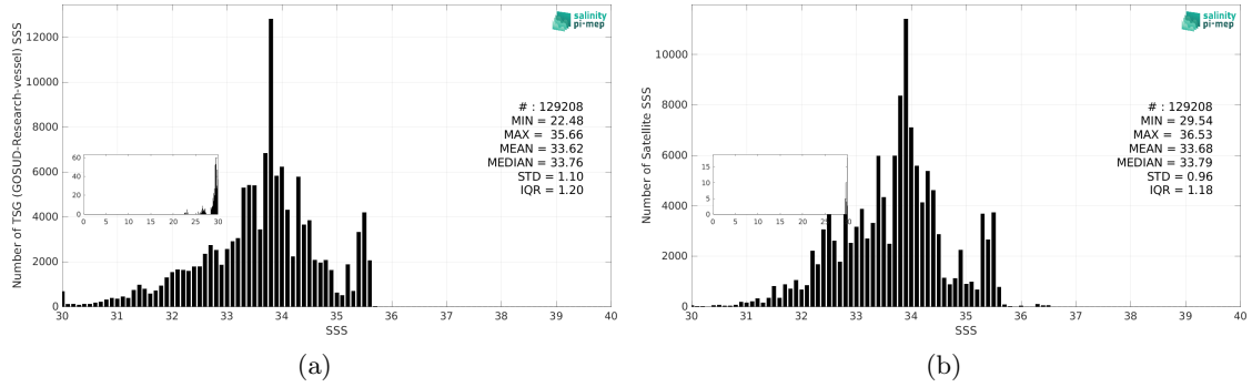
Figure 3: Histograms of SSS from TSG (GOSUD-Research-vessel) (a) and SMOS SSS L3 v9 - 9 Days (CATDS-CEC-LOCEAN) (b) considering all match-up pairs per bins of 0.1 over the North Pacific Ocean Pi-MEP region and for the full satellite product period.
