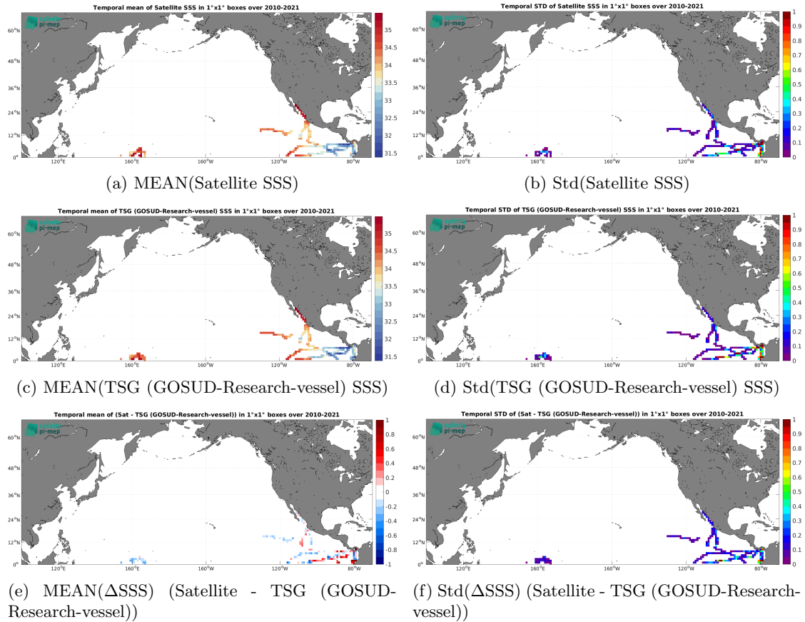
Figure 7: Temporal mean (left) and Std (right) of SSS from SMOS SSS L3 v9 - 9 Days (CATDS-CEC-LOCEAN) (top), TSG (GOSUD-Research-vessel) (middle), and of \Delta SSS (Satellite - TSG (GOSUD-Research-vessel)). Only match-up pairs are used to generate these maps.
