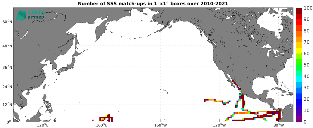
Figure 5: Number of SSS match-ups between TSG (GOSUD-Research-vessel) SSS and the SMOS SSS L3 v9 - 9 Days (CATDS-CEC-LOCEAN) SSS product for the North Pacific Ocean Pi-MEP region over 1^\circ \times 1^\circ boxes and for the full satellite product period.
