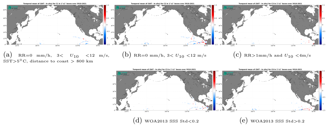
Figure 14: Temporal mean gridded over spatial boxes of size 1^\circ \times 1^\circ of \Delta\text{SSS} (SMOS SSS L3 v9 - 9 Days (CATDS-CEC-LOCEAN) - TSG (GOSUD-Research-vessel)) for 5 different subdatasets corresponding to:RR=0 mm/h, 3 < U_{10} < 12 m/s, SST >5^\circ\text{C} , distance to coast > 800 km (a), RR=0 mm/h, 3 < U_{10} < 12 m/s (b), RR >1 mm/h and U_{10} < 4 m/s (c), WOA2013 SSS Std <0.2 (d), WOA2013 SSS Std >0.2 (e).
