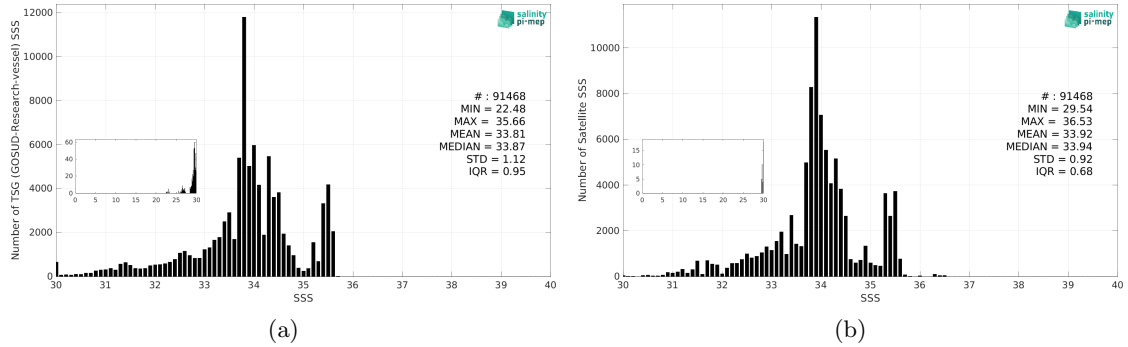
Figure 3: Histograms of SSS from TSG (GOSUD-Research-vessel) (a) and SMOS SSS L3 v9 - 9 Days (CATDS-CEC-LOCEAN) (b) considering all match-up pairs per bins of 0.1 over the North Pacific Ocean Pi-MEP region and for the full satellite product period.
