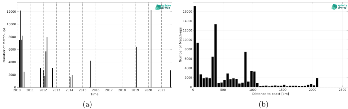
Figure 1: Number of match-ups between TSG (GOSUD-Research-vessel) and SMOS SSS L3 v9 - 9 Days (CATDS-CEC-LOCEAN) SSS as a function of time (a) and as function of the distance to coast (b) over the North Pacific Ocean Pi-MEP region and for the full satellite product period.
