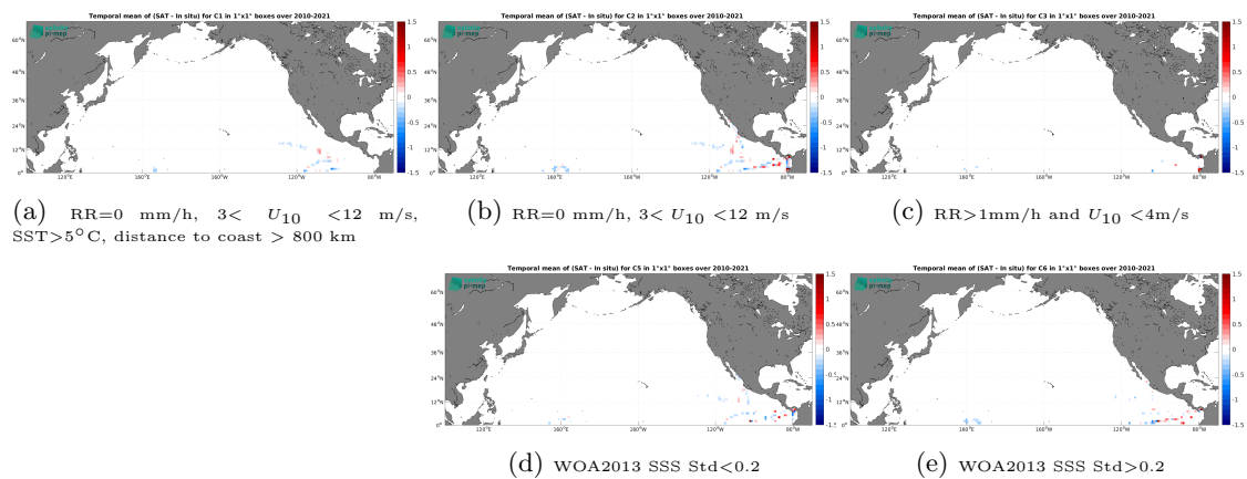
Figure 12: Temporal mean gridded over spatial boxes of size 1^\circ \times 1^\circ of \Delta\text{SSS} (SMOS SSS L3 v9 - 9 Days (CATDS-CEC-LOCEAN) - TSG (GOSUD-Research-vessel)) for 5 different subdatasets corresponding to: RR=0 mm/h, 3 < U_{10} < 12 m/s, SST > 5°C, distance to coast > 800 km (a), RR=0 mm/h, 3 < U_{10} < 12 m/s (b), RR > 1mm/h and U_{10} < 4 m/s (c), WOA2013 SSS Std < 0.2 (d), WOA2013 SSS Std > 0.2 (e).
