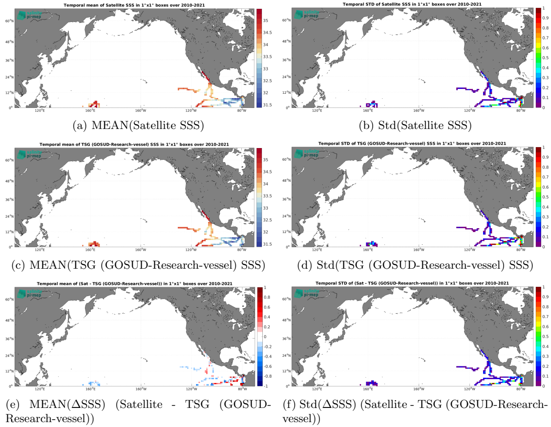
Figure 6: Temporal mean (left) and Std (right) of SSS from SMOS SSS L3 v9 - 9 Days (CATDS-CEC-LOCEAN) (top), TSG (GOSUD-Research-vessel) (middle), and of \Delta SSS (Satellite - TSG (GOSUD-Research-vessel)). Only match-up pairs are used to generate these maps.
