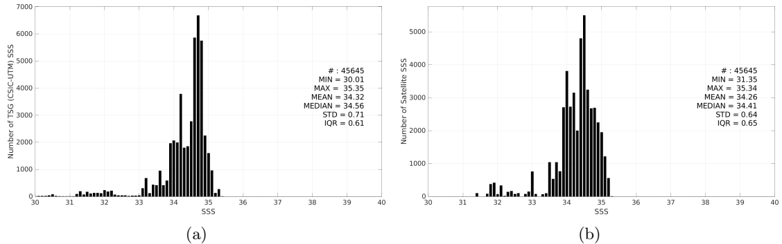
Figure 3: Histograms of SSS from TSG (CSIC-UTM) (a) and SMOS SSS L3 v9 - 9 Days (CATDS-CEC-LOCEAN) (b) considering all match-up pairs per bins of 0.1 over the North Pacific Ocean Pi-MEP region and for the full satellite product period.
