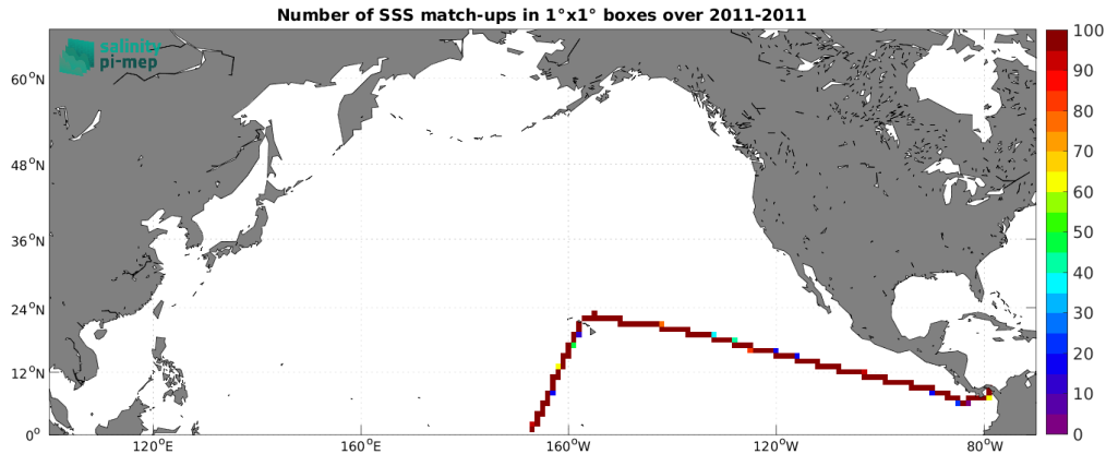
Figure 5: Number of SSS match-ups between TSG (CSIC-UTM) SSS and the SMOS SSS L3 v9 - 9 Days (CATDS-CEC-LOCEAN) SSS product for the North Pacific Ocean Pi-MEP region over 1^\circ \times 1^\circ boxes and for the full satellite product period.
