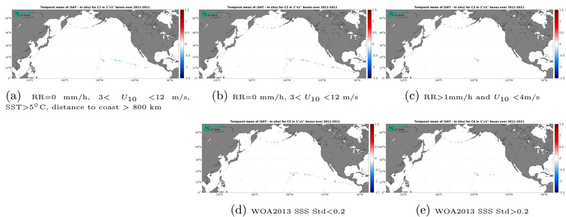
Figure 14: Temporal mean gridded over spatial boxes of size 1^\circ \times 1^\circ of \Delta SSS (SMOS SSS L3 v9 - 9 Days (CATDS-CEC-LOCEAN) - TSG (CSIC-UTM)) for 5 different subdatasets corresponding to:RR=0 mm/h, 3 < U_{10} < 12 m/s, SST>5°C, distance to coast > 800 km (a), RR=0 mm/h, 3 < U_{10} < 12 m/s (b), RR>1mm/h and U_{10} < 4 m/s (c), WOA2013 SSS Std<0.2 (d), WOA2013 SSS Std>0.2 (e).
