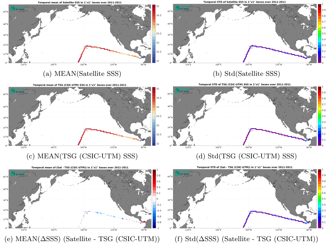
Figure 7: Temporal mean (left) and Std (right) of SSS from SMOS SSS L3 v9 - 9 Days (CATDS-CEC-LOCEAN) (top), TSG (CSIC-UTM) (middle), and of \Delta\text{SSS} (Satellite - TSG (CSIC-UTM)). Only match-up pairs are used to generate these maps.
