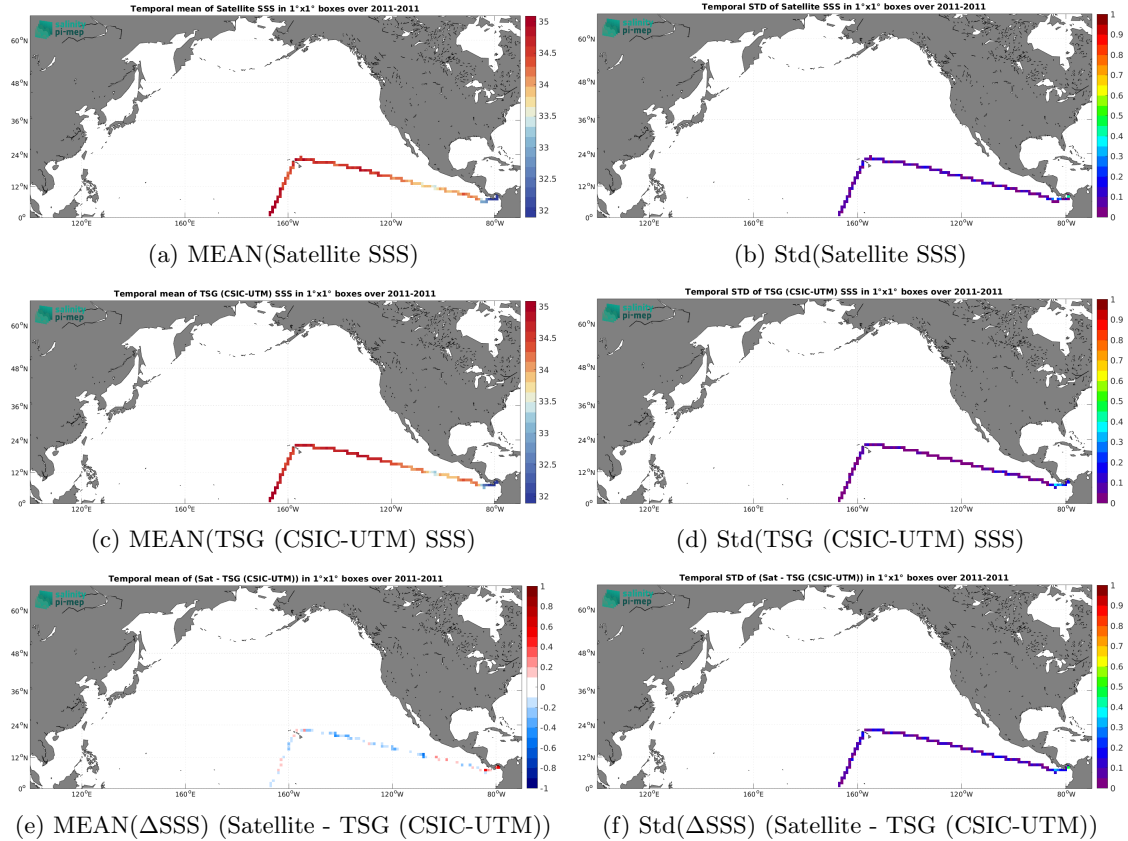
Figure 6: Temporal mean (left) and Std (right) of SSS from SMOS SSS L3 v9 - 9 Days (CATDS-CEC-LOCEAN) (top), TSG (CSIC-UTM) (middle), and of \Delta\text{SSS} (Satellite - TSG (CSIC-UTM)). Only match-up pairs are used to generate these maps.
