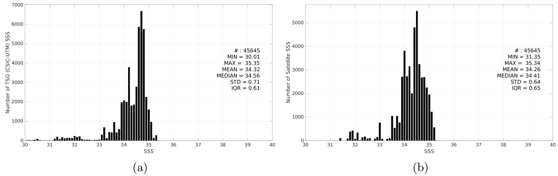
Figure 2: Histograms of SSS from TSG (CSIC-UTM) (a) and SMOS SSS L3 v9 - 9 Days (CATDS-CEC-LOCEAN) (b) considering all match-up pairs per bins of 0.1 over the North Pacific Ocean Pi-MEP region and for the full satellite product period.
