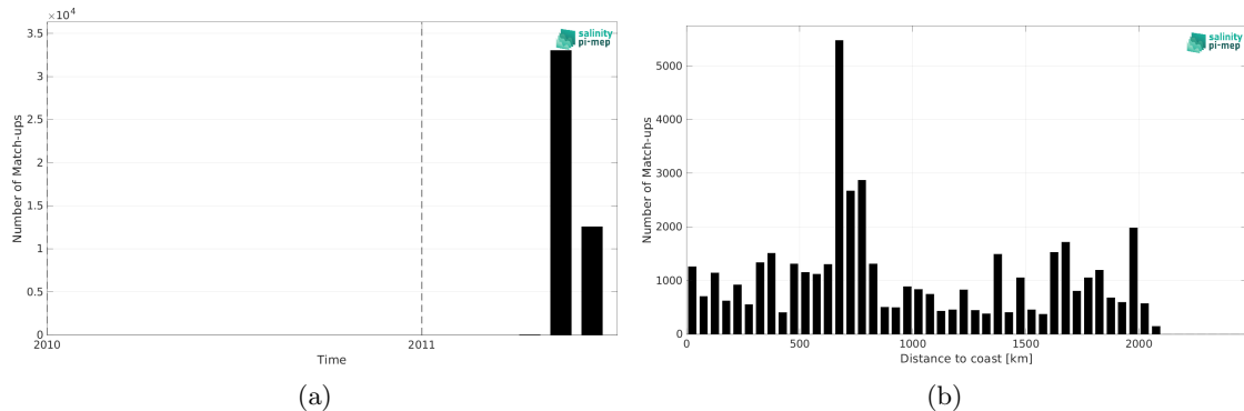
Figure 1: Number of match-ups between TSG (CSIC-UTM) and SMOS SSS L3 v9 - 9 Days (CATDS-CEC-LOCEAN) SSS as a function of time (a) and as function of the distance to coast (b) over the North Pacific Ocean Pi-MEP region and for the full satellite product period.
