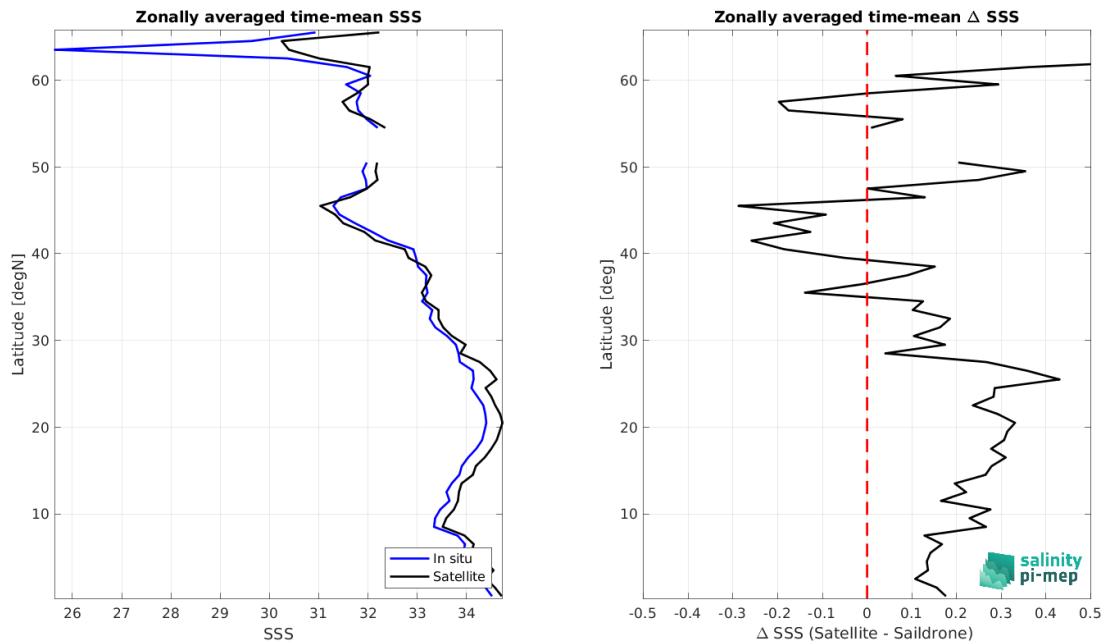
Figure 8: Left panel: Zonal mean SSS from SMOS SSS L3 v9 - 9 Days (CATDS-CEC-LOCEAN) satellite product (black) and from Saildrone (blue). Right panel: Zonal mean of \Delta SSS (Satellite - Saildrone) for all the collected Pi-MEP match-up pairs estimated over the full satellite product period.
