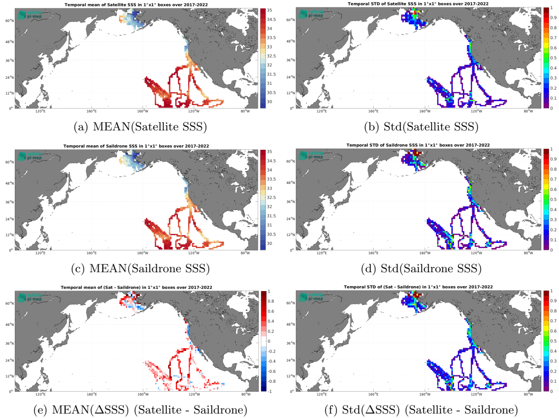
Figure 6: Temporal mean (left) and Std (right) of SSS from SMOS SSS L3 v9 - 9 Days (CATDS-CEC-LOCEAN) (top), Saildrone (middle), and of \Delta SSS (Satellite - Saildrone). Only match-up pairs are used to generate these maps.
