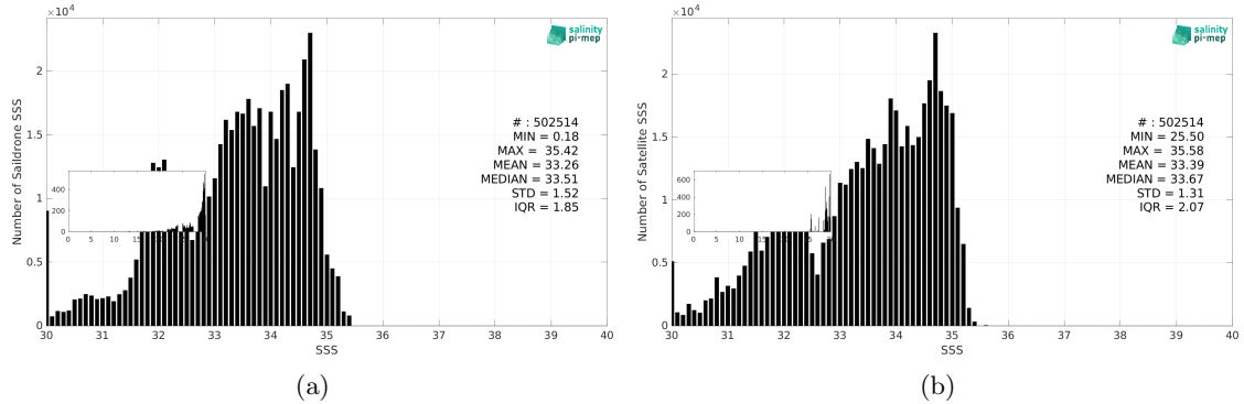
Figure 2: Histograms of SSS from Saildrone (a) and SMOS SSS L3 v9 - 9 Days (CATDS-CEC-LOCEAN) (b) considering all match-up pairs per bins of 0.1 over the North Pacific Ocean Pi-MEP region and for the full satellite product period.
