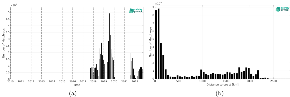
Figure 1: Number of match-ups between Saildrone and SMOS SSS L3 v9 - 9 Days (CATDS-CEC-LOCEAN) SSS as a function of time (a) and as function of the distance to coast (b) over the North Pacific Ocean Pi-MEP region and for the full satellite product period.
