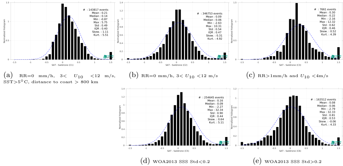
Figure 13: Normalized histogram of \Delta SSS (SMOS SSS L3 v9 - 9 Days (CATDS-CEC-LOCEAN) - Saildrone) for 5 different subdatasets corresponding to: RR=0 mm/h, 3 < U_{10} < 12 m/s, SST>5°C, distance to coast > 800 km (a), RR=0 mm/h, 3 < U_{10} < 12 m/s (b), RR>1mm/h and U_{10} < 4 m/s (c), WOA2013 SSS Std<0.2 (d), WOA2013 SSS Std>0.2 (e).
