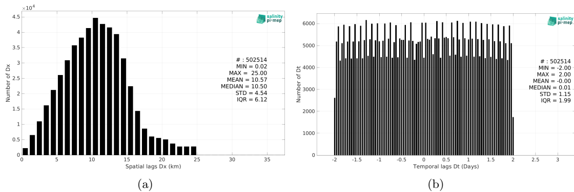
Figure 5: Histograms of the spatial (a) and temporal (b) lags between the location/time of the Saildrone measurement and the date of the corresponding SMOS SSS L3 v9 - 9 Days (CATDS-CEC-LOCEAN) SSS pixel.
