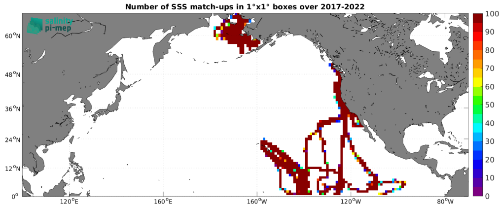
Figure 4: Number of SSS match-ups between Saildrone SSS and the SMOS SSS L3 v9 - 9 Days (CATDS-CEC-LOCEAN) SSS product for the North Pacific Ocean Pi-MEP region over 1^\circ \times 1^\circ boxes and for the full satellite product period.
