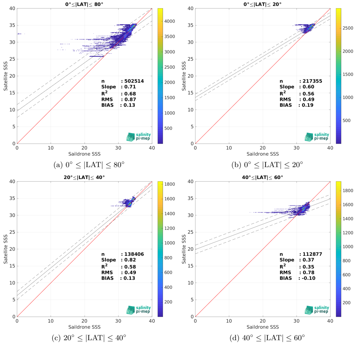
Figure 9: Contour maps of the concentration of SMOS SSS L3 v9 - 9 Days (CATDS-CEC-LOCEAN) SSS (y-axis) versus Sairdrone SSS (x-axis) at match-up pairs for different latitude bands. For each plot, the red line shows x=y . The black thin and dashed lines indicate a linear fit through the data cloud and the \pm 95\% confidence levels, respectively. The number match-up pairs n , the slope and R^2 coefficient of the linear fit, the root mean square (RMS) and the mean bias between satellite and in situ data are indicated for each latitude band in each plots.
