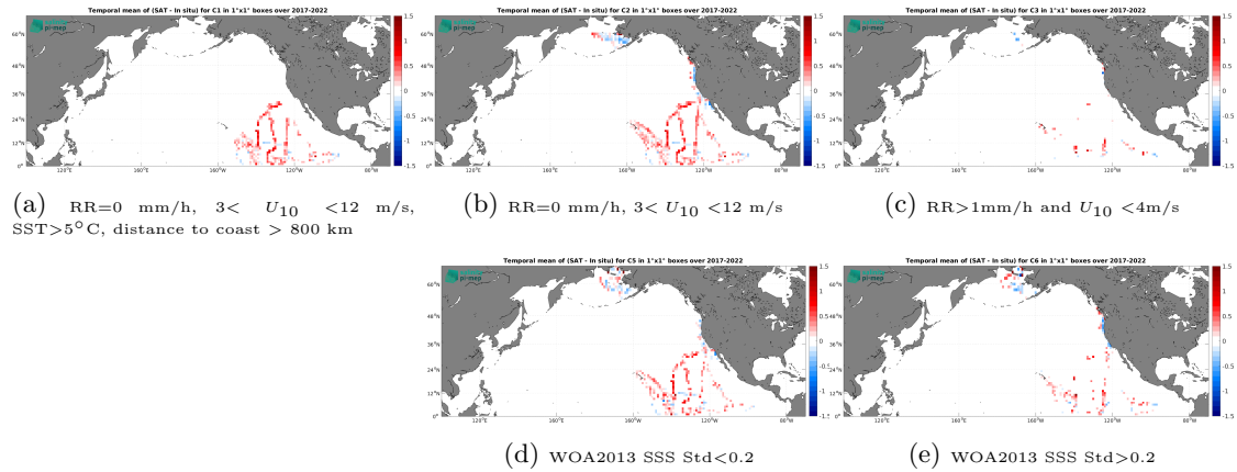
Figure 12: Temporal mean gridded over spatial boxes of size 1^\circ \times 1^\circ of \Delta SSS (SMOS SSS L3 v9 - 9 Days (CATDS-CEC-LOCEAN) - Sailldrone) for 5 different subdatasets corresponding to:RR=0 mm/h, 3 < U_{10} < 12 m/s, SST>5°C, distance to coast > 800 km (a), RR=0 mm/h, 3 < U_{10} < 12 m/s (b), RR>1mm/h and U_{10} < 4 m/s (c), WOA2013 SSS Std<0.2 (d), WOA2013 SSS Std>0.2 (e).
