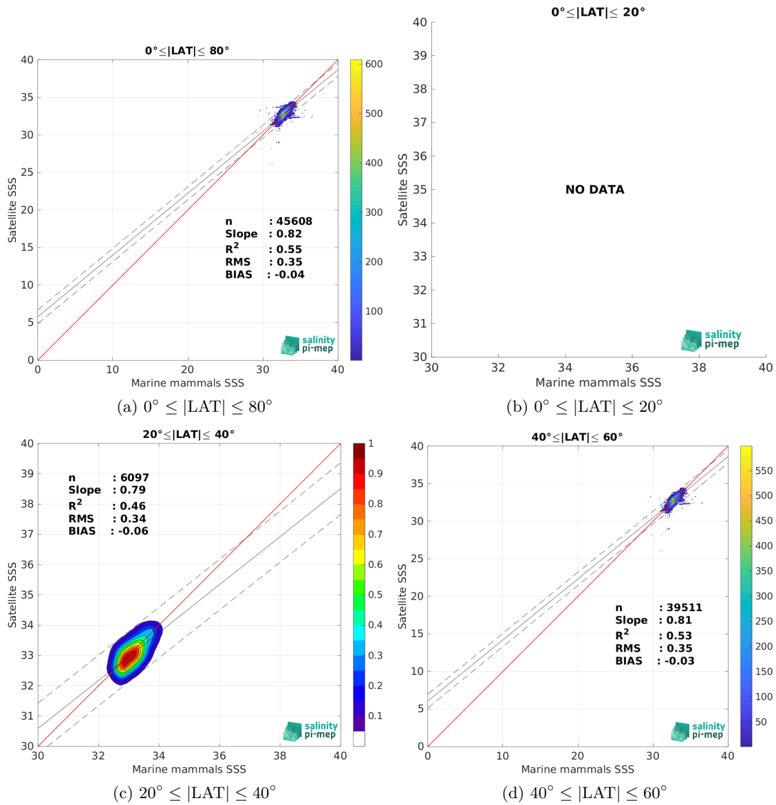
Figure 10: Contour maps of the concentration of SMOS SSS L3 v9 - 9 Days (CATDS-CEC-LOCEAN) SSS (y-axis) versus Marine mammals SSS (x-axis) at match-up pairs for different latitude bands. For each plot, the red line shows x=y . The black thin and dashed lines indicate a linear fit through the data cloud and the \pm 95\% confidence levels, respectively. The number match-up pairs n , the slope and R^2 coefficient of the linear fit, the root mean square (RMS) and the mean bias between satellite and in situ data are indicated for each latitude band in each plots.
