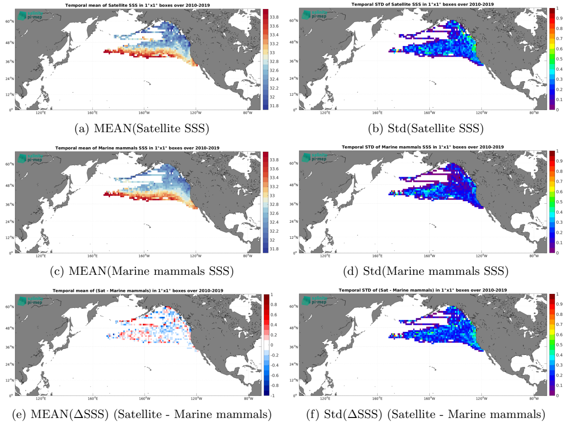
Figure 6: Temporal mean (left) and Std (right) of SSS from SMOS SSS L3 v9 - 9 Days (CATDS-CEC-LOCEAN) (top), Marine mammals (middle), and of \Delta SSS (Satellite - Marine mammals). Only match-up pairs are used to generate these maps.
