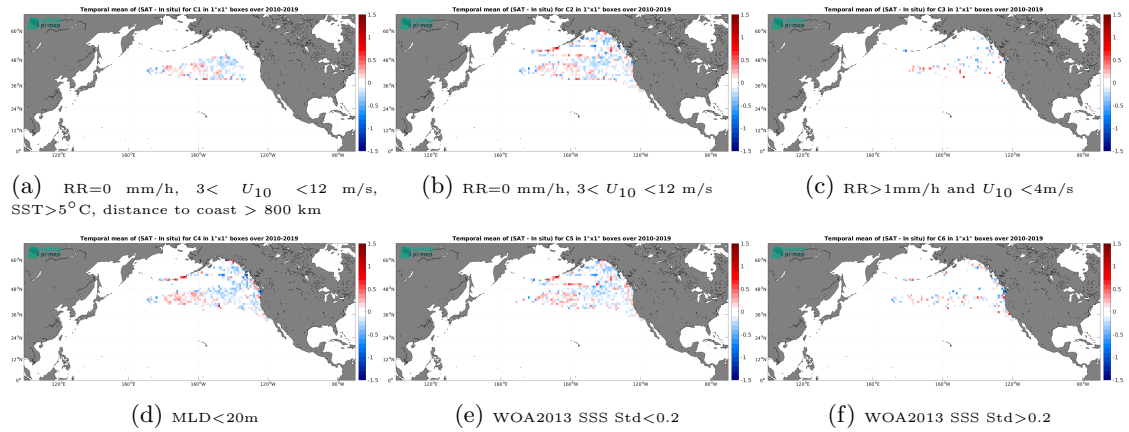
Figure 12: Temporal mean gridded over spatial boxes of size 1^{\circ}\times 1^{\circ} of \Delta\text{SSS} (SMOS SSS L3 v9 - 9 Days (CATDS-CEC-LOCEAN) - Marine mammals) for 6 different subdatasets corresponding to:RR=0 mm/h, 3 < U_{10} < 12 m/s, \text{SST} > 5^{\circ}\text{C} , distance to coast > 800 km (a), RR=0 mm/h, 3 < U_{10} < 12 m/s (b), RR > 1\text{mm/h} and U_{10} < 4\text{m/s} (c),MLD < 20\text{m} (d),WOA2013 SSS Std < 0.2 (e),WOA2013 SSS Std > 0.2 (f).
