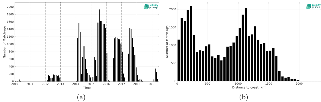
Figure 1: Number of match-ups between Marine mammals and SMOS SSS L3 v9 - 9 Days (CATDS-CEC-LOCEAN) SSS as a function of time (a) and as function of the distance to coast (b) over the North Pacific Ocean Pi-MEP region and for the full satellite product period.
