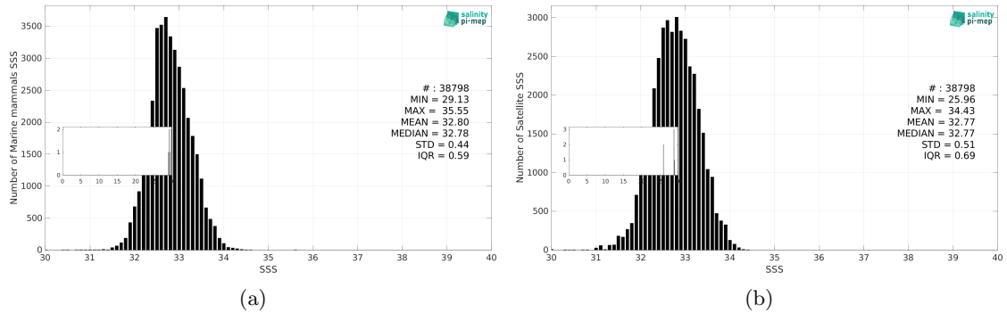
Figure 2: Histograms of SSS from Marine mammals (a) and SMOS SSS L3 v9 - 9 Days (CATDS-CEC-LOCEAN) (b) considering all match-up pairs per bins of 0.1 over the North Pacific Ocean Pi-MEP region and for the full satellite product period.
