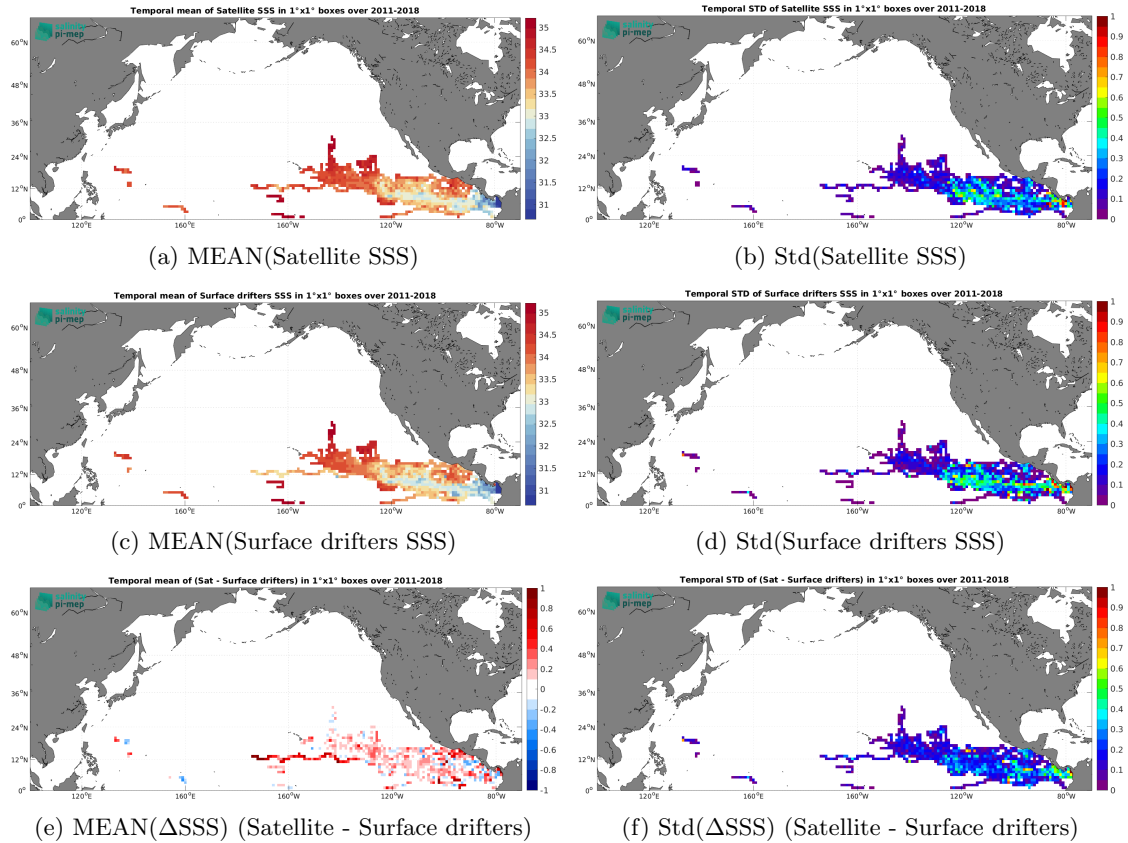
Figure 6: Temporal mean (left) and Std (right) of SSS from SMOS SSS L3 v9 - 9 Days (CATDS-CEC-LOCEAN) (top), Surface drifters (middle), and of \Delta SSS (Satellite - Surface drifters). Only match-up pairs are used to generate these maps.
