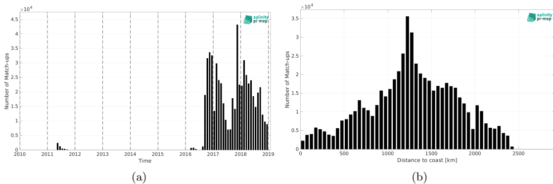
Figure 2: Number of match-ups between Surface drifters and SMOS SSS L3 v9 - 9 Days (CATDS-CEC-LOCEAN) SSS as a function of time (a) and as function of the distance to coast (b) over the North Pacific Ocean Pi-MEP region and for the full satellite product period.
