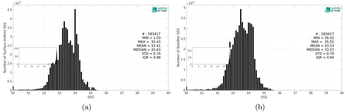
Figure 3: Histograms of SSS from Surface drifters (a) and SMOS SSS L3 v9 - 9 Days (CATDS-CEC-LOCEAN) (b) considering all match-up pairs per bins of 0.1 over the North Pacific Ocean Pi-MEP region and for the full satellite product period.
