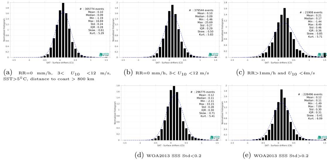
Figure 12: Normalized histogram of \Delta SSS (SMOS SSS L3 v9 - 9 Days (CATDS-CEC-LOCEAN) - Surface drifters) for 5 different subdatasets corresponding to: RR=0 mm/h, 3 < U_{10} < 12 m/s, SST>5°C, distance to coast > 800 km (a), RR=0 mm/h, 3 < U_{10} < 12 m/s (b), RR>1mm/h and U_{10} < 4 m/s (c), WOA2013 SSS Std<0.2 (d), WOA2013 SSS Std>0.2 (e).
