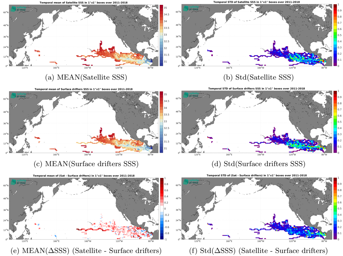
Figure 5: Temporal mean (left) and Std (right) of SSS from SMOS SSS L3 v9 - 9 Days (CATDS-CEC-LOCEAN) (top), Surface drifters (middle), and of \Delta SSS (Satellite - Surface drifters). Only match-up pairs are used to generate these maps.
