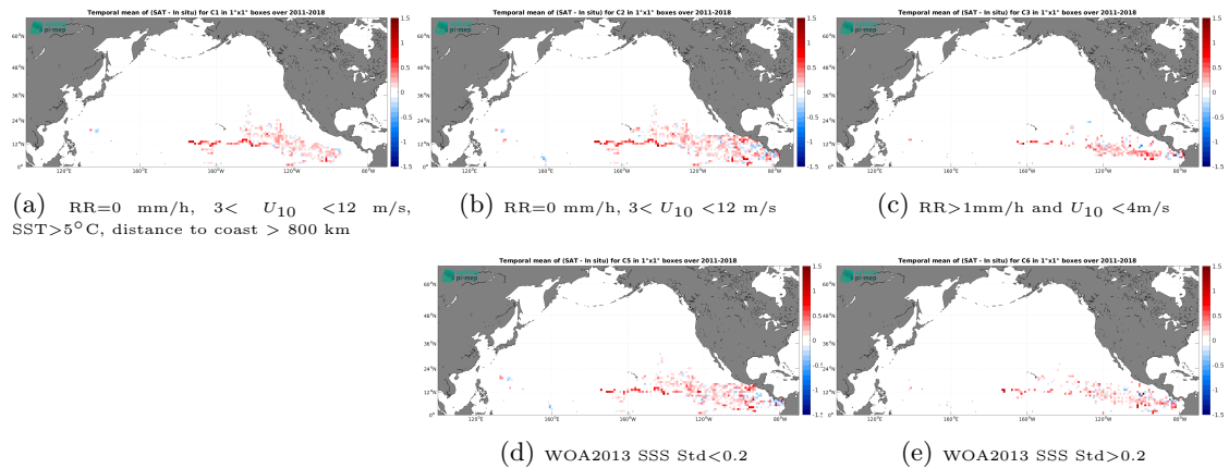
Figure 11: Temporal mean gridded over spatial boxes of size 1^\circ \times 1^\circ of \Delta SSS (SMOS SSS L3 v9 - 9 Days (CATDS-CEC-LOCEAN) - Surface drifters) for 5 different subdatasets corresponding to:RR=0 mm/h, 3 < U_{10} < 12 m/s, SST >5^\circ C, distance to coast > 800 km (a), RR=0 mm/h, 3 < U_{10} < 12 m/s (b), RR >1 mm/h and U_{10} < 4 m/s (c), WOA2013 SSS Std <0.2 (d), WOA2013 SSS Std >0.2 (e).
