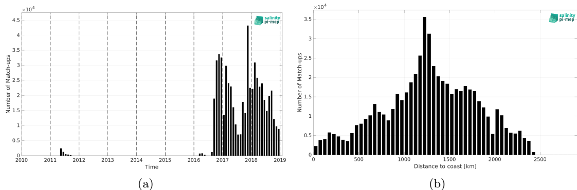
Figure 1: Number of match-ups between Surface drifters and SMOS SSS L3 v9 - 9 Days (CATDS-CEC-LOCEAN) SSS as a function of time (a) and as function of the distance to coast (b) over the North Pacific Ocean Pi-MEP region and for the full satellite product period.
