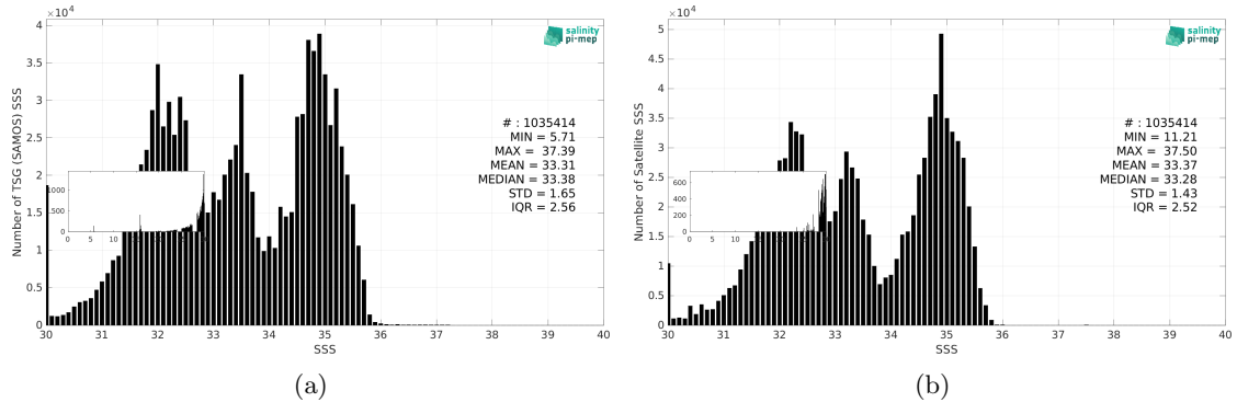
Figure 3: Histograms of SSS from TSG (SAMOS) (a) and SMOS SSS L3 v9 - 18 Days (CATDS-CEC-LOCEAN) (b) considering all match-up pairs per bins of 0.1 over the North Pacific Ocean Pi-MEP region and for the full satellite product period.
