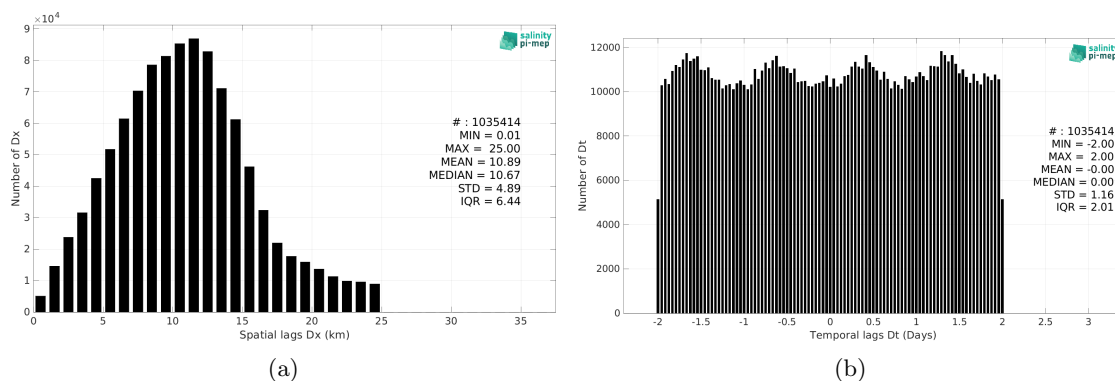
Figure 6: Histograms of the spatial (a) and temporal (b) lags between the location/time of the TSG (SAMOS) measurement and the date of the corresponding SMOS SSS L3 v9 - 18 Days (CATDS-CEC-LOCEAN) SSS pixel.
