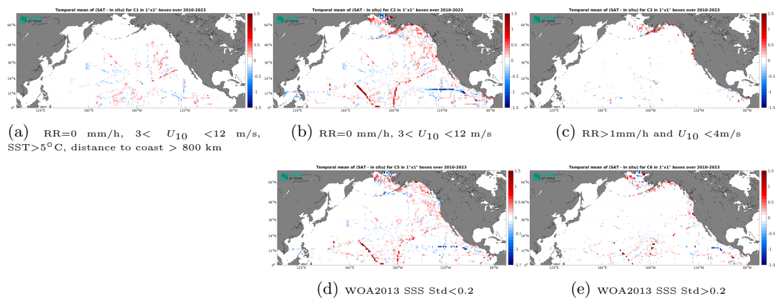
Figure 14: Temporal mean gridded over spatial boxes of size 1^\circ \times 1^\circ of \Delta SSS (SMOS SSS L3 v9 - 18 Days (CATDS-CEC-LOCEAN) - TSG (SAMOS)) for 5 different subdatasets corresponding to: RR=0 mm/h, 3 < U_{10} < 12 m/s, SST > 5°C, distance to coast > 800 km (a), RR=0 mm/h, 3 < U_{10} < 12 m/s (b), RR > 1 mm/h and U_{10} < 4 m/s (c), WOA2013 SSS Std < 0.2 (d), WOA2013 SSS Std > 0.2 (e).
