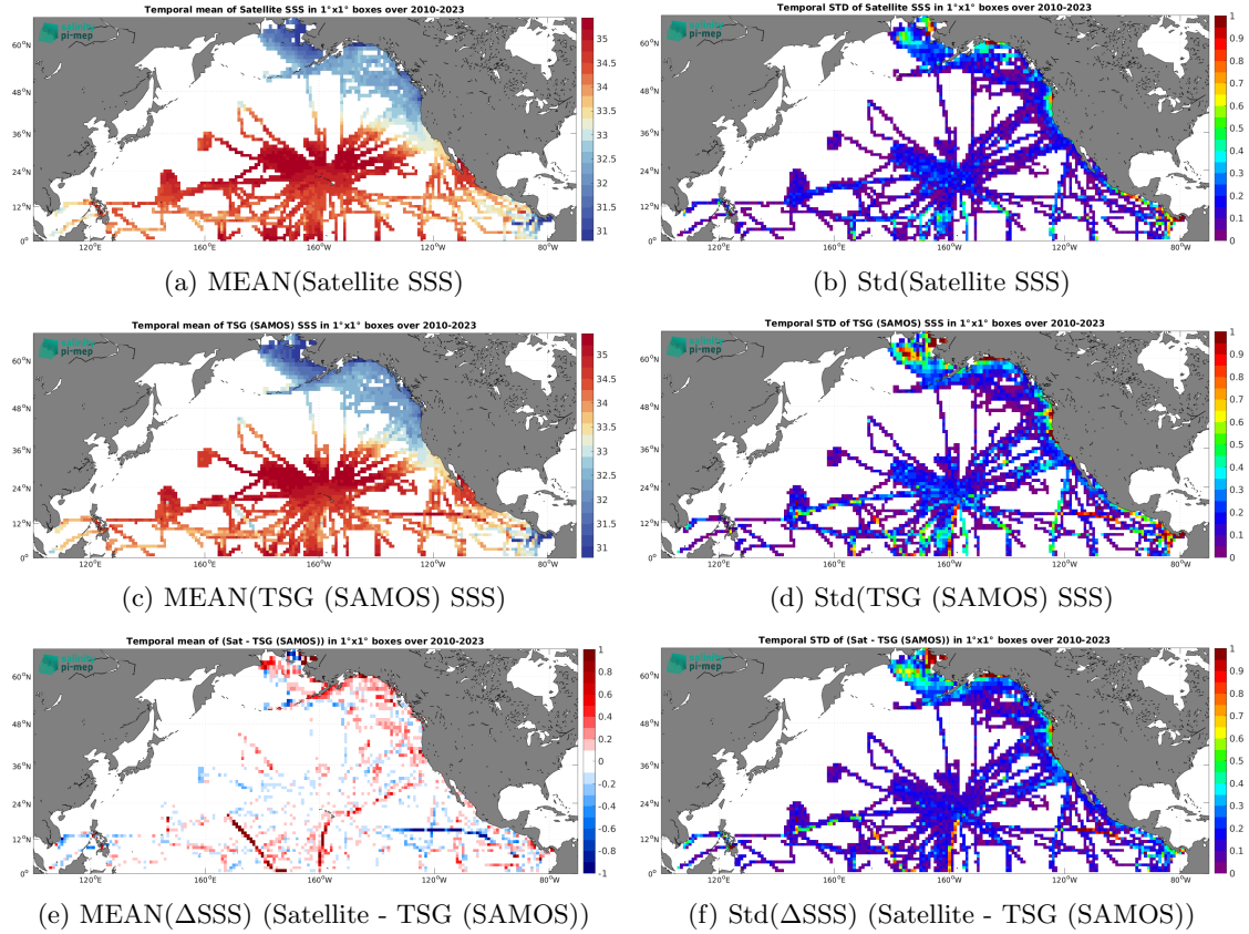
Figure 7: Temporal mean (left) and Std (right) of SSS from SMOS SSS L3 v9 - 18 Days (CATDS-CEC-LOCEAN) (top), TSG (SAMOS) (middle), and of \Delta\text{SSS} (Satellite - TSG (SAMOS)). Only match-up pairs are used to generate these maps.
