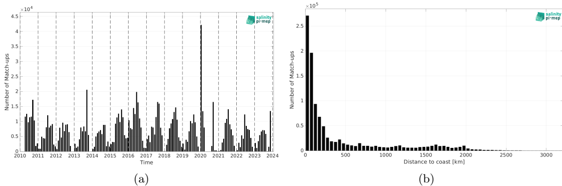
Figure 2: Number of match-ups between TSG (SAMOS) and SMOS SSS L3 v9 - 18 Days (CATDS-CEC-LOCEAN) SSS as a function of time (a) and as function of the distance to coast (b) over the North Pacific Ocean Pi-MEP region and for the full satellite product period.
