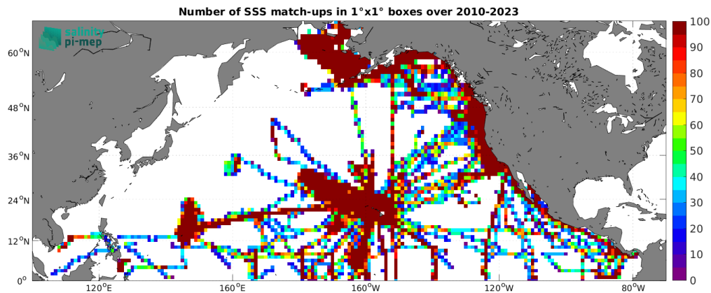
Figure 5: Number of SSS match-ups between TSG (SAMOS) SSS and the SMOS SSS L3 v9 - 18 Days (CATDS-CEC-LOCEAN) SSS product for the North Pacific Ocean Pi-MEP region over 1^\circ \times 1^\circ boxes and for the full satellite product period.
