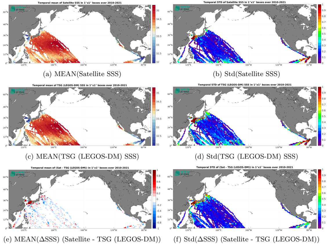
Figure 6: Temporal mean (left) and Std (right) of SSS from SMOS SSS L3 v9 - 18 Days (CATDS-CEC-LOCEAN) (top), TSG (LEGOS-DM) (middle), and of \Delta\text{SSS} (Satellite - TSG (LEGOS-DM)). Only match-up pairs are used to generate these maps.
