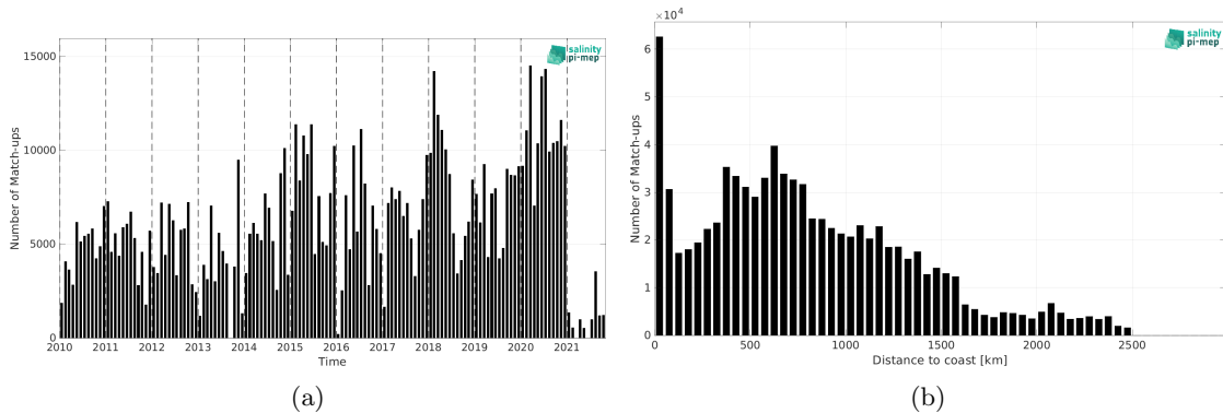
Figure 1: Number of match-ups between TSG (LEGOS-DM) and SMOS SSS L3 v9 - 18 Days (CATDS-CEC-LOCEAN) SSS as a function of time (a) and as function of the distance to coast (b) over the North Pacific Ocean Pi-MEP region and for the full satellite product period.
