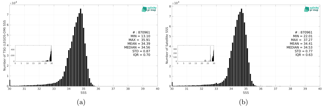
Figure 2: Histograms of SSS from TSG (LEGOS-DM) (a) and SMOS SSS L3 v9 - 18 Days (CATDS-CEC-LOCEAN) (b) considering all match-up pairs per bins of 0.1 over the North Pacific Ocean Pi-MEP region and for the full satellite product period.
