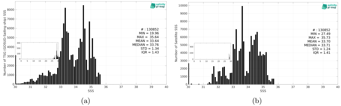
Figure 3: Histograms of SSS from TSG (GOSUD-Sailing-ship) (a) and SMOS SSS L3 v9 - 18 Days (CATDS-CEC-LOCEAN) (b) considering all match-up pairs per bins of 0.1 over the North Pacific Ocean Pi-MEP region and for the full satellite product period.
