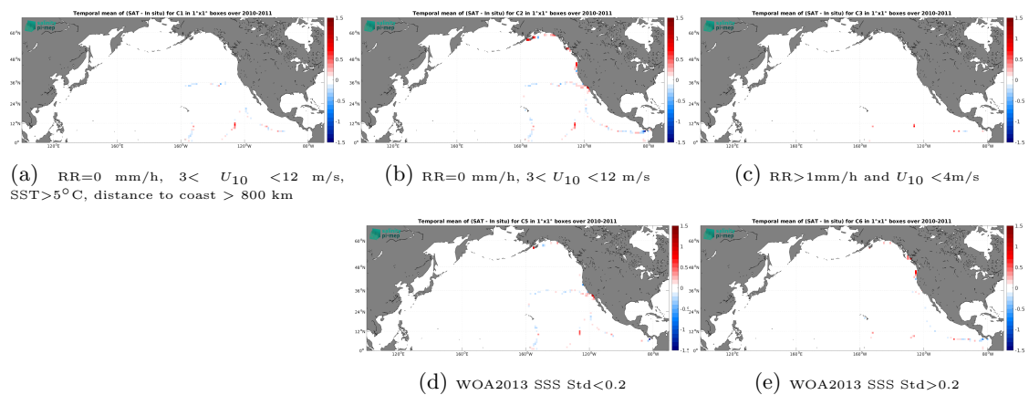
Figure 14: Temporal mean gridded over spatial boxes of size 1^\circ \times 1^\circ of \Delta\text{SSS} (SMOS SSS L3 v9 - 18 Days (CATDS-CEC-LOCEAN) - TSG (GOSUD-Sailing-ship)) for 5 different subdatasets corresponding to: RR=0 mm/h, 3 < U_{10} < 12 m/s, SST > 5°C, distance to coast > 800 km (a), RR=0 mm/h, 3 < U_{10} < 12 m/s (b), RR > 1 mm/h and U_{10} < 4 m/s (c), WOA2013 SSS Std < 0.2 (d), WOA2013 SSS Std > 0.2 (e).
