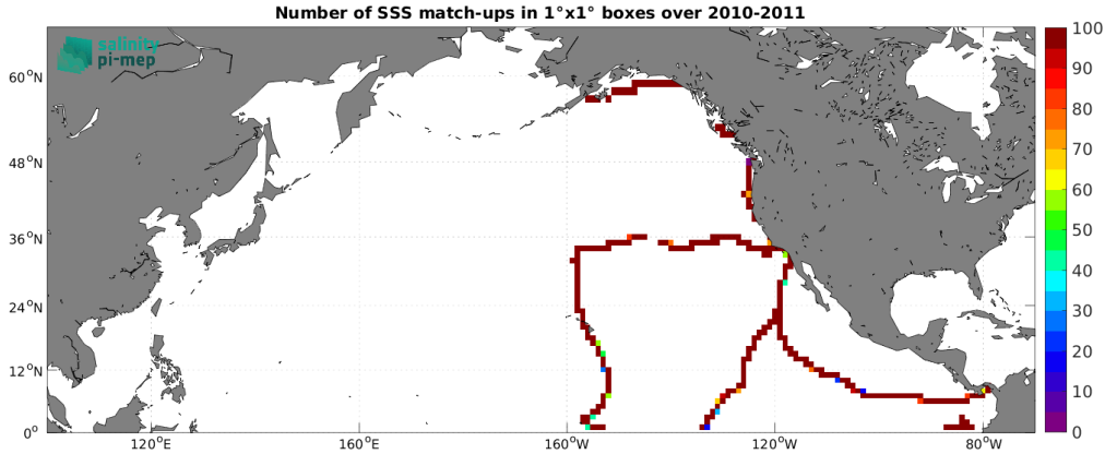
Figure 4: Number of SSS match-ups between TSG (GOSUD-Sailing-ship) SSS and the SMOS SSS L3 v9 - 18 Days (CATDS-CEC-LOCEAN) SSS product for the North Pacific Ocean Pi-MEP region over 1^\circ \times 1^\circ boxes and for the full satellite product period.
