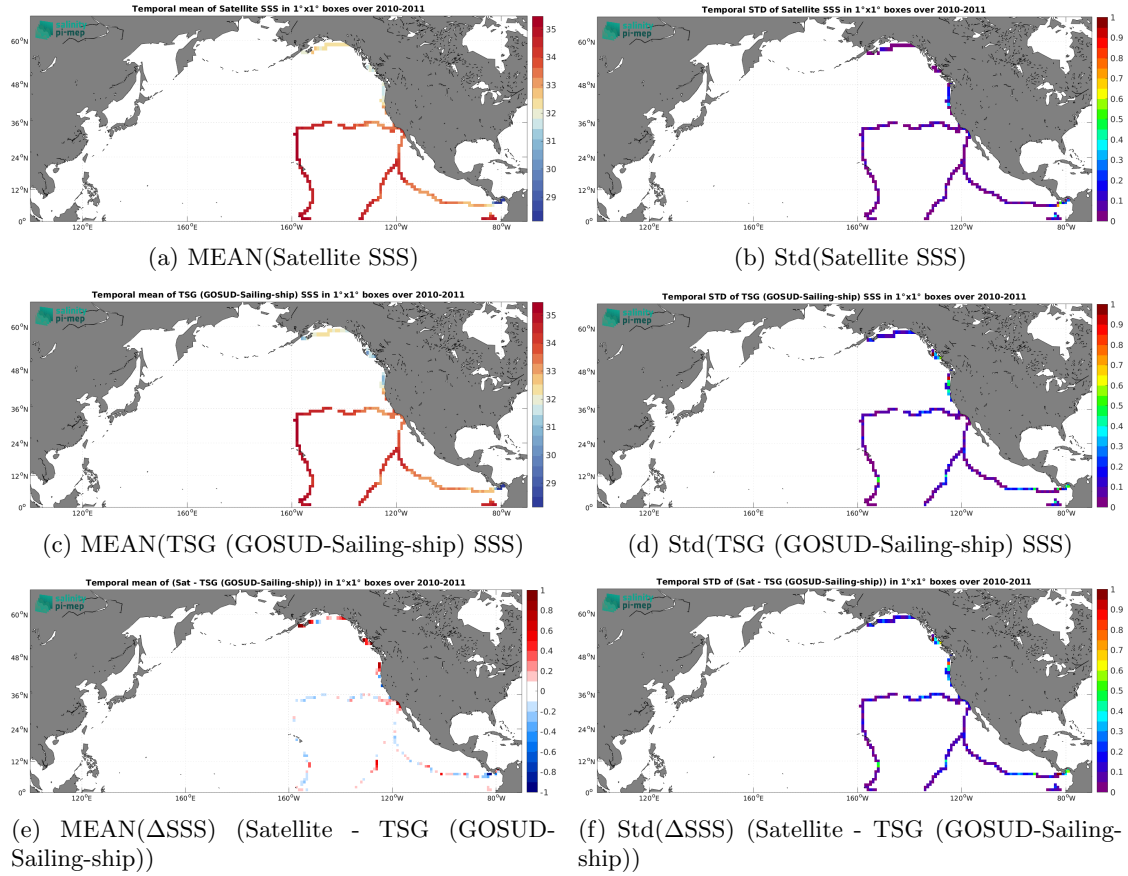
Figure 6: Temporal mean (left) and Std (right) of SSS from SMOS SSS L3 v9 - 18 Days (CATDS-CEC-LOCEAN) (top), TSG (GOSUD-Sailing-ship) (middle), and of \Delta SSS (Satellite - TSG (GOSUD-Sailing-ship)). Only match-up pairs are used to generate these maps.
