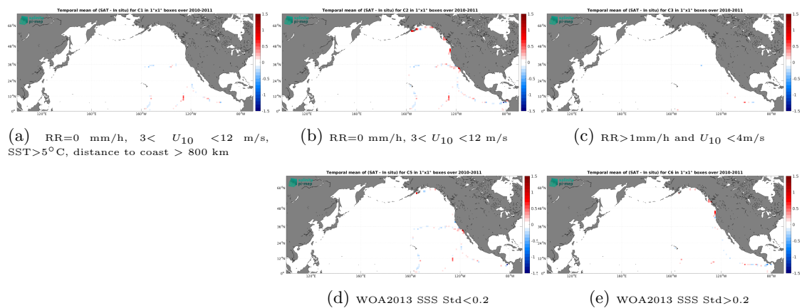
Figure 12: Temporal mean gridded over spatial boxes of size 1^\circ \times 1^\circ of \Delta SSS (SMOS SSS L3 v9 - 18 Days (CATDS-CEC-LOCEAN) - TSG (GOSUD-Sailing-ship)) for 5 different subdatasets corresponding to: RR=0 mm/h, 3 < U_{10} < 12 m/s, SST > 5°C, distance to coast > 800 km (a), RR=0 mm/h, 3 < U_{10} < 12 m/s (b), RR > 1mm/h and U_{10} < 4 m/s (c), WOA2013 SSS Std < 0.2 (d), WOA2013 SSS Std > 0.2 (e).
