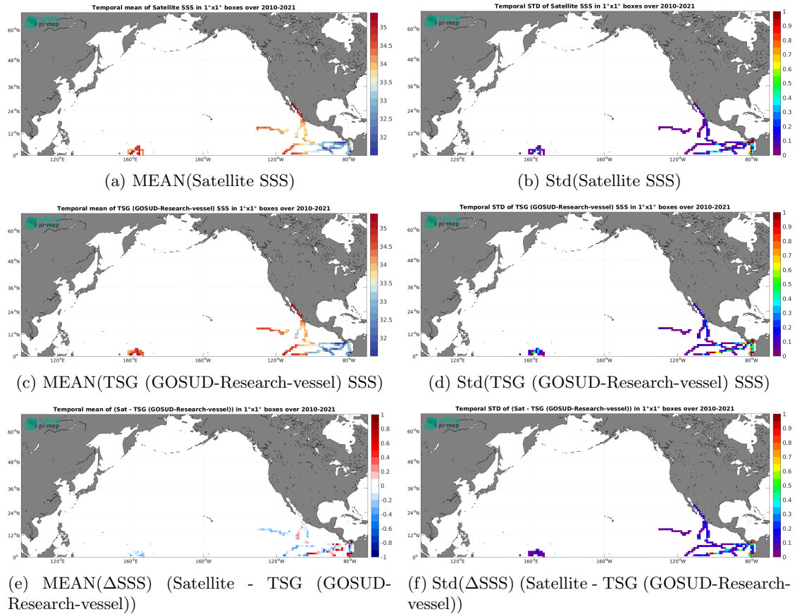
Figure 7: Temporal mean (left) and Std (right) of SSS from SMOS SSS L3 v9 - 18 Days (CATDS-CEC-LOCEAN) (top), TSG (GOSUD-Research-vessel) (middle), and of \Delta SSS (Satellite - TSG (GOSUD-Research-vessel)). Only match-up pairs are used to generate these maps.
