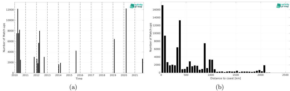
Figure 2: Number of match-ups between TSG (GOSUD-Research-vessel) and SMOS SSS L3 v9 - 18 Days (CATDS-CEC-LOCEAN) SSS as a function of time (a) and as function of the distance to coast (b) over the North Pacific Ocean Pi-MEP region and for the full satellite product period.
