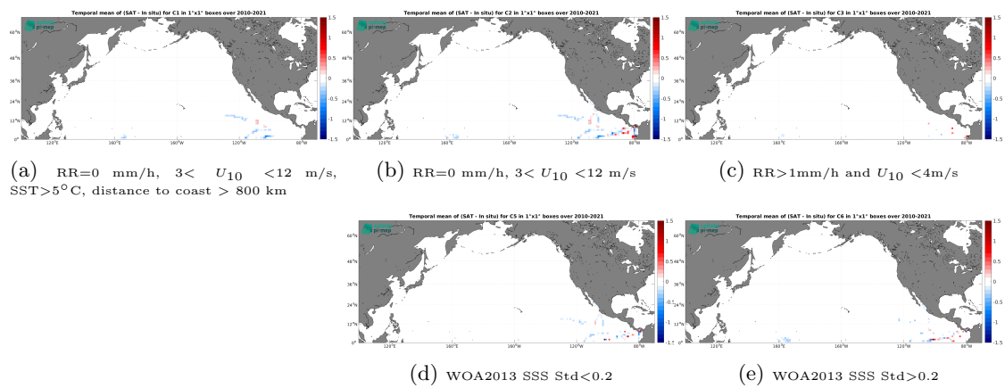
Figure 14: Temporal mean gridded over spatial boxes of size 1^\circ \times 1^\circ of \Delta\text{SSS} (SMOS SSS L3 v9 - 18 Days (CATDS-CEC-LOCEAN) - TSG (GOSUD-Research-vessel)) for 5 different subdatasets corresponding to: RR=0 mm/h, 3 < U_{10} < 12 m/s, SST > 5°C, distance to coast > 800 km (a), RR=0 mm/h, 3 < U_{10} < 12 m/s (b), RR > 1 mm/h and U_{10} < 4 m/s (c), WOA2013 SSS Std < 0.2 (d), WOA2013 SSS Std > 0.2 (e).
