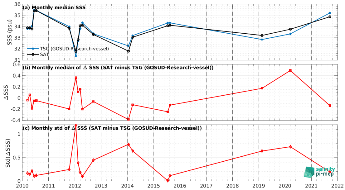
Figure 8: Time series of the monthly median SSS (top), median of \Delta SSS (Satellite - TSG (GOSUD-Research-vessel)) and Std of \Delta SSS (Satellite - TSG (GOSUD-Research-vessel)) over the North Pacific Ocean Pi-MEP region considering all match-ups collected by the Pi-MEP.
