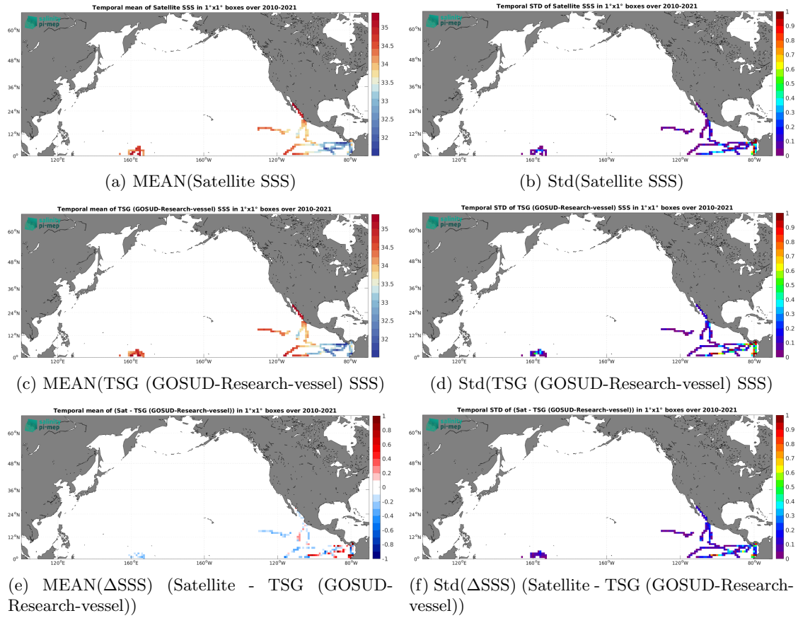
Figure 6: Temporal mean (left) and Std (right) of SSS from SMOS SSS L3 v9 - 18 Days (CATDS-CEC-LOCEAN) (top), TSG (GOSUD-Research-vessel) (middle), and of \Delta SSS (Satellite - TSG (GOSUD-Research-vessel)). Only match-up pairs are used to generate these maps.
