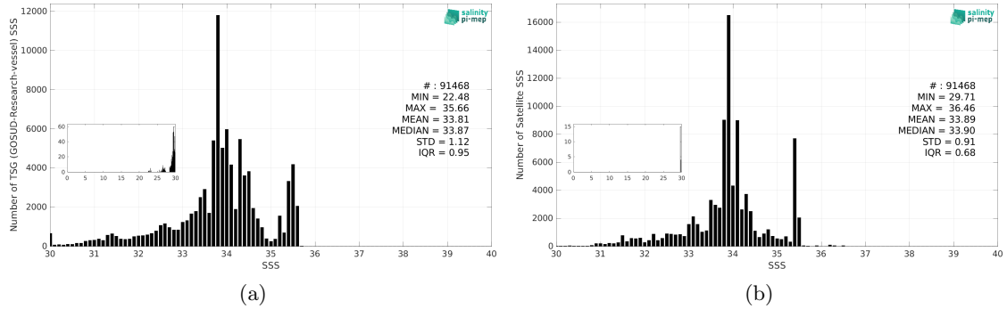
Figure 2: Histograms of SSS from TSG (GOSUD-Research-vessel) (a) and SMOS SSS L3 v9 - 18 Days (CATDS-CEC-LOCEAN) (b) considering all match-up pairs per bins of 0.1 over the North Pacific Ocean Pi-MEP region and for the full satellite product period.
