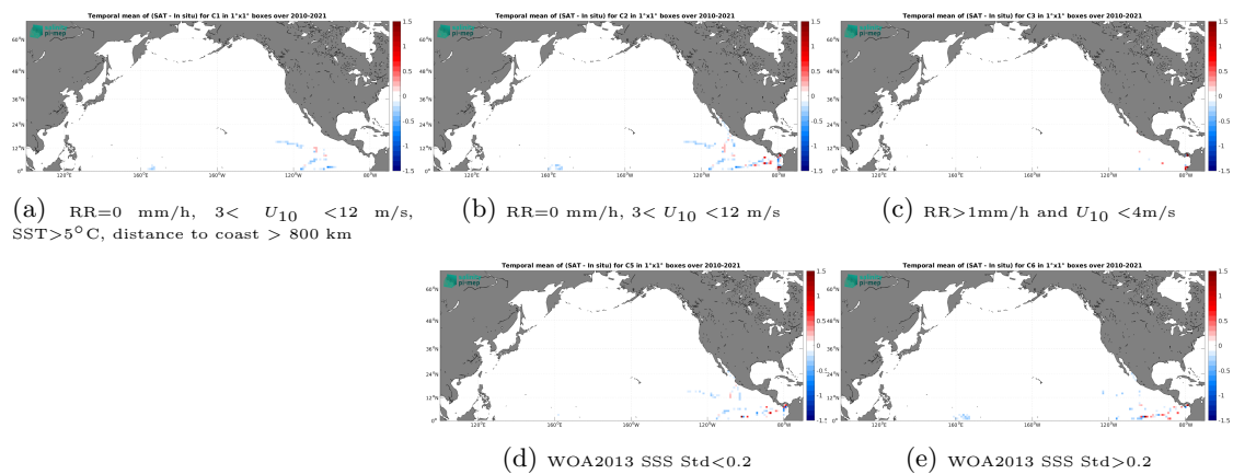
Figure 12: Temporal mean gridded over spatial boxes of size 1^\circ \times 1^\circ of \Delta\text{SSS} (SMOS SSS L3 v9 - 18 Days (CATDS-CEC-LOCEAN) - TSG (GOSUD-Research-vessel)) for 5 different subdatasets corresponding to:RR=0 mm/h, 3 < U_{10} < 12 m/s, SST>5°C, distance to coast > 800 km (a), RR=0 mm/h, 3 < U_{10} < 12 m/s (b), RR>1mm/h and U_{10} < 4 m/s (c), WOA2013 SSS Std<0.2 (d), WOA2013 SSS Std>0.2 (e).
