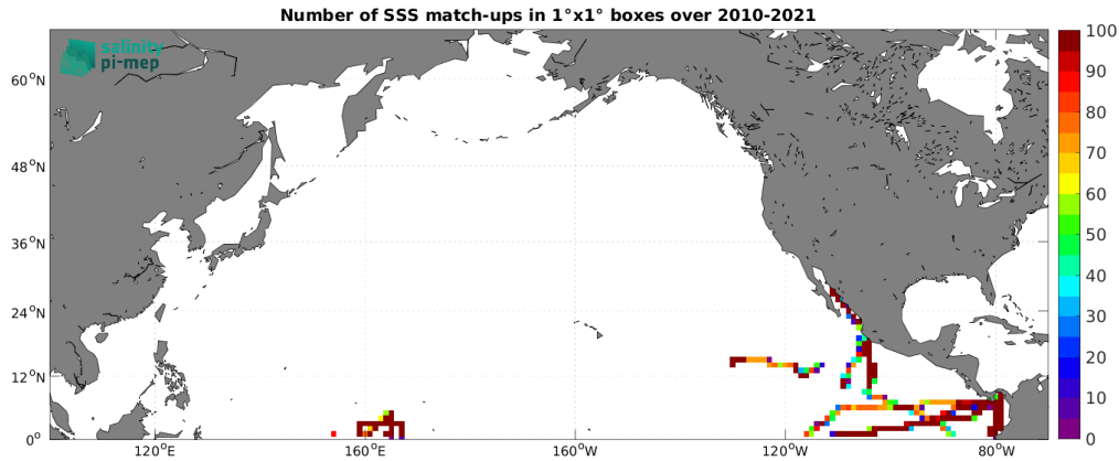
Figure 4: Number of SSS match-ups between TSG (GOSUD-Research-vessel) SSS and the SMOS SSS L3 v9 - 18 Days (CATDS-CEC-LOCEAN) SSS product for the North Pacific Ocean Pi-MEP region over 1^\circ \times 1^\circ boxes and for the full satellite product period.
