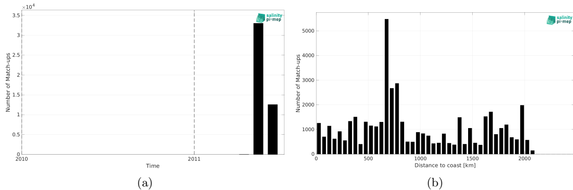
Figure 1: Number of match-ups between TSG (CSIC-UTM) and SMOS SSS L3 v9 - 18 Days (CATDS-CEC-LOCEAN) SSS as a function of time (a) and as function of the distance to coast (b) over the North Pacific Ocean Pi-MEP region and for the full satellite product period.
