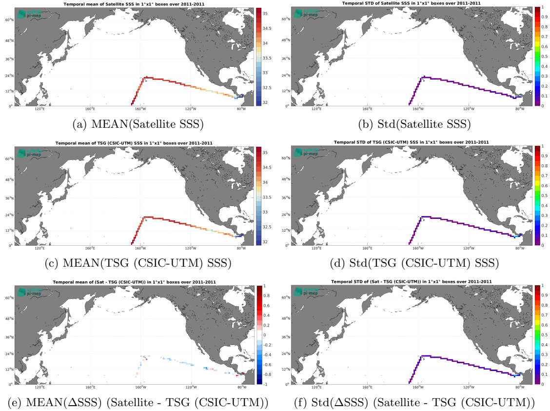
Figure 6: Temporal mean (left) and Std (right) of SSS from SMOS SSS L3 v9 - 18 Days (CATDS-CEC-LOCEAN) (top), TSG (CSIC-UTM) (middle), and of \Delta\text{SSS} (Satellite - TSG (CSIC-UTM)). Only match-up pairs are used to generate these maps.
