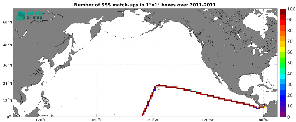
Figure 4: Number of SSS match-ups between TSG (CSIC-UTM) SSS and the SMOS SSS L3 v9 - 18 Days (CATDS-CEC-LOCEAN) SSS product for the North Pacific Ocean Pi-MEP region over 1^\circ \times 1^\circ boxes and for the full satellite product period.
