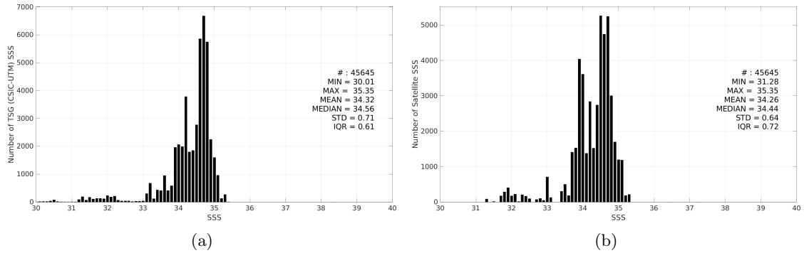
Figure 2: Histograms of SSS from TSG (CSIC-UTM) (a) and SMOS SSS L3 v9 - 18 Days (CATDS-CEC-LOCEAN) (b) considering all match-up pairs per bins of 0.1 over the North Pacific Ocean Pi-MEP region and for the full satellite product period.
