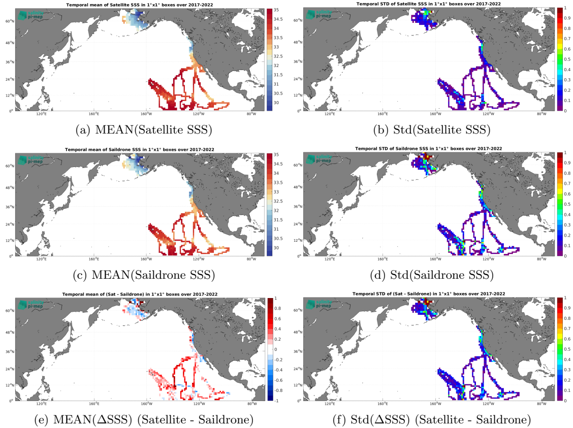
Figure 6: Temporal mean (left) and Std (right) of SSS from SMOS SSS L3 v9 - 18 Days (CATDS-CEC-LOCEAN) (top), Saildrone (middle), and of \Delta SSS (Satellite - Saildrone). Only match-up pairs are used to generate these maps.
