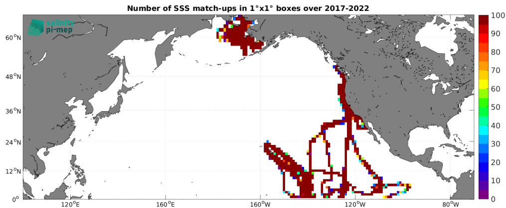
Figure 4: Number of SSS match-ups between Saildrone SSS and the SMOS SSS L3 v9 - 18 Days (CATDS-CEC-LOCEAN) SSS product for the North Pacific Ocean Pi-MEP region over 1^\circ \times 1^\circ boxes and for the full satellite product period.
