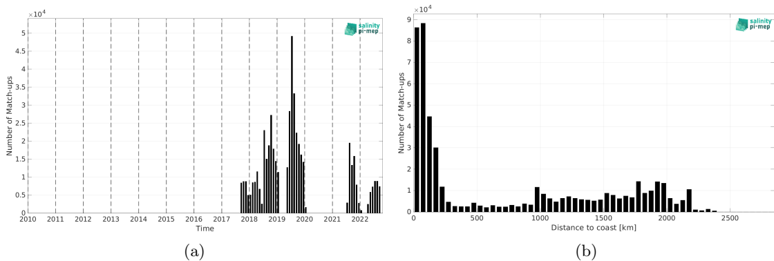
Figure 1: Number of match-ups between Saildrone and SMOS SSS L3 v9 - 18 Days (CATDS-CEC-LOCEAN) SSS as a function of time (a) and as function of the distance to coast (b) over the North Pacific Ocean Pi-MEP region and for the full satellite product period.
