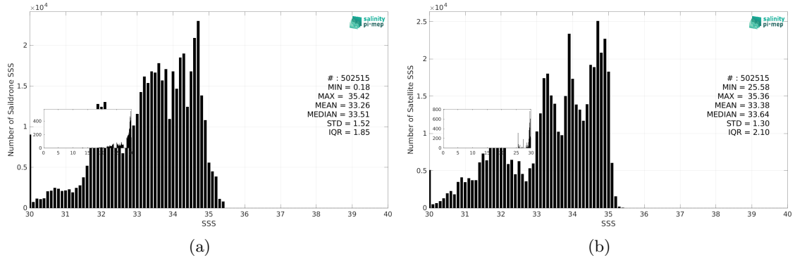
Figure 2: Histograms of SSS from Saildrone (a) and SMOS SSS L3 v9 - 18 Days (CATDS-CEC-LOCEAN) (b) considering all match-up pairs per bins of 0.1 over the North Pacific Ocean Pi-MEP region and for the full satellite product period.
