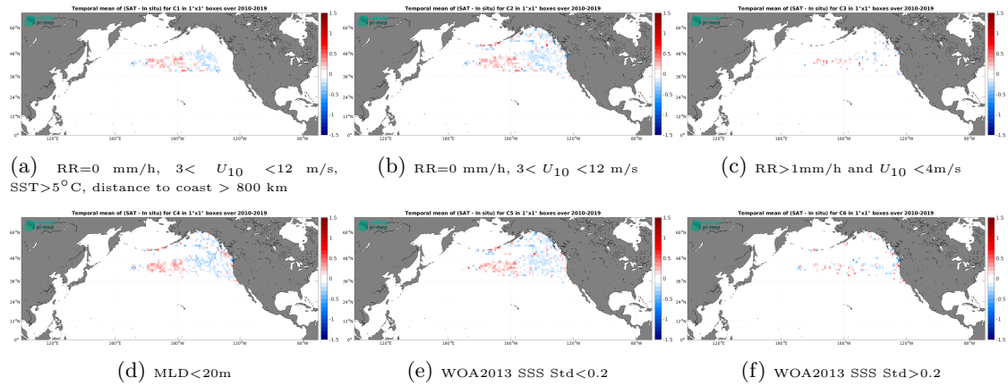
Figure 12: Temporal mean gridded over spatial boxes of size 1^{\circ}\times 1^{\circ} of \Delta\text{SSS} (SMOS SSS L3 v9 - 18 Days (CATDS-CEC-LOCEAN) - Marine mammals) for 6 different subdatasets corresponding to:RR=0 mm/h, 3 < U_{10} < 12 m/s, \text{SST} > 5^{\circ}\text{C} , distance to coast > 800 km (a), RR=0 mm/h, 3 < U_{10} < 12 m/s (b), RR > 1\text{mm/h} and U_{10} < 4\text{m/s} (c),MLD < 20\text{m} (d),WOA2013 SSS Std < 0.2 (e),WOA2013 SSS Std > 0.2 (f).
