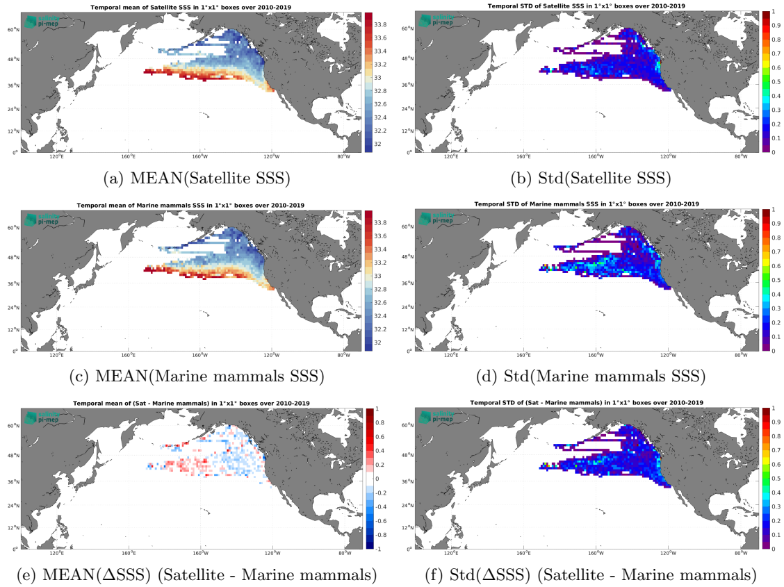
Figure 6: Temporal mean (left) and Std (right) of SSS from SMOS SSS L3 v9 - 18 Days (CATDS-CEC-LOCEAN) (top), Marine mammals (middle), and of \Delta SSS (Satellite - Marine mammals). Only match-up pairs are used to generate these maps.
