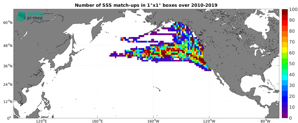
Figure 4: Number of SSS match-ups between Marine mammals SSS and the SMOS SSS L3 v9 - 18 Days (CATDS-CEC-LOCEAN) SSS product for the North Pacific Ocean Pi-MEP region over 1^\circ \times 1^\circ boxes and for the full satellite product period.
