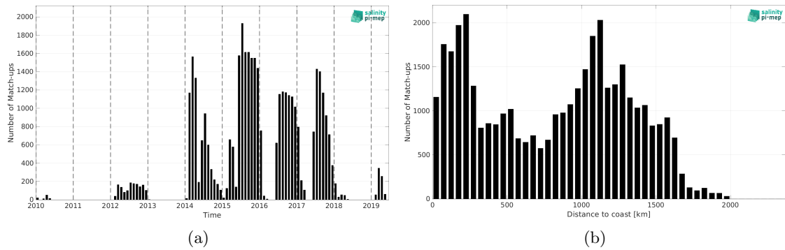
Figure 1: Number of match-ups between Marine mammals and SMOS SSS L3 v9 - 18 Days (CATDS-CEC-LOCEAN) SSS as a function of time (a) and as function of the distance to coast (b) over the North Pacific Ocean Pi-MEP region and for the full satellite product period.
