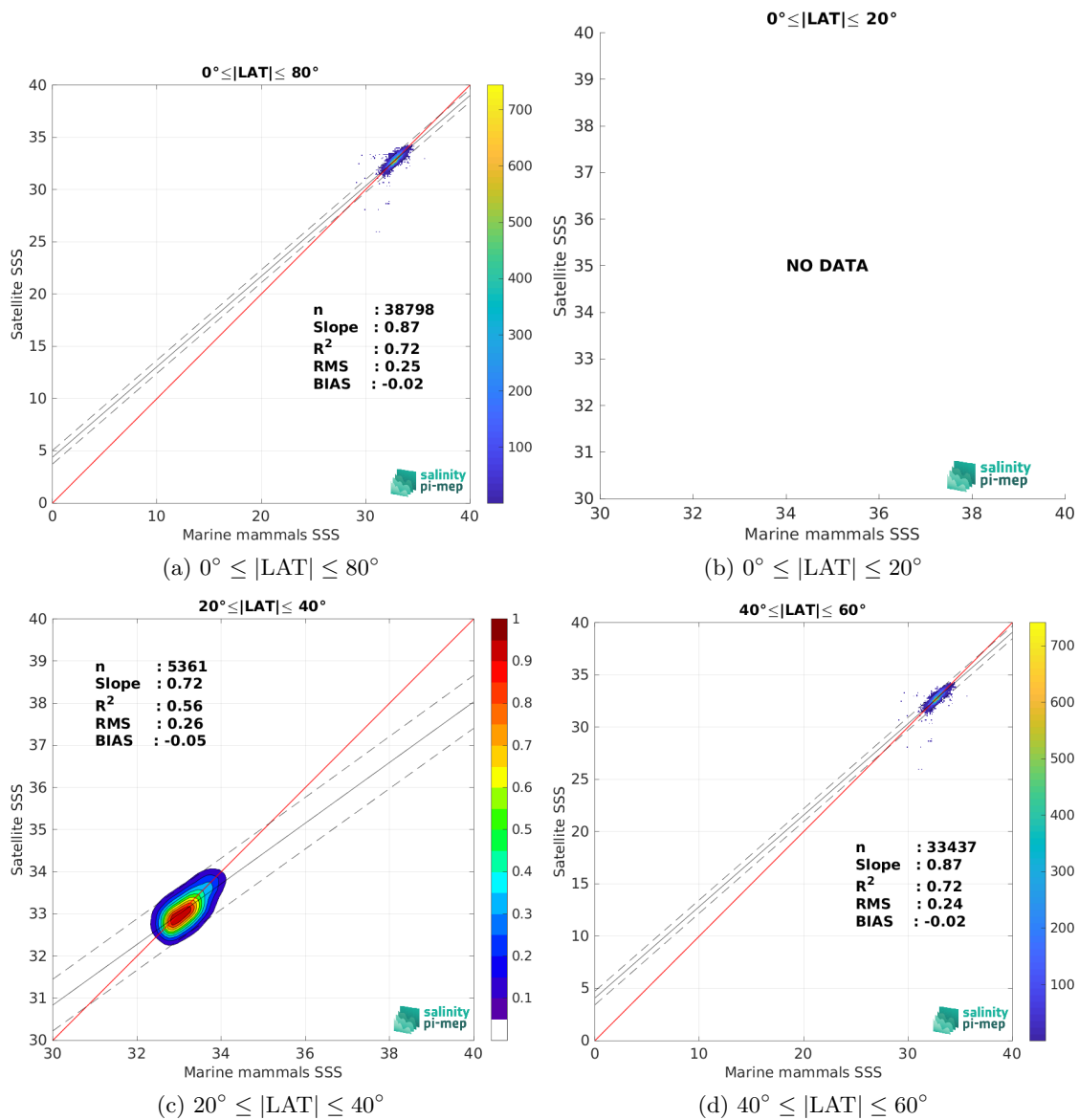
Figure 9: Contour maps of the concentration of SMOS SSS L3 v9 - 18 Days (CATDS-CEC-LOCEAN) SSS ( y -axis) versus Marine mammals SSS ( x -axis) at match-up pairs for different latitude bands. For each plot, the red line shows x=y . The black thin and dashed lines indicate a linear fit through the data cloud and the \pm 95\% confidence levels, respectively. The number match-up pairs n , the slope and R^2 coefficient of the linear fit, the root mean square (RMS) and the mean bias between satellite and in situ data are indicated for each latitude band in each plots.
