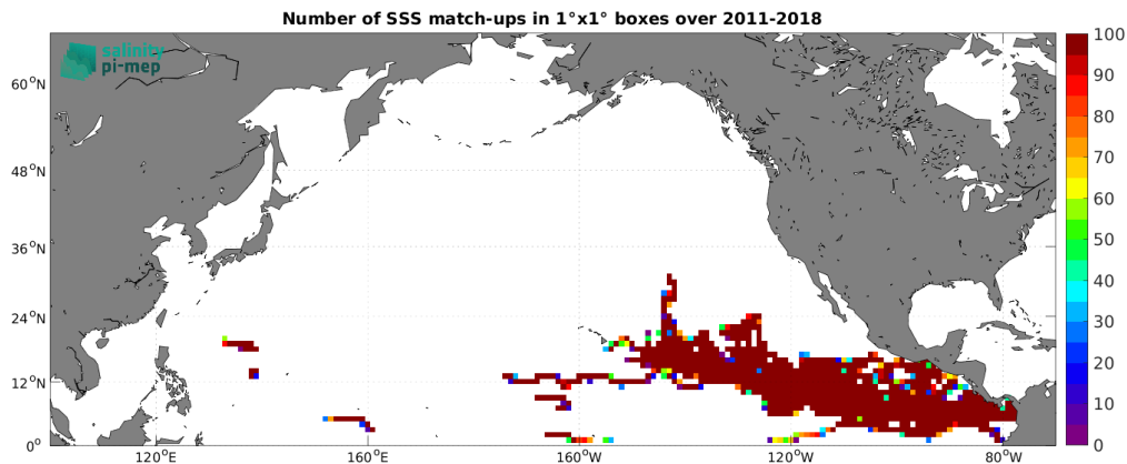
Figure 3: Number of SSS match-ups between Surface drifters SSS and the SMOS SSS L3 v9 - 18 Days (CATDS-CEC-LOCEAN) SSS product for the North Pacific Ocean Pi-MEP region over 1^\circ \times 1^\circ boxes and for the full satellite product period.
