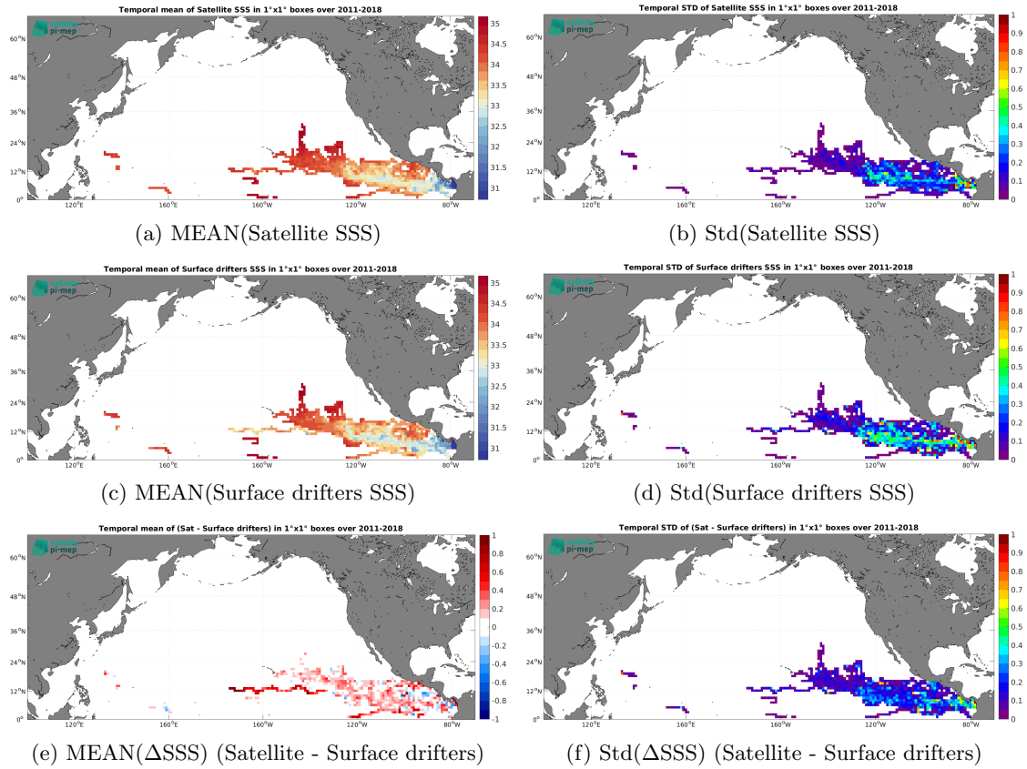
Figure 5: Temporal mean (left) and Std (right) of SSS from SMOS SSS L3 v9 - 18 Days (CATDS-CEC-LOCEAN) (top), Surface drifters (middle), and of \Delta SSS (Satellite - Surface drifters). Only match-up pairs are used to generate these maps.
