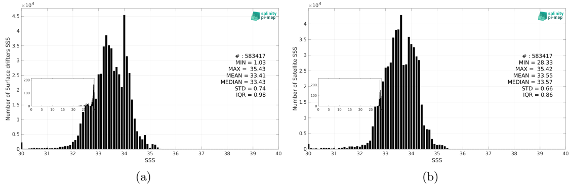
Figure 2: Histograms of SSS from Surface drifters (a) and SMOS SSS L3 v9 - 18 Days (CATDS-CEC-LOCEAN) (b) considering all match-up pairs per bins of 0.1 over the North Pacific Ocean Pi-MEP region and for the full satellite product period.
