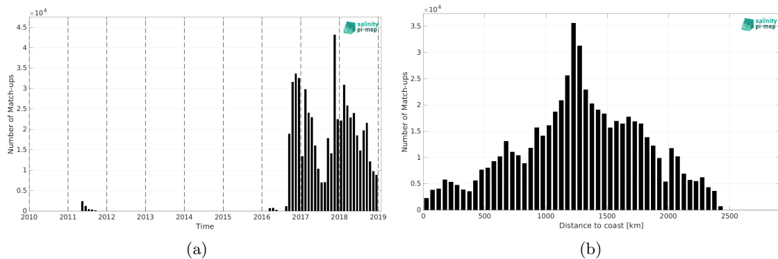
Figure 1: Number of match-ups between Surface drifters and SMOS SSS L3 v9 - 18 Days (CATDS-CEC-LOCEAN) SSS as a function of time (a) and as function of the distance to coast (b) over the North Pacific Ocean Pi-MEP region and for the full satellite product period.
