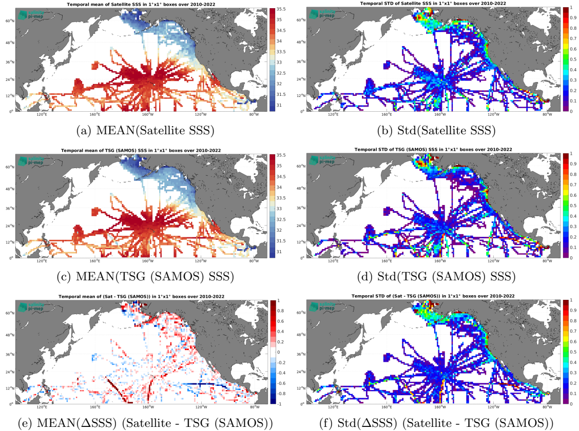
Figure 6: Temporal mean (left) and Std (right) of SSS from SMOS SSS L3 v8 - 9 Days (CATDS-CEC-LOCEAN) (top), TSG (SAMOS) (middle), and of \Delta SSS (Satellite - TSG (SAMOS)). Only match-up pairs are used to generate these maps.
