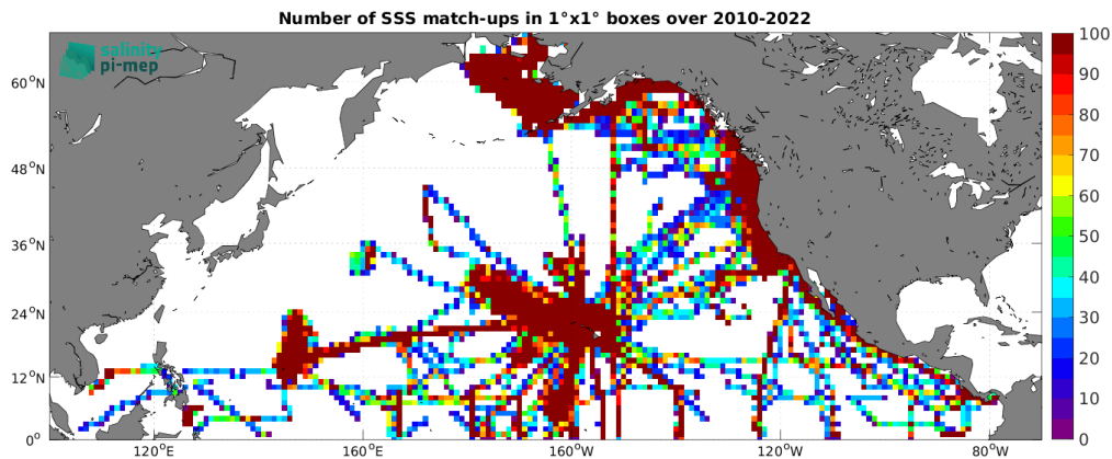
Figure 4: Number of SSS match-ups between TSG (SAMOS) SSS and the SMOS SSS L3 v8 - 9 Days (CATDS-CEC-LOCEAN) SSS product for the North Pacific Ocean Pi-MEP region over 1^\circ \times 1^\circ boxes and for the full satellite product period.
