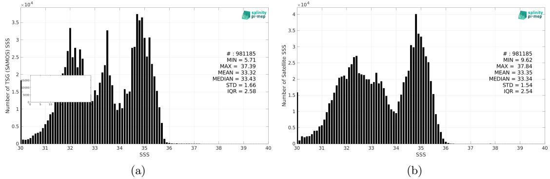
Figure 2: Histograms of SSS from TSG (SAMOS) (a) and SMOS SSS L3 v8 - 9 Days (CATDS-CEC-LOCEAN) (b) considering all match-up pairs per bins of 0.1 over the North Pacific Ocean Pi-MEP region and for the full satellite product period.
