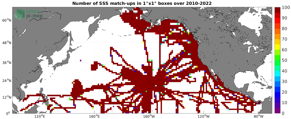
Figure 4: Number of SSS match-ups between TSG (SAMOS) SSS and the SMOS SSS L3 v8 - 9 Days (CATDS-CECOS-LOCEAN) SSS product for the North Pacific Ocean Pi-MEP region over 1^\circ \times 1^\circ boxes and for the full satellite product period.
