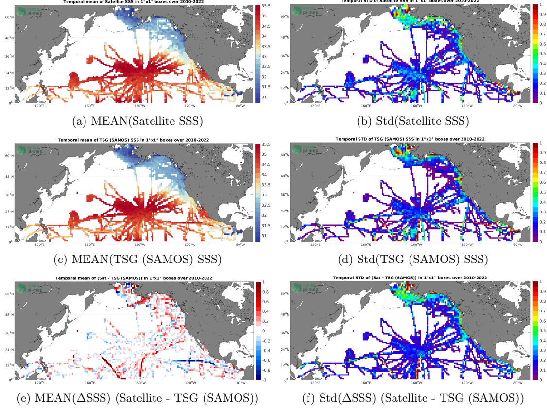
Figure 6: Temporal mean (left) and Std (right) of SSS from SMOS SSS L3 v8 - 9 Days (CATDS-CECOS-LOCEAN) (top), TSG (SAMOS) (middle), and of \Delta\text{SSS} (Satellite - TSG (SAMOS)). Only match-up pairs are used to generate these maps.
