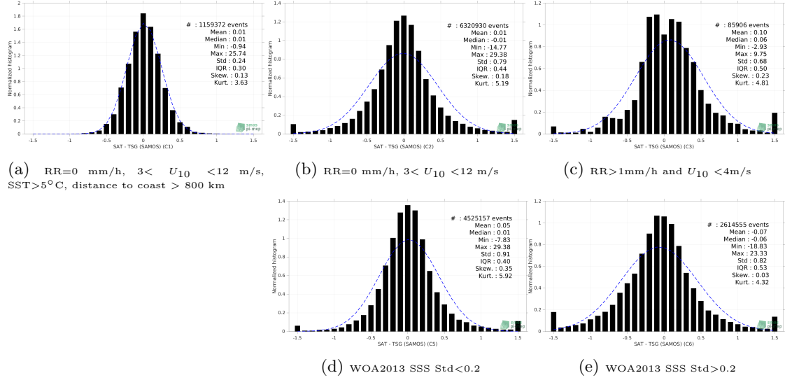
Figure 13: Normalized histogram of \Delta\text{SSS} (SMOS SSS L3 v8 - 9 Days (CATDS-CECOS-LOCEAN) - TSG (SAMOS)) for 5 different subdatasets corresponding to: RR=0 mm/h, 3 < U_{10} < 12 m/s, SST > 5^\circ\text{C} , distance to coast > 800 km (a), RR=0 mm/h, 3 < U_{10} < 12 m/s (b), RR > 1 mm/h and U_{10} < 4 m/s (c), WOA2013 SSS Std < 0.2 (d), WOA2013 SSS Std > 0.2 (e).
