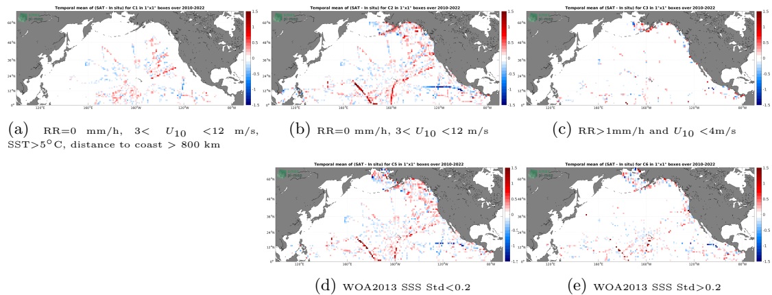
Figure 12: Temporal mean gridded over spatial boxes of size 1^\circ \times 1^\circ of \Delta SSS (SMOS SSS L3 v8 - 9 Days (CATDS-CECOS-LOCEAN) - TSG (SAMOS)) for 5 different subdatasets corresponding to:RR=0 mm/h, 3 < U_{10} < 12 m/s, SST >5^\circ C, distance to coast > 800 km (a), RR=0 mm/h, 3 < U_{10} < 12 m/s (b), RR >1 mm/h and U_{10} < 4 m/s (c), WOA2013 SSS Std <0.2 (d), WOA2013 SSS Std >0.2 (e).
