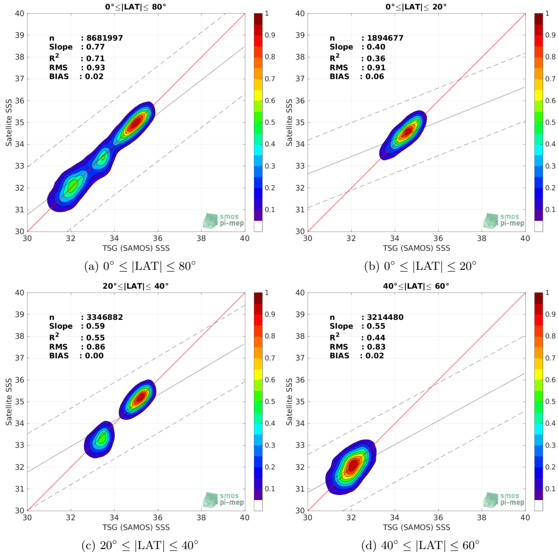
Figure 9: Contour maps of the concentration of SMOS SSS L3 v8 - 9 Days (CATDS-CECOS-LOCEAN) SSS (y-axis) versus TSG (SAMOS) SSS (x-axis) at match-up pairs for different latitude bands. For each plot, the red line shows x=y . The black thin and dashed lines indicate a linear fit through the data cloud and the \pm 95\% confidence levels, respectively. The number match-up pairs n , the slope and R^2 coefficient of the linear fit, the root mean square (RMS) and the mean bias between satellite and in situ data are indicated for each latitude band in each plots.
