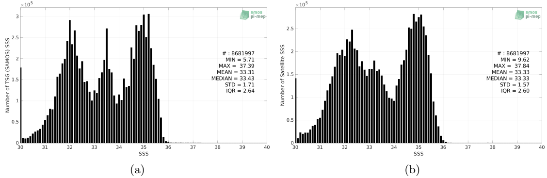
Figure 2: Histograms of SSS from TSG (SAMOS) (a) and SMOS SSS L3 v8 - 9 Days (CATDS-CECOS-LOCEAN) (b) considering all match-up pairs per bins of 0.1 over the North Pacific Ocean Pi-MEP region and for the full satellite product period.
