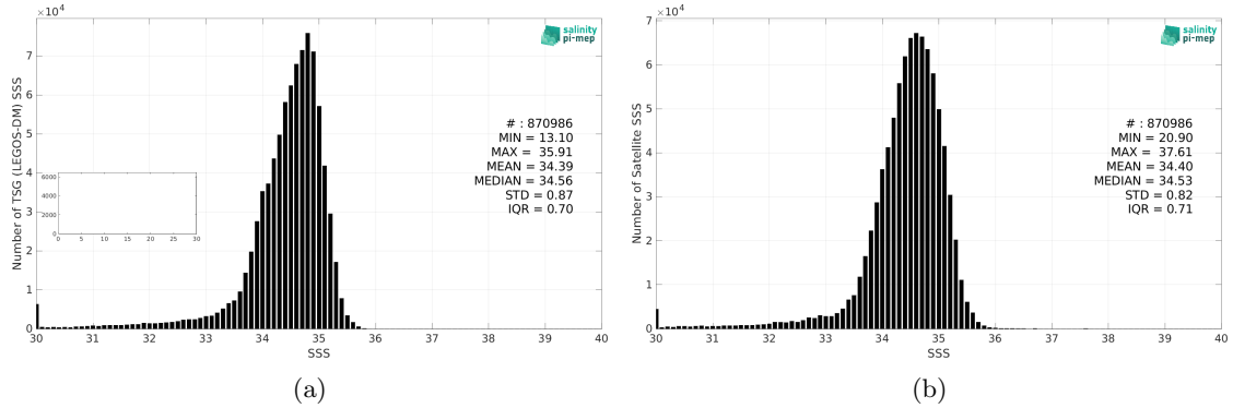
Figure 2: Histograms of SSS from TSG (LEGOS-DM) (a) and SMOS SSS L3 v8 - 9 Days (CATDS-CEC-LOCEAN) (b) considering all match-up pairs per bins of 0.1 over the North Pacific Ocean Pi-MEP region and for the full satellite product period.
