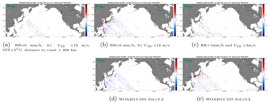
Figure 12: Temporal mean gridded over spatial boxes of size 1^\circ \times 1^\circ of \Delta SSS (SMOS SSS L3 v8 - 9 Days (CATDS-CEC-LOCEAN) - TSG (LEGOS-DM)) for 5 different subdatasets corresponding to:RR=0 mm/h, 3 < U_{10} < 12 m/s, SST >5^\circ C, distance to coast > 800 km (a), RR=0 mm/h, 3 < U_{10} < 12 m/s (b), RR >1 mm/h and U_{10} < 4 m/s (c), WOA2013 SSS Std <0.2 (d), WOA2013 SSS Std >0.2 (e).
