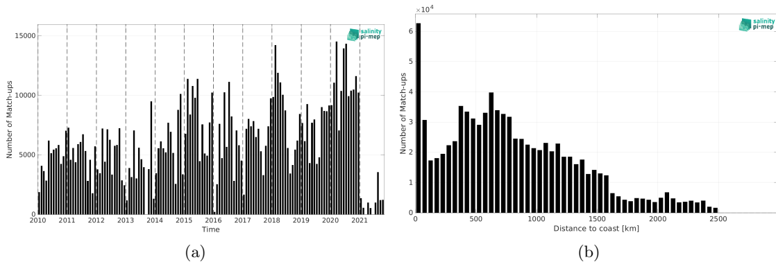
Figure 1: Number of match-ups between TSG (LEGOS-DM) and SMOS SSS L3 v8 - 9 Days (CATDS-CEC-LOCEAN) SSS as a function of time (a) and as function of the distance to coast (b) over the North Pacific Ocean Pi-MEP region and for the full satellite product period.
