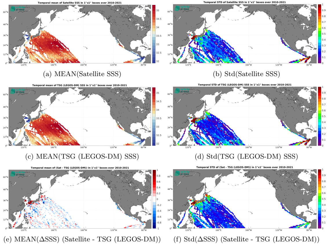
Figure 6: Temporal mean (left) and Std (right) of SSS from SMOS SSS L3 v8 - 9 Days (CATDS-CEC-LOCEAN) (top), TSG (LEGOS-DM) (middle), and of \Delta\text{SSS} (Satellite - TSG (LEGOS-DM)). Only match-up pairs are used to generate these maps.
