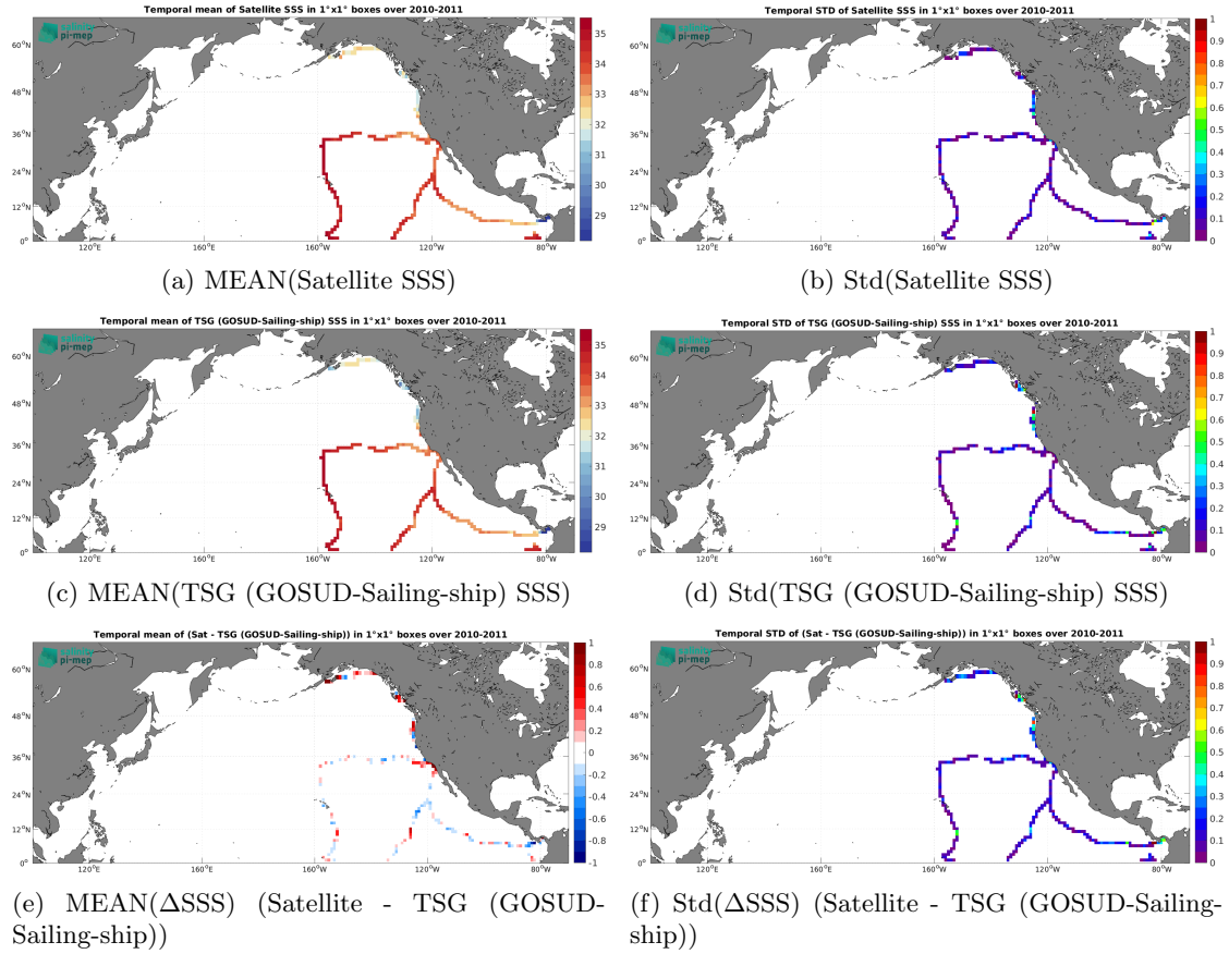
Figure 6: Temporal mean (left) and Std (right) of SSS from SMOS SSS L3 v8 - 9 Days (CATDS-CEC-LOCEAN) (top), TSG (GOSUD-Sailing-ship) (middle), and of \Delta SSS (Satellite - TSG (GOSUD-Sailing-ship)). Only match-up pairs are used to generate these maps.
