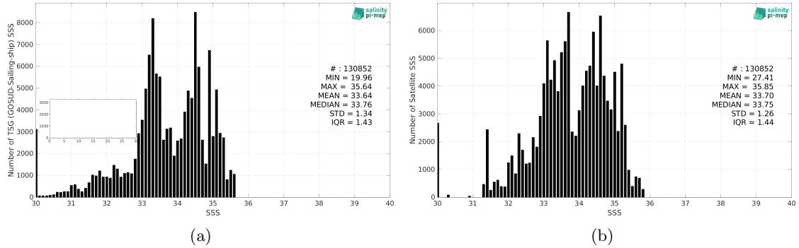
Figure 2: Histograms of SSS from TSG (GOSUD-Sailing-ship) (a) and SMOS SSS L3 v8 - 9 Days (CATDS-CEC-LOCEAN) (b) considering all match-up pairs per bins of 0.1 over the North Pacific Ocean Pi-MEP region and for the full satellite product period.
