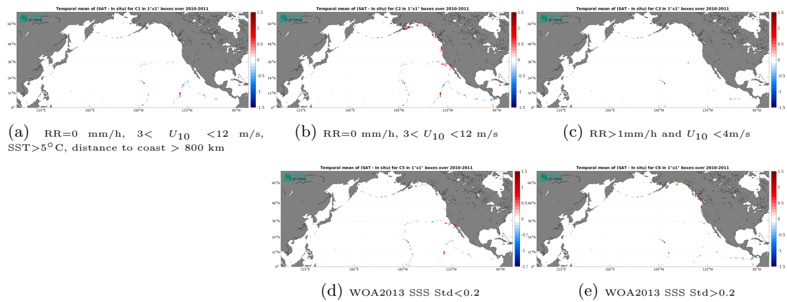
Figure 12: Temporal mean gridded over spatial boxes of size 1^\circ \times 1^\circ of \Delta SSS (SMOS SSS L3 v8 - 9 Days (CATDS-CEC-LOCEAN) - TSG (GOSUD-Sailing-ship)) for 5 different subdatasets corresponding to: RR=0 mm/h, 3 < U_{10} < 12 m/s, SST > 5°C, distance to coast > 800 km (a), RR=0 mm/h, 3 < U_{10} < 12 m/s (b), RR > 1mm/h and U_{10} < 4 m/s (c), WOA2013 SSS Std < 0.2 (d), WOA2013 SSS Std > 0.2 (e).
