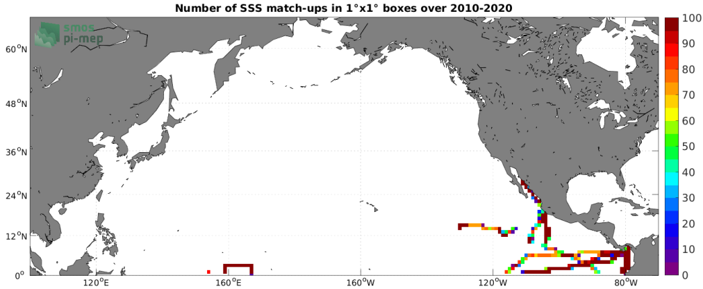
Figure 4: Number of SSS match-ups between TSG (GOSUD-Research-vessel) SSS and the SMOS SSS L3 v8 - 9 Days (CATDS-CECOS-LOCEAN) SSS product for the North Pacific Ocean Pi-MEP region over 1^\circ \times 1^\circ boxes and for the full satellite product period.
