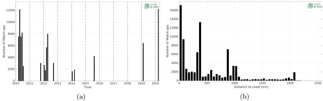
Figure 1: Number of match-ups between TSG (GOSUD-Research-vessel) and SMOS SSS L3 v8 - 9 Days (CATDS-CECOS-LOCEAN) SSS as a function of time (a) and as function of the distance to coast (b) over the North Pacific Ocean Pi-MEP region and for the full satellite product period.
