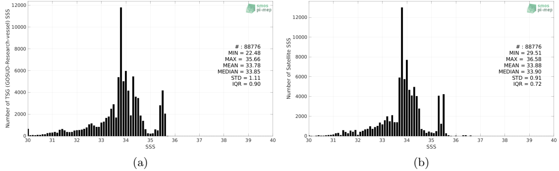
Figure 2: Histograms of SSS from TSG (GOSUD-Research-vessel) (a) and SMOS SSS L3 v8 - 9 Days (CATDS-CECOS-LOCEAN) (b) considering all match-up pairs per bins of 0.1 over the North Pacific Ocean Pi-MEP region and for the full satellite product period.
