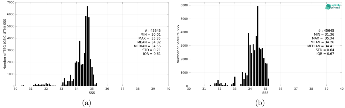
Figure 2: Histograms of SSS from TSG (CSIC-UTM) (a) and SMOS SSS L3 v8 - 9 Days (CATDS-CEC-LOCEAN) (b) considering all match-up pairs per bins of 0.1 over the North Pacific Ocean Pi-MEP region and for the full satellite product period.
