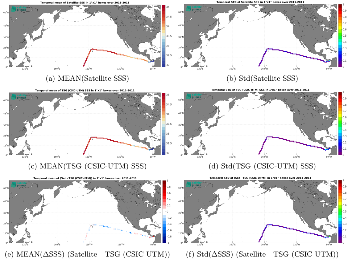
Figure 6: Temporal mean (left) and Std (right) of SSS from SMOS SSS L3 v8 - 9 Days (CATDS-CEC-LOCEAN) (top), TSG (CSIC-UTM) (middle), and of \Delta\text{SSS} (Satellite - TSG (CSIC-UTM)). Only match-up pairs are used to generate these maps.
