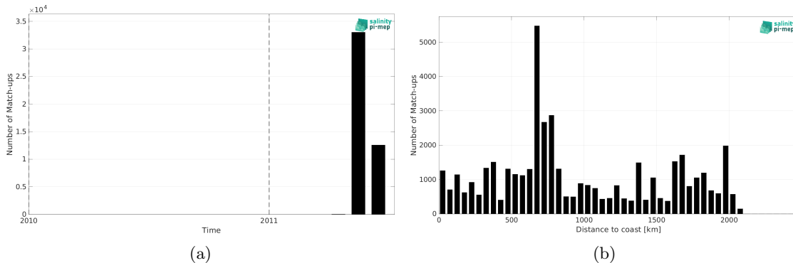
Figure 1: Number of match-ups between TSG (CSIC-UTM) and SMOS SSS L3 v8 - 9 Days (CATDS-CEC-LOCEAN) SSS as a function of time (a) and as function of the distance to coast (b) over the North Pacific Ocean Pi-MEP region and for the full satellite product period.
