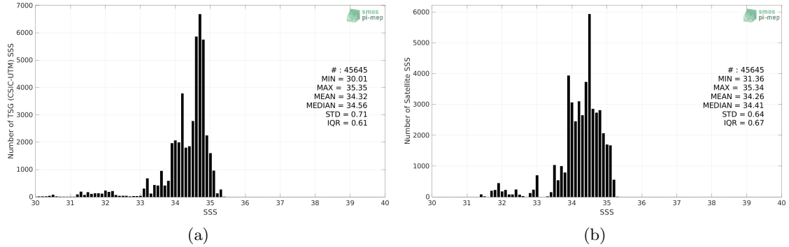
Figure 2: Histograms of SSS from TSG (CSIC-UTM) (a) and SMOS SSS L3 v8 - 9 Days (CATDS-CECOS-LOCEAN) (b) considering all match-up pairs per bins of 0.1 over the North Pacific Ocean Pi-MEP region and for the full satellite product period.
