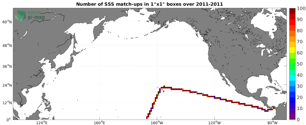
Figure 4: Number of SSS match-ups between TSG (CSIC-UTM) SSS and the SMOS SSS L3 v8 - 9 Days (CATDS-CECOS-LOCEAN) SSS product for the North Pacific Ocean Pi-MEP region over 1^\circ \times 1^\circ boxes and for the full satellite product period.
