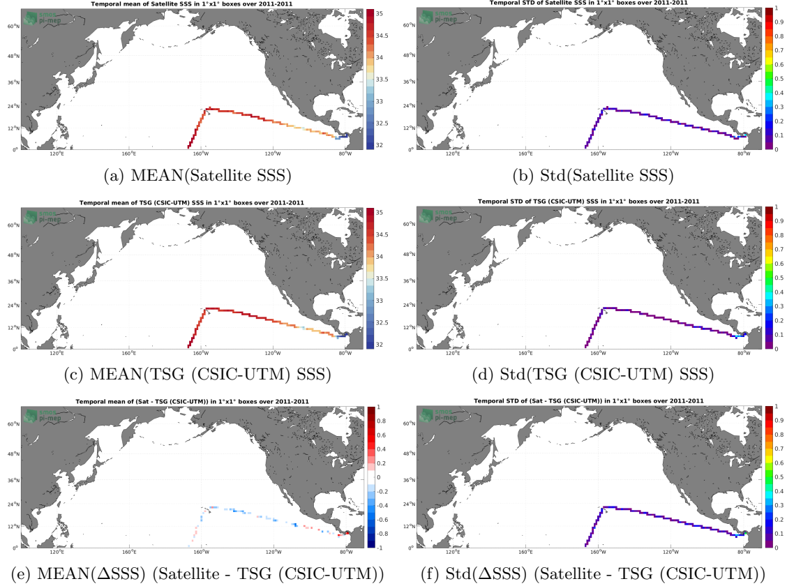
Figure 6: Temporal mean (left) and Std (right) of SSS from SMOS SSS L3 v8 - 9 Days (CATDS-CECOS-LOCEAN) (top), TSG (CSIC-UTM) (middle), and of \Delta\text{SSS} (Satellite - TSG (CSIC-UTM)). Only match-up pairs are used to generate these maps.
