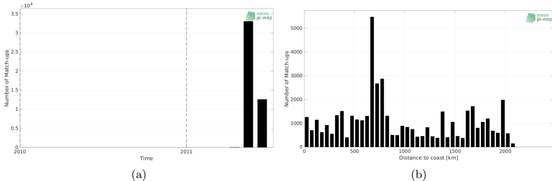
Figure 1: Number of match-ups between TSG (CSIC-UTM) and SMOS SSS L3 v8 - 9 Days (CATDS-CECOS-LOCEAN) SSS as a function of time (a) and as function of the distance to coast (b) over the North Pacific Ocean Pi-MEP region and for the full satellite product period.
