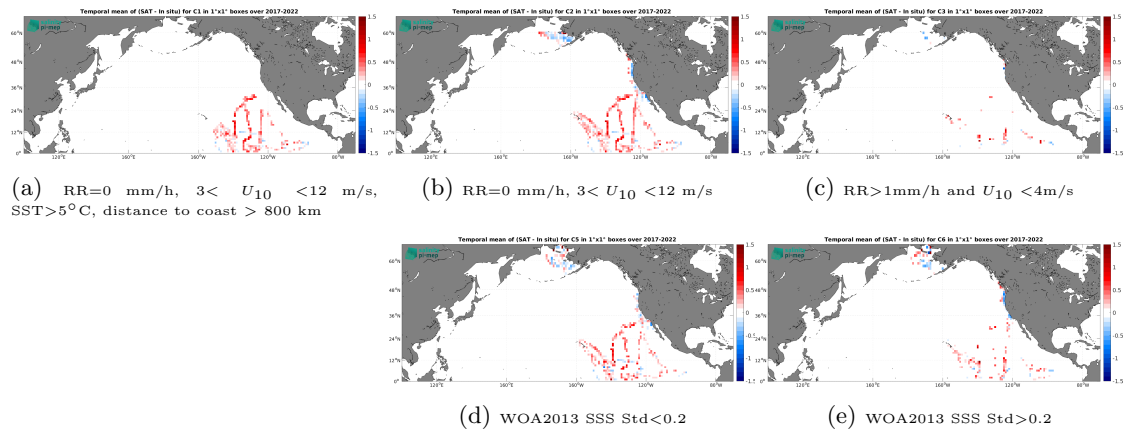
Figure 12: Temporal mean gridded over spatial boxes of size 1^\circ \times 1^\circ of \Delta SSS (SMOS SSS L3 v8 - 9 Days (CATDS-CEC-LOCEAN) - Sailldrone) for 5 different subdatasets corresponding to:RR=0 mm/h, 3 < U_{10} < 12 m/s, SST >5^\circ C, distance to coast > 800 km (a), RR=0 mm/h, 3 < U_{10} < 12 m/s (b), RR >1 mm/h and U_{10} < 4 m/s (c), WOA2013 SSS Std <0.2 (d), WOA2013 SSS Std >0.2 (e).
