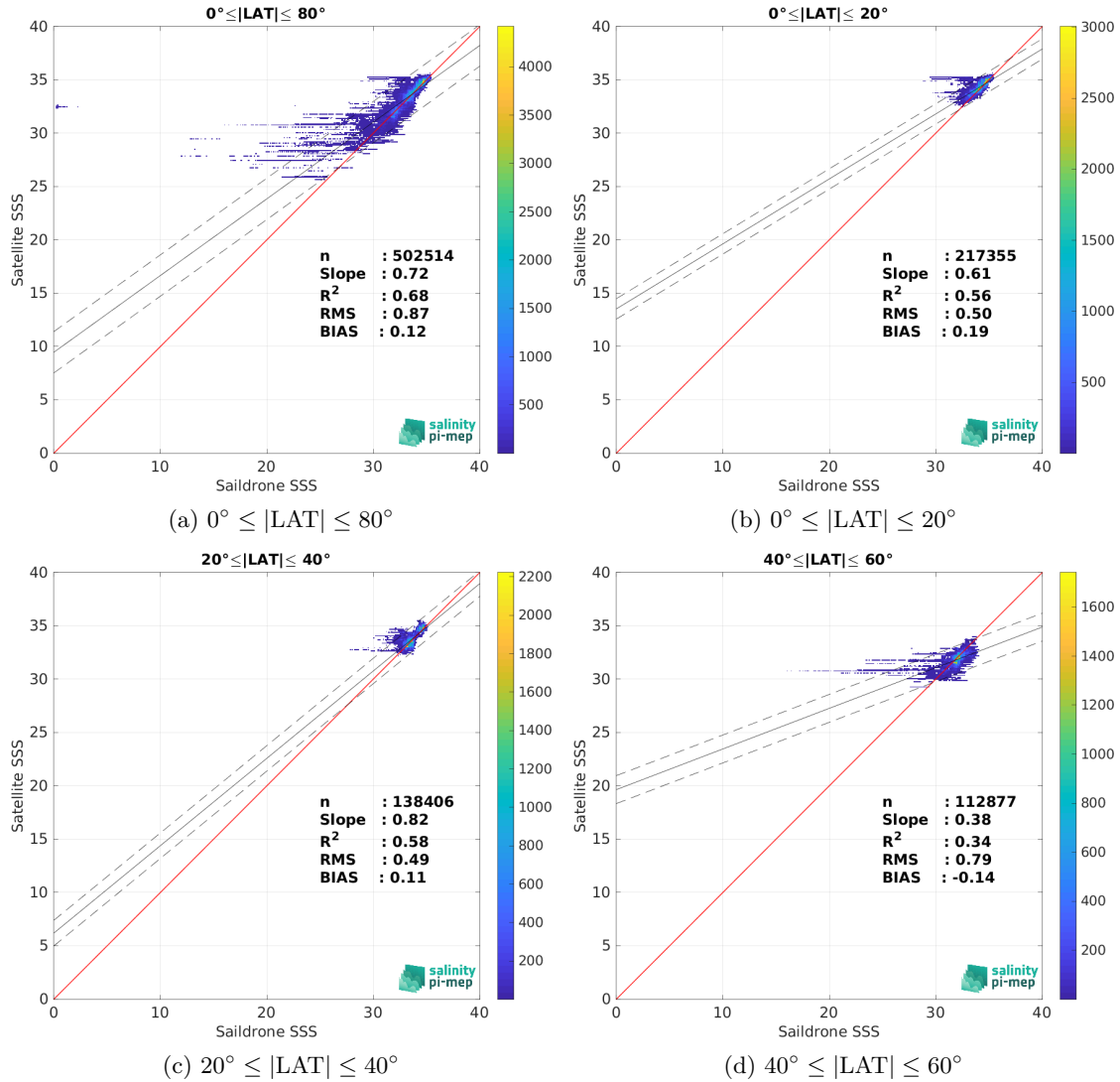
Figure 9: Contour maps of the concentration of SMOS SSS L3 v8 - 9 Days (CATDS-CEC-LOCEAN) SSS (y-axis) versus Sairdrone SSS (x-axis) at match-up pairs for different latitude bands. For each plot, the red line shows x=y . The black thin and dashed lines indicate a linear fit through the data cloud and the \pm 95\% confidence levels, respectively. The number match-up pairs n , the slope and R^2 coefficient of the linear fit, the root mean square (RMS) and the mean bias between satellite and in situ data are indicated for each latitude band in each plots.
