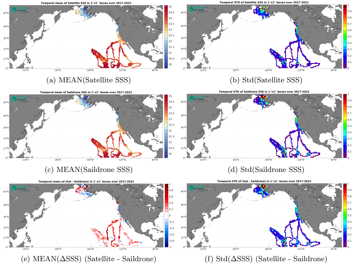
Figure 6: Temporal mean (left) and Std (right) of SSS from SMOS SSS L3 v8 - 9 Days (CATDS-CEC-LOCEAN) (top), Sairdrone (middle), and of \Delta\text{SSS} (Satellite - Sairdrone). Only match-up pairs are used to generate these maps.
