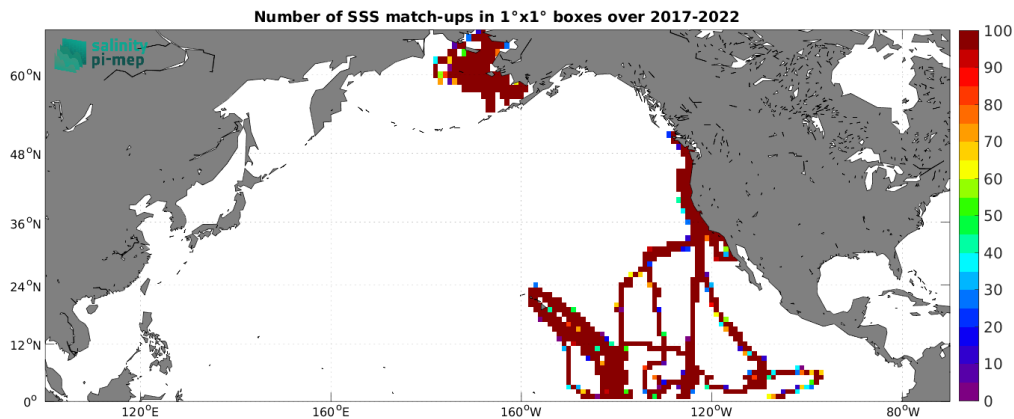
Figure 4: Number of SSS match-ups between Saildrone SSS and the SMOS SSS L3 v8 - 9 Days (CATDS-CEC-LOCEAN) SSS product for the North Pacific Ocean Pi-MEP region over 1^\circ \times 1^\circ boxes and for the full satellite product period.
