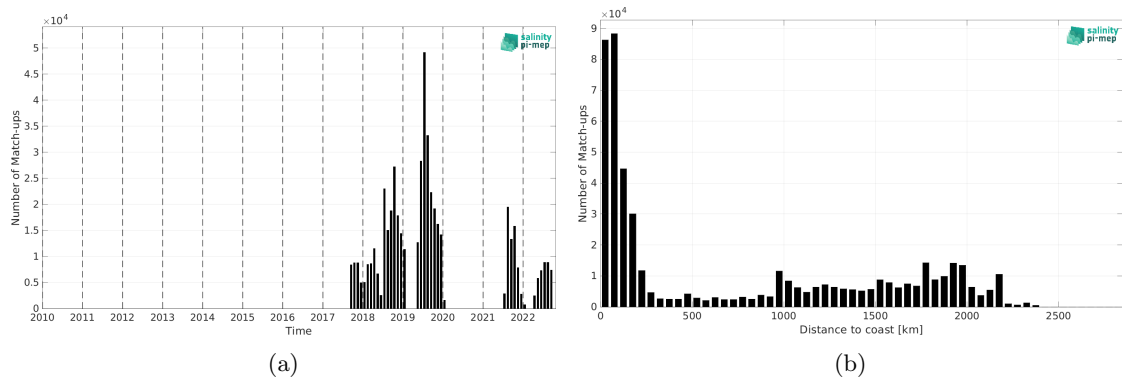
Figure 1: Number of match-ups between Saildrone and SMOS SSS L3 v8 - 9 Days (CATDS-CEC-LOCEAN) SSS as a function of time (a) and as function of the distance to coast (b) over the North Pacific Ocean Pi-MEP region and for the full satellite product period.
