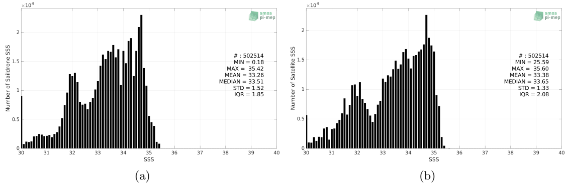
Figure 2: Histograms of SSS from Saildrone (a) and SMOS SSS L3 v8 - 9 Days (CATDS-CECOS-LOCEAN) (b) considering all match-up pairs per bins of 0.1 over the North Pacific Ocean Pi-MEP region and for the full satellite product period.
