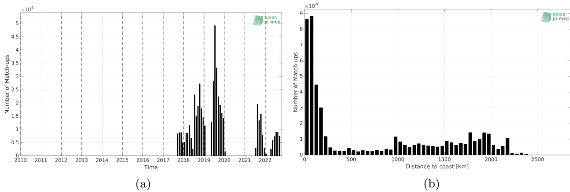
Figure 1: Number of match-ups between Saildrone and SMOS SSS L3 v8 - 9 Days (CATDS-CECOS-LOCEAN) SSS as a function of time (a) and as function of the distance to coast (b) over the North Pacific Ocean Pi-MEP region and for the full satellite product period.
