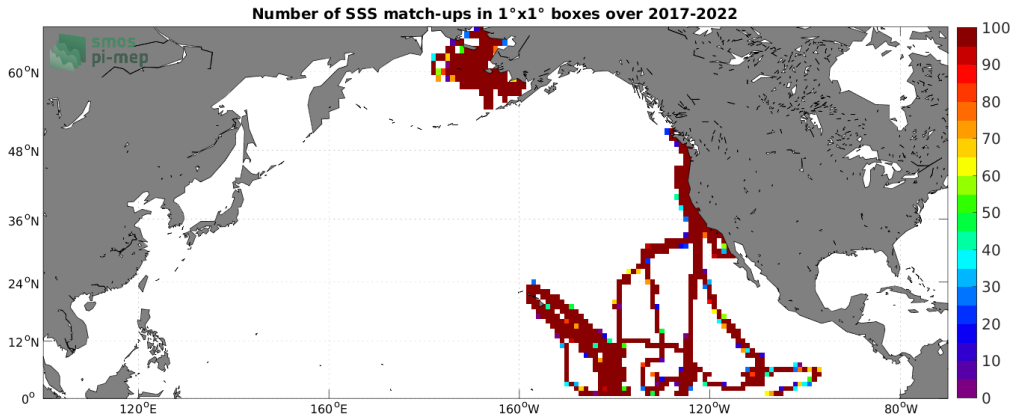
Figure 4: Number of SSS match-ups between Saildrone SSS and the SMOS SSS L3 v8 - 9 Days (CATDS-CECOS-LOCEAN) SSS product for the North Pacific Ocean Pi-MEP region over 1^\circ \times 1^\circ boxes and for the full satellite product period.
