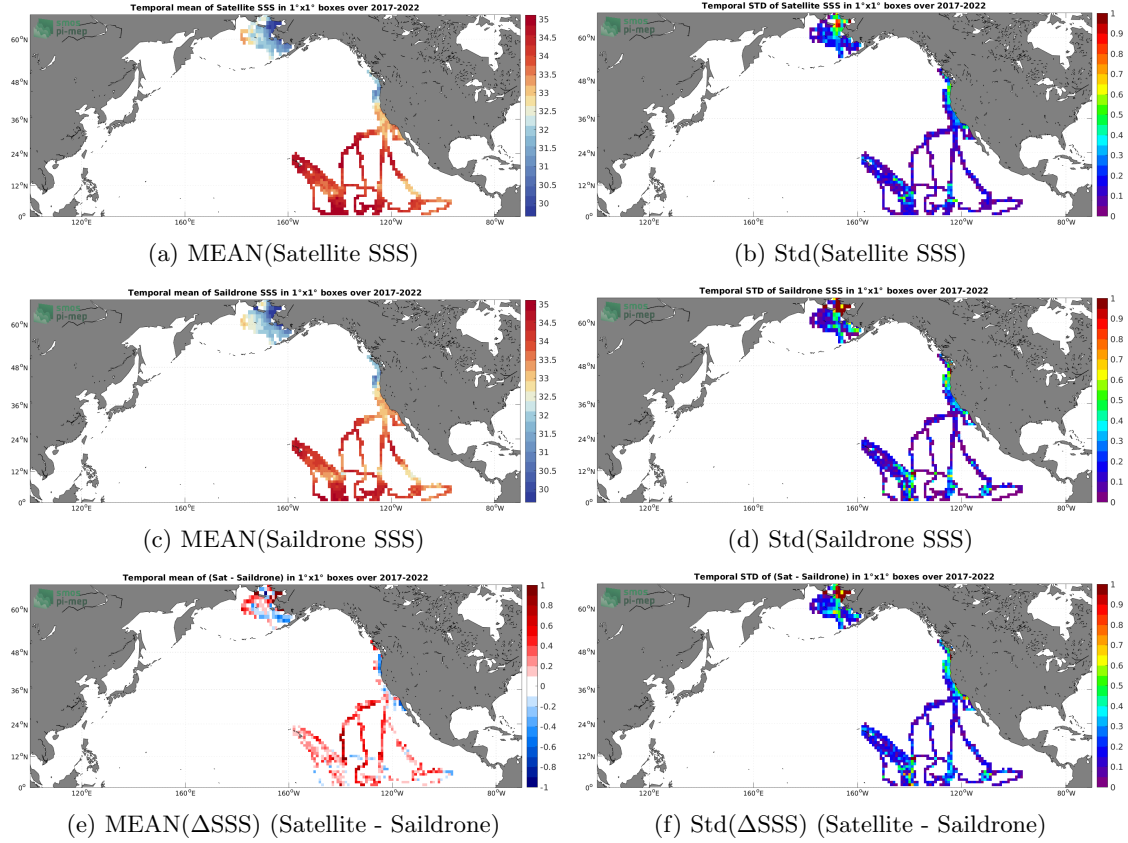
Figure 6: Temporal mean (left) and Std (right) of SSS from SMOS SSS L3 v8 - 9 Days (CATDS-CECOS-LOCEAN) (top), Saildrone (middle), and of \Delta\text{SSS} (Satellite - Saildrone). Only match-up pairs are used to generate these maps.
