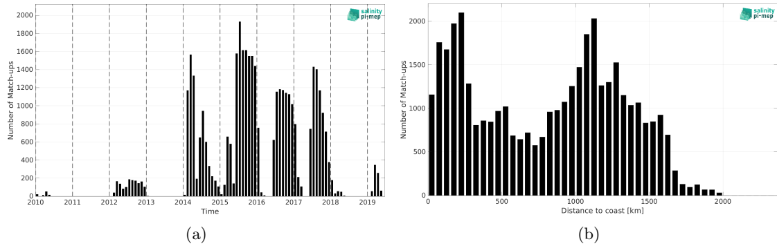
Figure 1: Number of match-ups between Marine mammals and SMOS SSS L3 v8 - 9 Days (CATDS-CEC-LOCEAN) SSS as a function of time (a) and as function of the distance to coast (b) over the North Pacific Ocean Pi-MEP region and for the full satellite product period.
