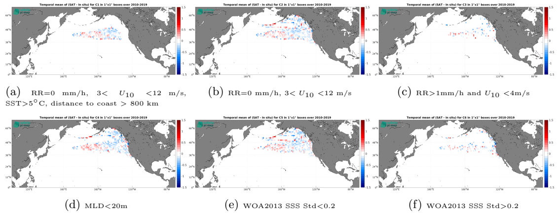
Figure 12: Temporal mean gridded over spatial boxes of size 1^{\circ}\times 1^{\circ} of \Delta\text{SSS} (SMOS SSS L3 v8 - 9 Days (CATDS-CEC-LOCEAN) - Marine mammals) for 6 different subdatasets corresponding to:RR=0 mm/h, 3 < U_{10} < 12 m/s, SST > 5^{\circ}\text{C} , distance to coast > 800 km (a), RR=0 mm/h, 3 < U_{10} < 12 m/s (b), RR > 1 mm/h and U_{10} < 4 m/s (c),MLD < 20\text{m} (d),WOA2013 SSS Std < 0.2 (e),WOA2013 SSS Std > 0.2 (f).
