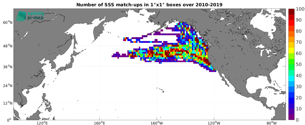
Figure 4: Number of SSS match-ups between Marine mammals SSS and the SMOS SSS L3 v8 - 9 Days (CATDS-CEC-LOCEAN) SSS product for the North Pacific Ocean Pi-MEP region over 1^\circ \times 1^\circ boxes and for the full satellite product period.
