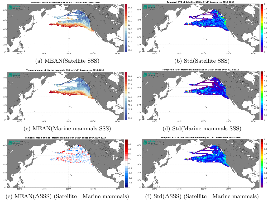
Figure 6: Temporal mean (left) and Std (right) of SSS from SMOS SSS L3 v8 - 9 Days (CATDS-CEC-LOCEAN) (top), Marine mammals (middle), and of \Delta SSS (Satellite - Marine mammals). Only match-up pairs are used to generate these maps.
